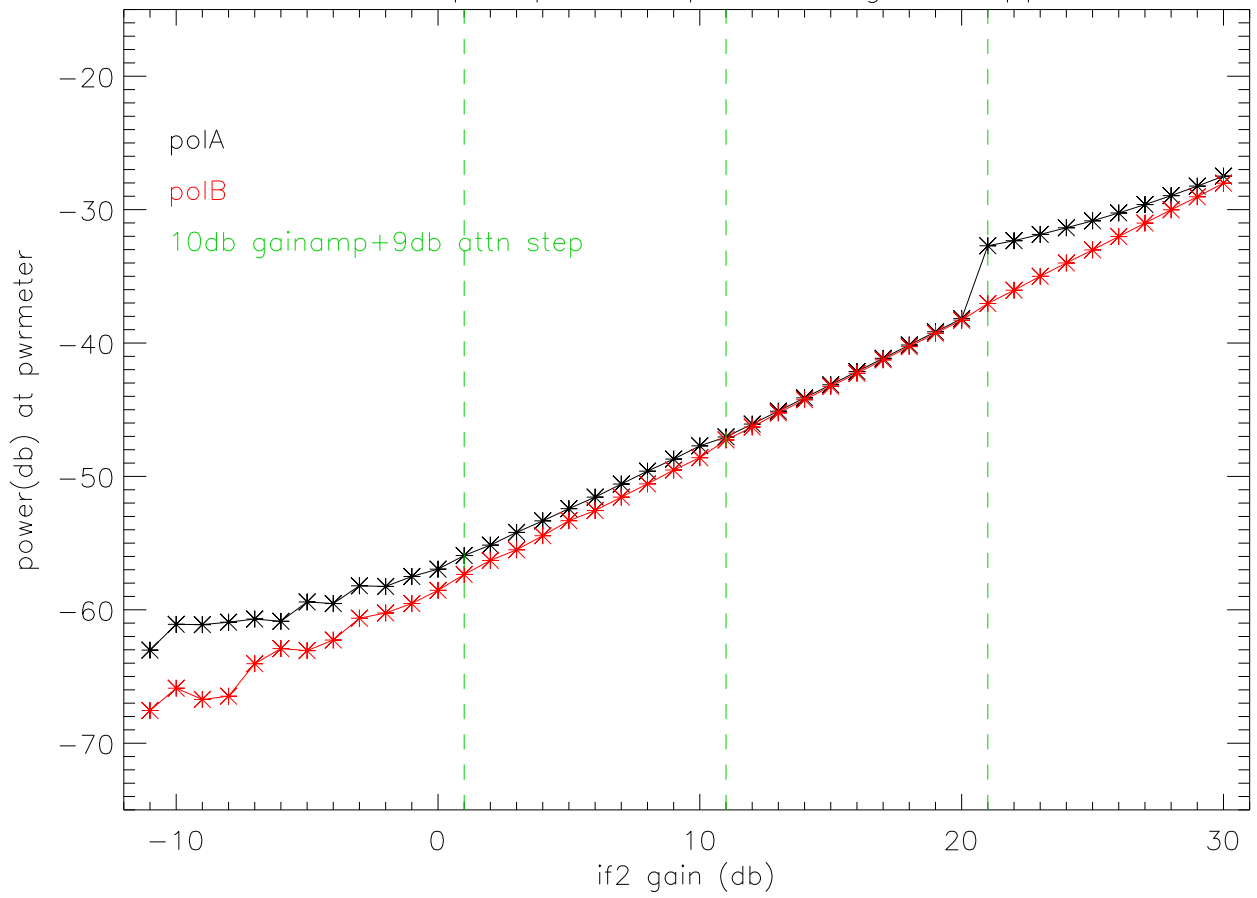
27nov06 polA-polB if2 power dif as gain stepped
