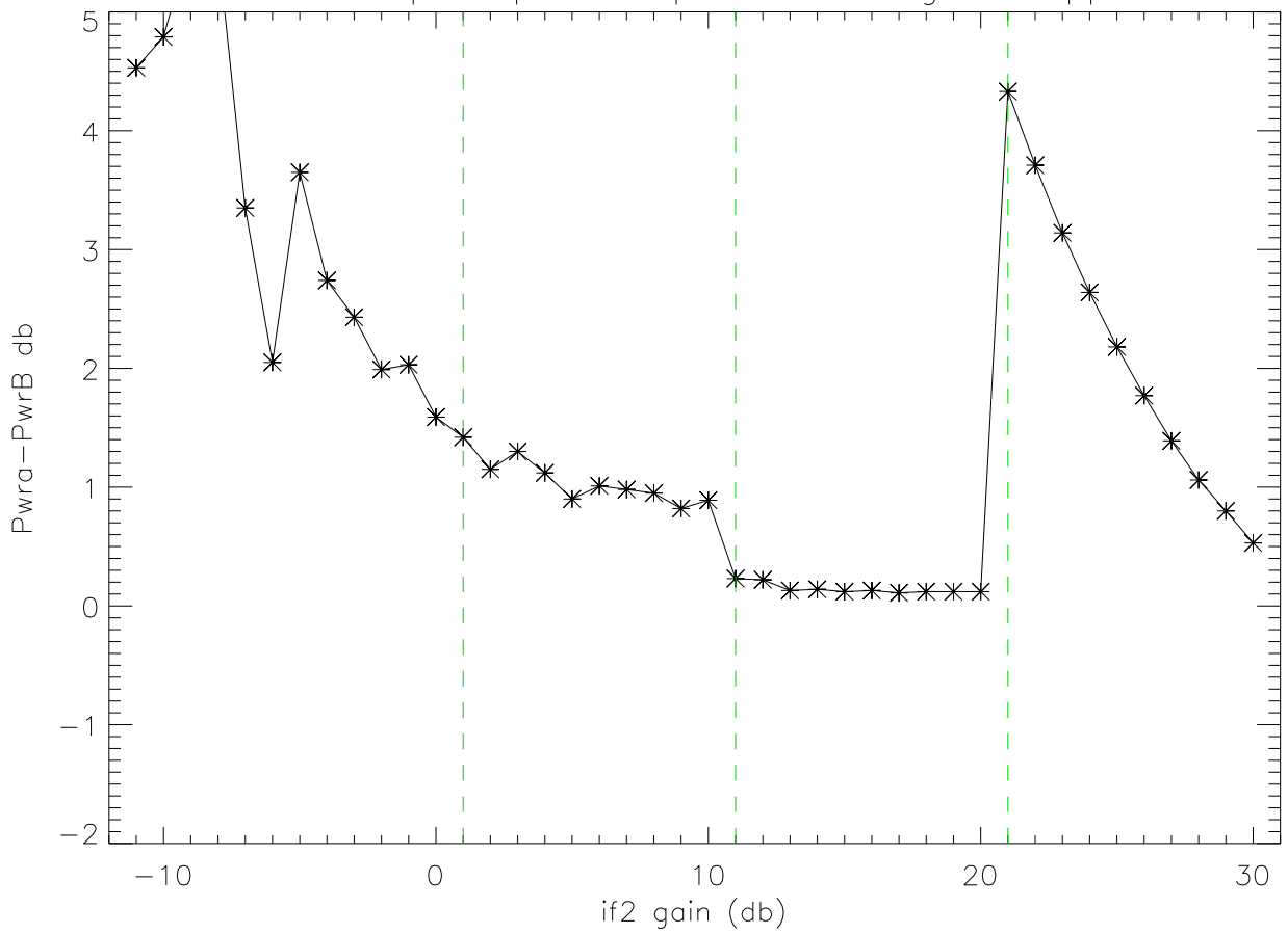
27nov06 polA-polB if2 power dif as gain stepped
