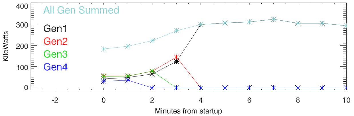
Power output (by gen)
