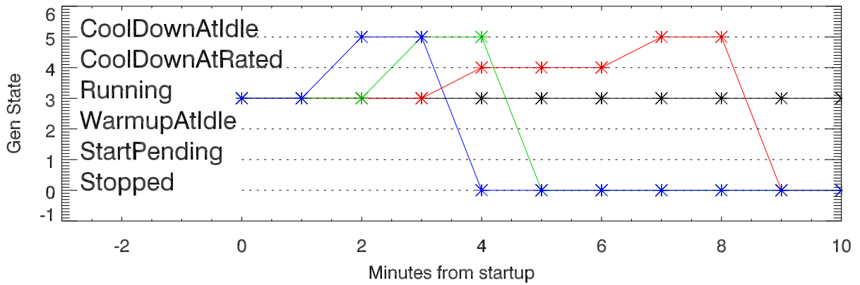
01dec13 (Sun 17:40:01) generator startup (load=site). Gen State.
