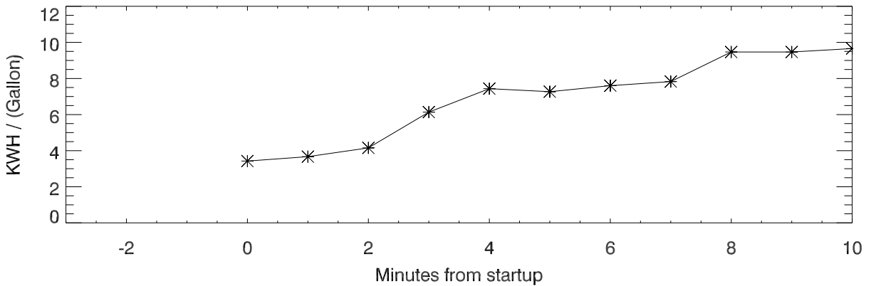
Efficiency: (KiloWatt hours output) per (gallon) (all gen summed)
