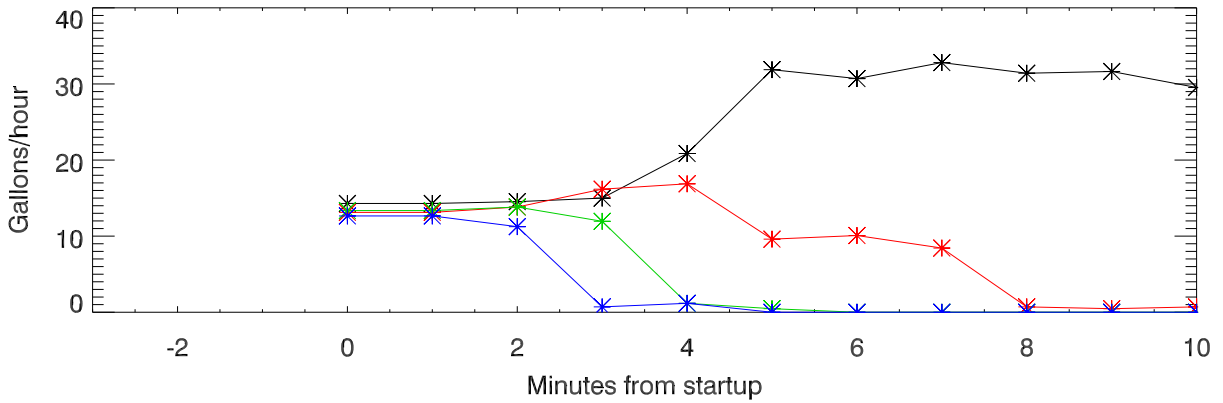
Fuel usage (by generator)
