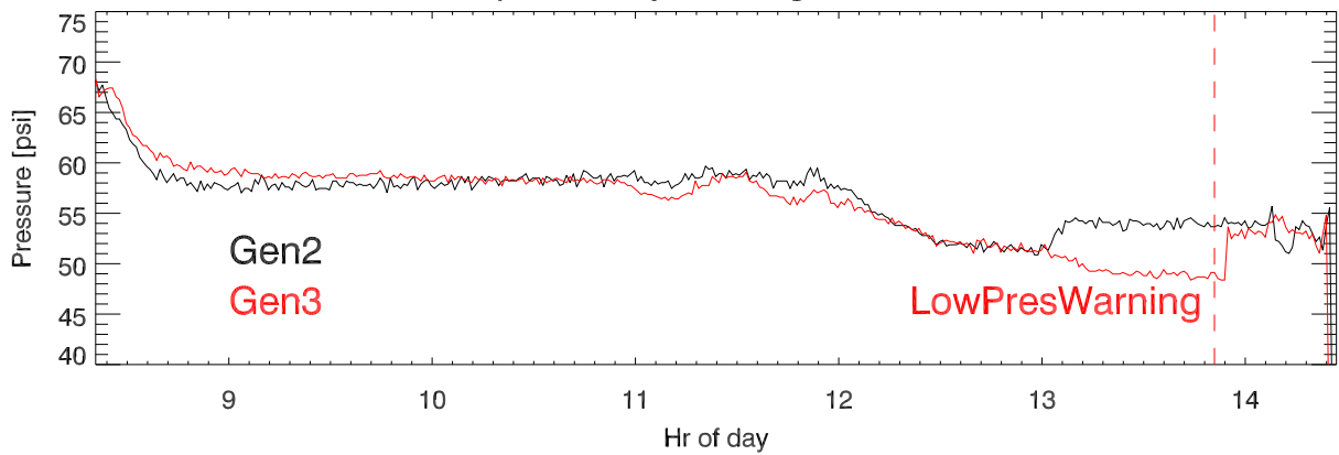
oil pressure by montor/generator set
