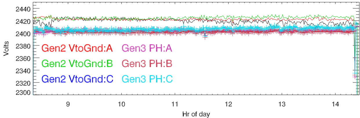
phase to ground voltage for each phase
