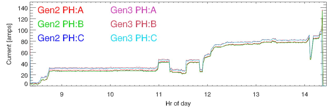
generator Current for each phase
