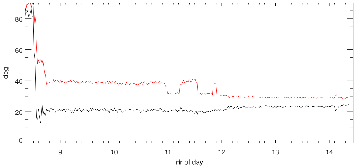
phase angle between current and voltage
