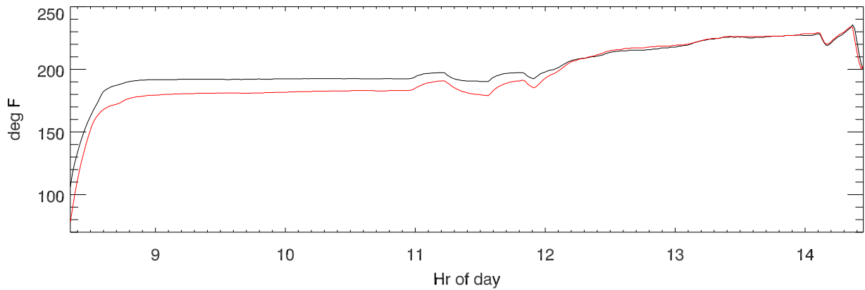
oil Temperature by motor/generator set
