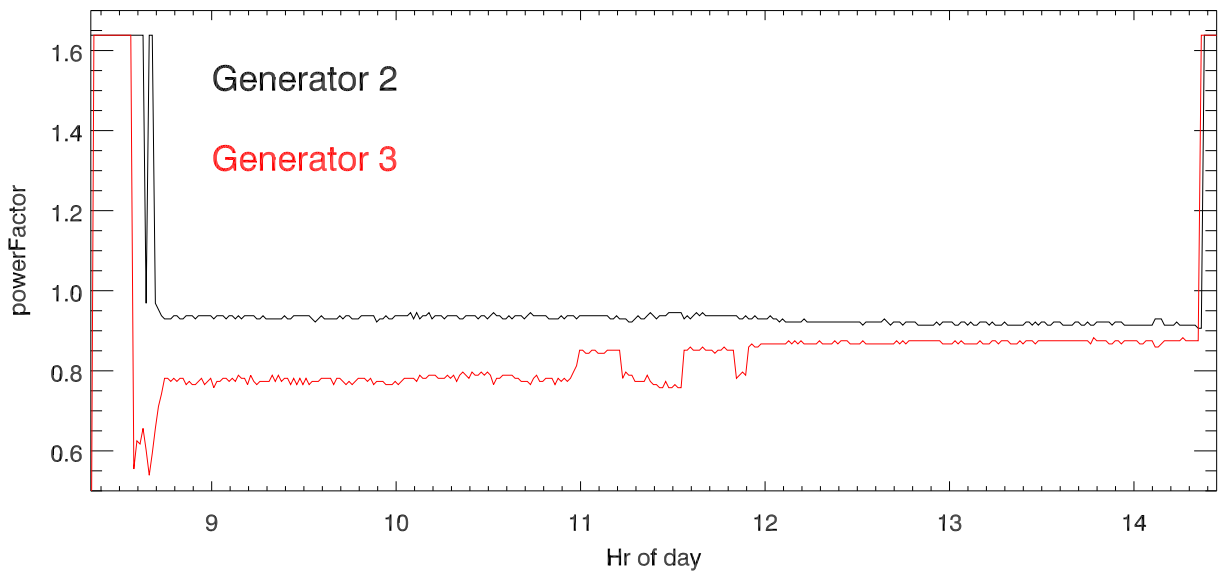
Power factor
