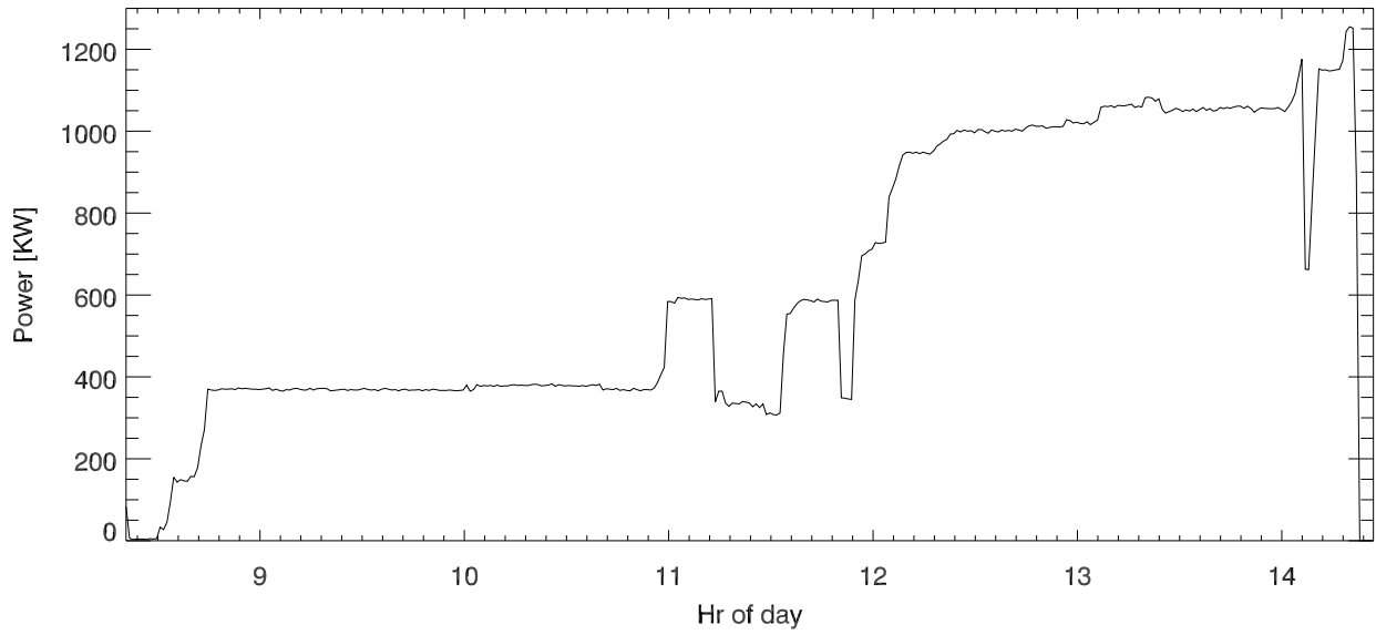
180309 Generator status during hfTest. Total output power
