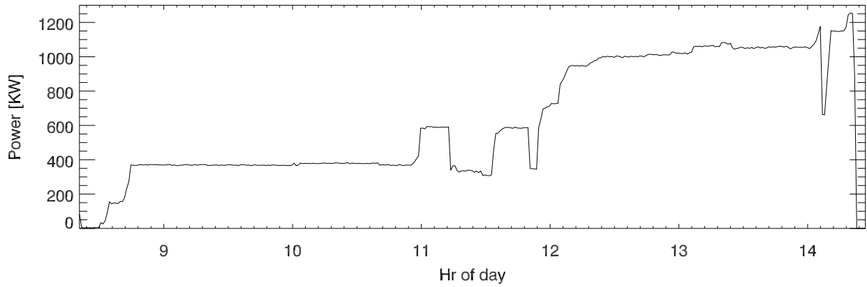
180309 Generator status cont.. Total output power
