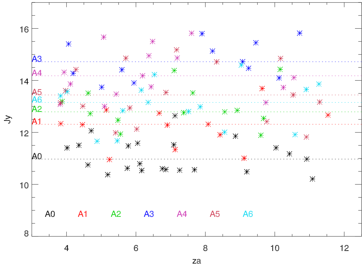
AO40 SEFD vs za from dipole 1 crosses
