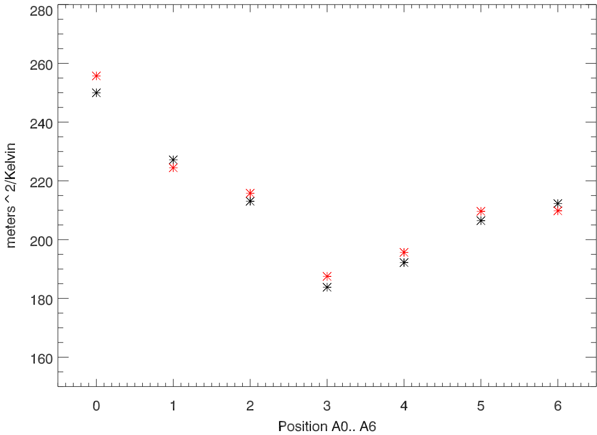
Average Ae/Tsys for positions A0..A6
