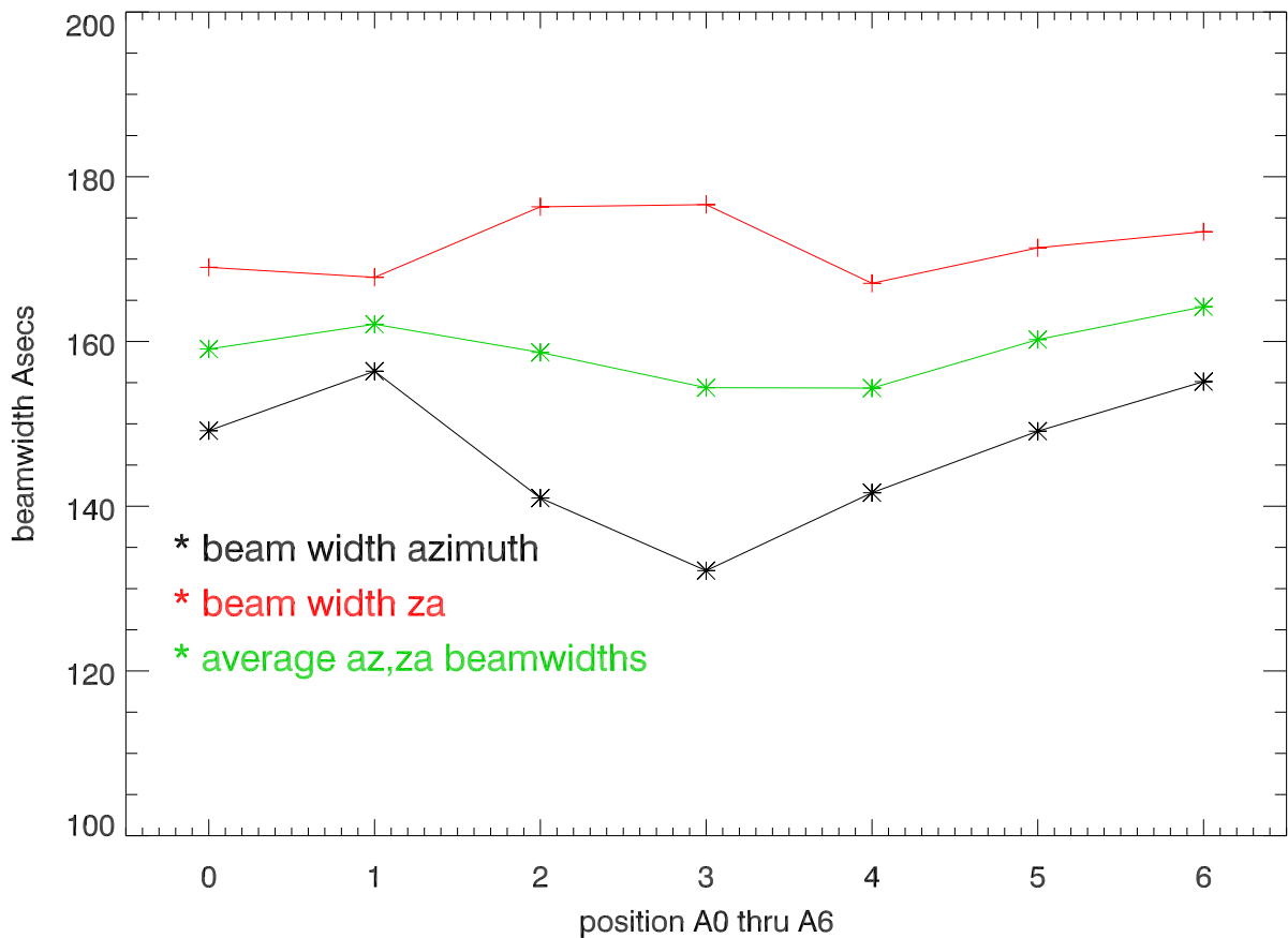
AO40 average FWHM beamWidths for positions A0..A6
