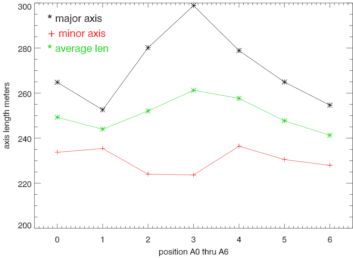
AO40 major, minor axis lengths from beamwidths
