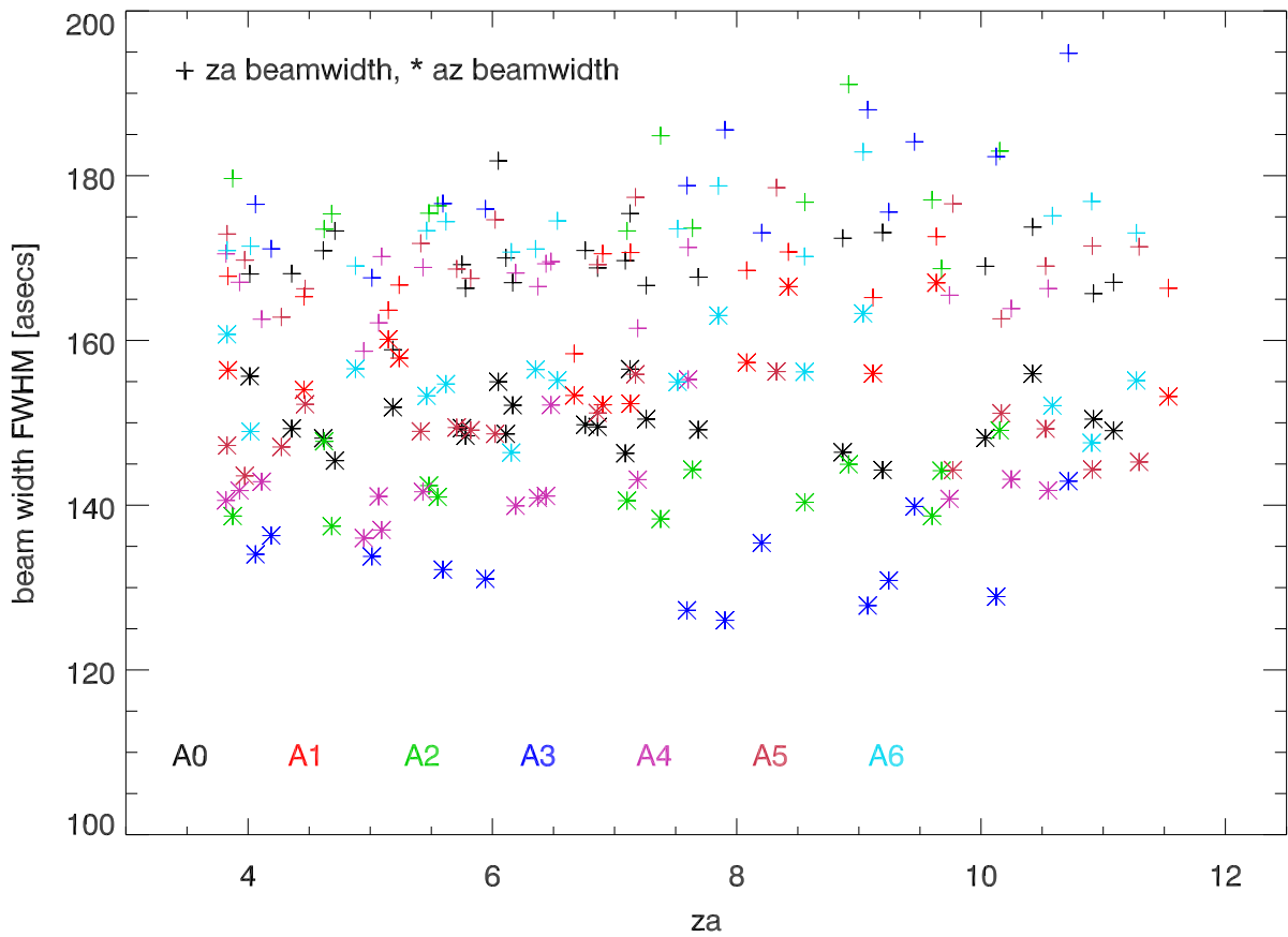
AO40 Beamwidths vs za from dipole_1 crosses (each cross plotted)
