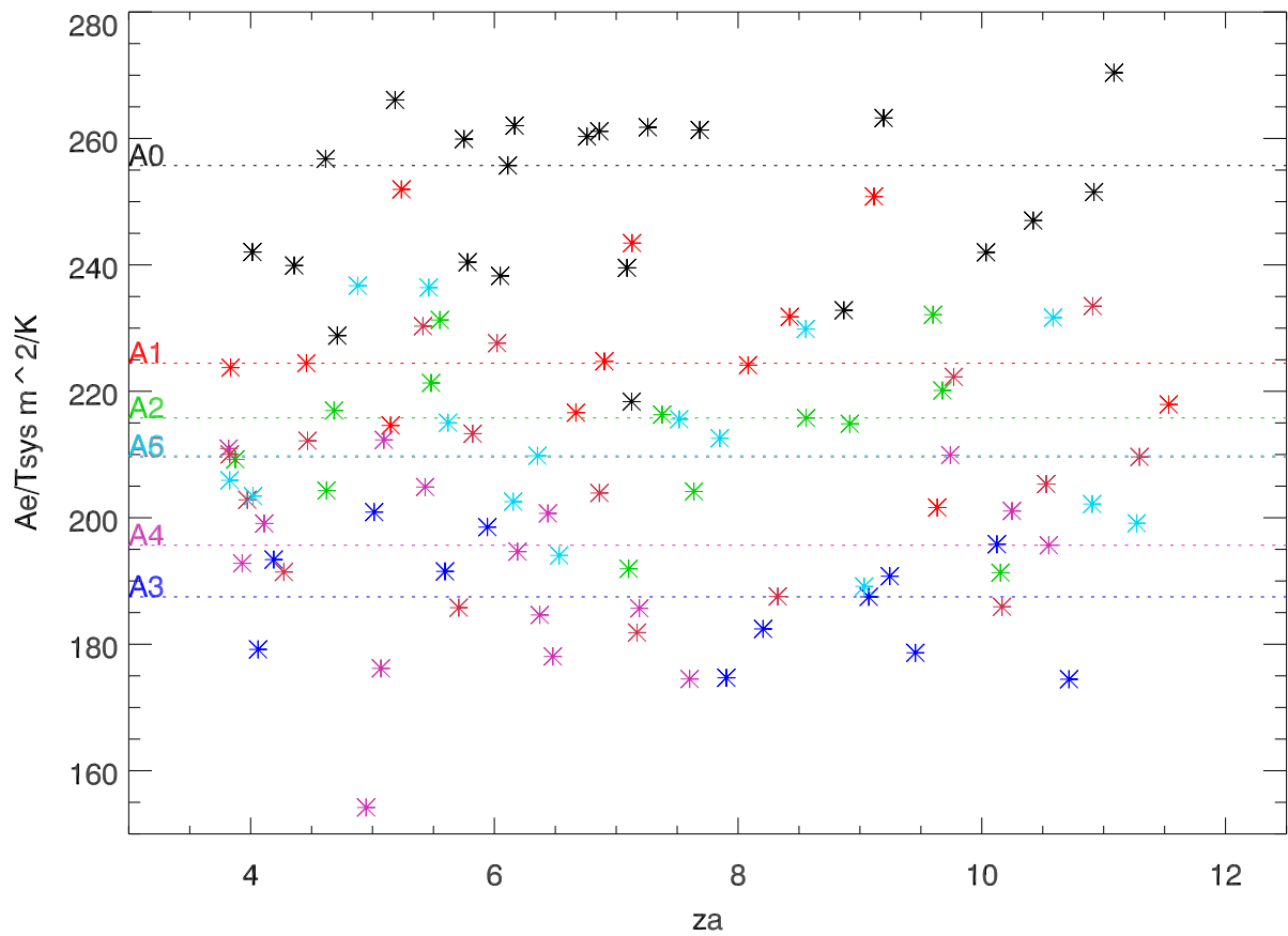
AO40 Sensitivity A_e/T_{sys} vs za from dipole 1 crosses
