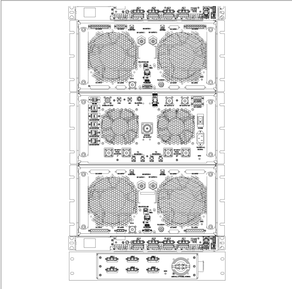
SYSTEM OUTLINE (Rear View)
