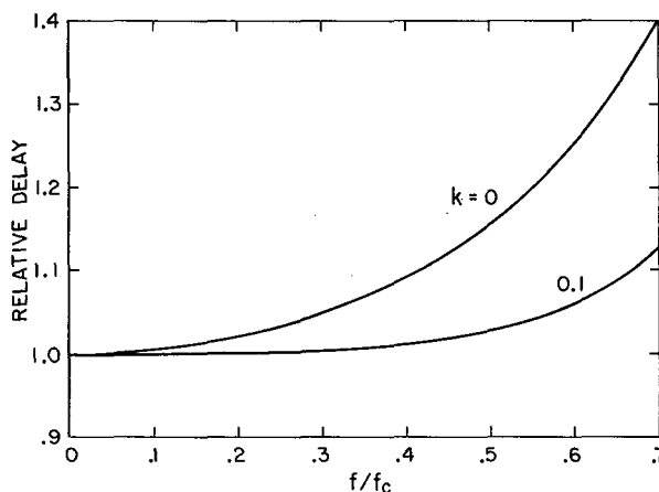
Figure P-2. Delay versus frequency for k = 0, 0.1 .
