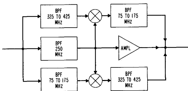
Figure 10-9. Channel interchanger.
