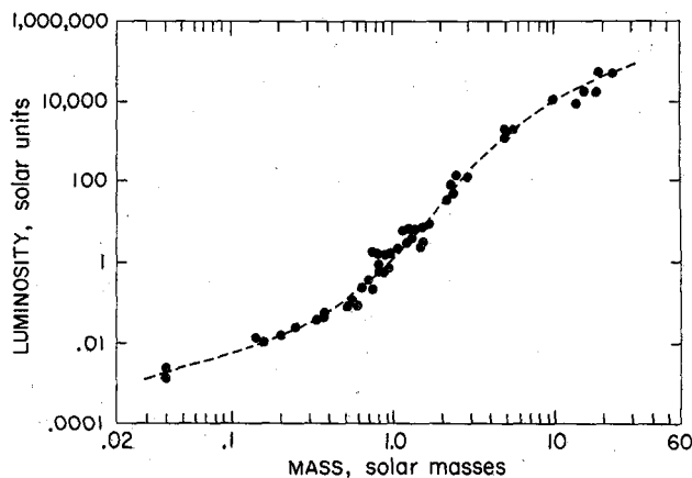
Figure 2-4. The mass-luminosity relation.
