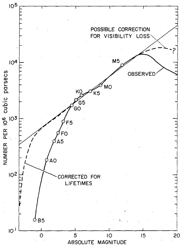
Figure 2-5. The luminosity function.
