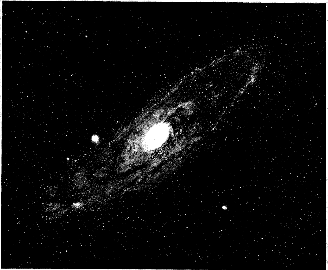
Figure 2-1. M31, the great galaxy in Andromeda. (Photo courtesy Lick Observatory)
