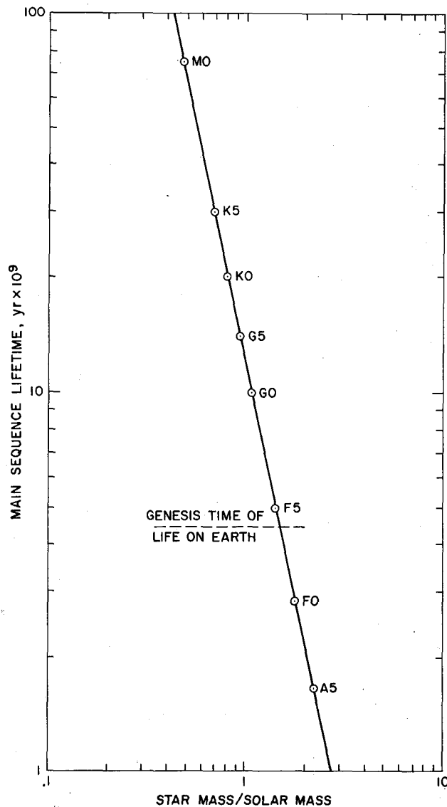
Figure 2-7. Stellar lifetimes versus mass.
