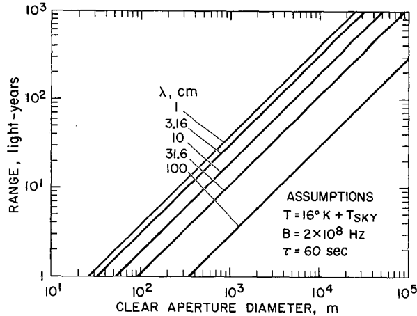
Figure R-1. Radio visibility of the quiet sun.
