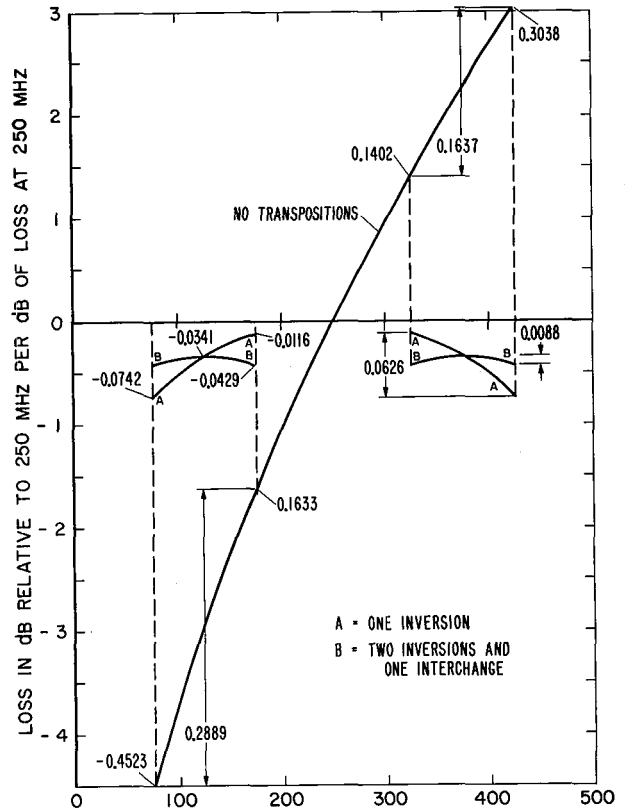
Figure 10-7. Effect of transposition equalization.
