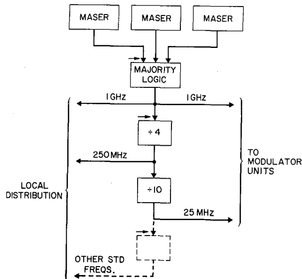
Figure 9-17. Frequency standard.
