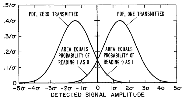
Figure 5-4. Probability density functions—symmetric binary channel ( S/N = 2 ).
