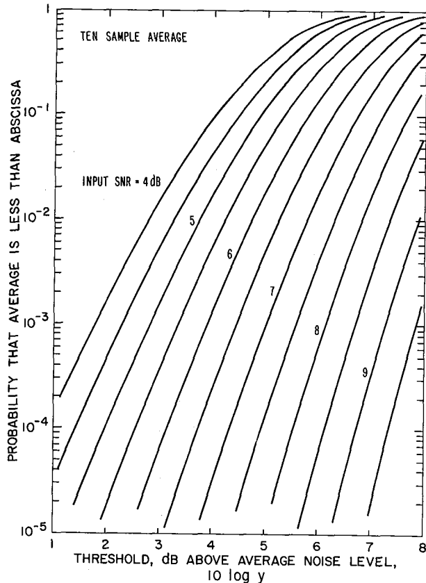
Figure 11-12. Ten sample average of signal plus noise.
