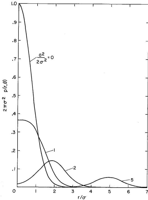
Figure 11-2. Probability density versus radius (Golay detector).
