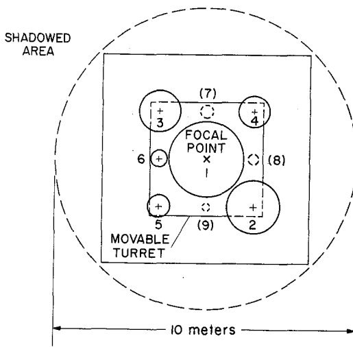
Figure 9-5c. XY displaceable receiver turret for on-axis feeds.
