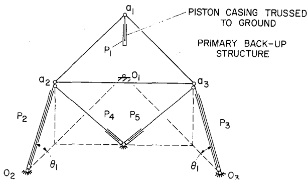
Figure F-3. Machine structure schematic.
