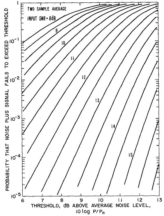
Figure Q-3. Two-sample average of signal plus noise.
