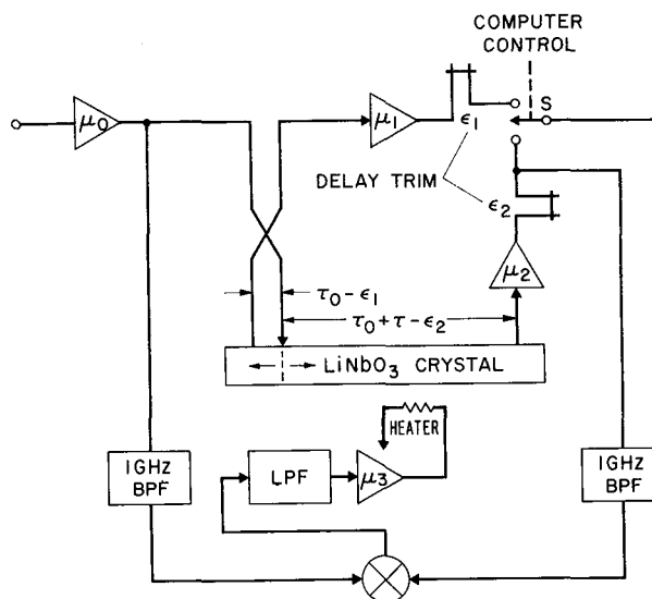
Figure 10-11. Acoustic delay unit.
