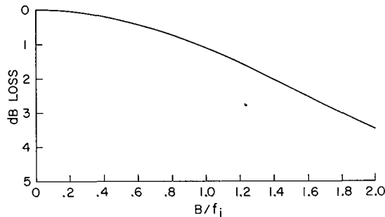
Figure M-3. Decorrelation loss produced by delay phasing.
