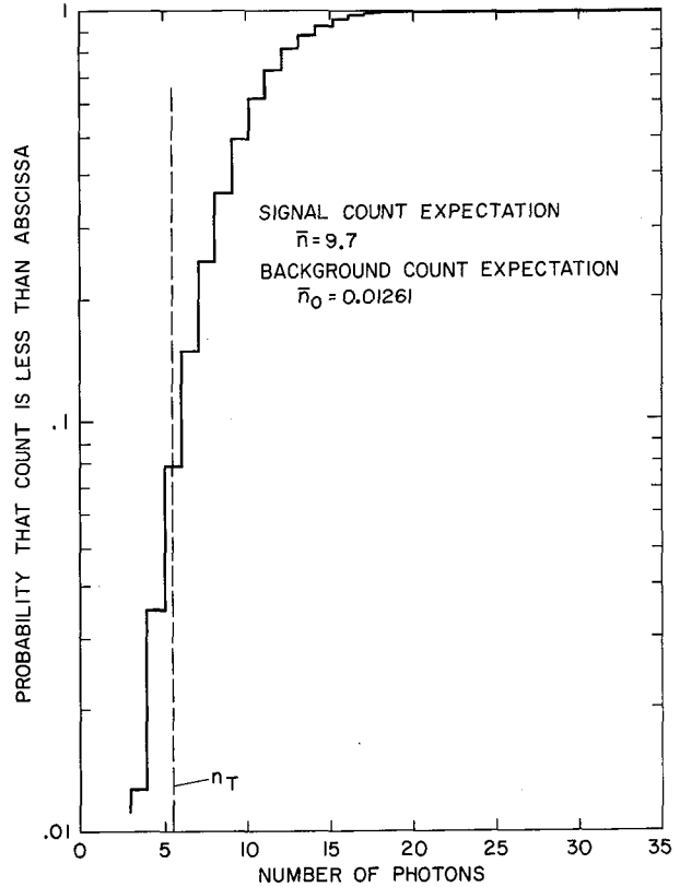
Figure 5-7. Photon count distribution.
