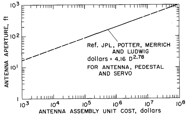
Figure 8-5. Diameter versus antenna unit cost.
