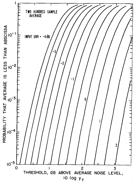
Figure Q-8. One-hundred sample average of signal plus noise. Figure Q-9. Two-hundred sample average of signal plus noise.
