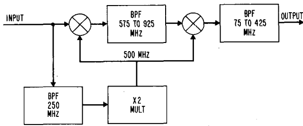
Figure 10-8. Channel inverter.
