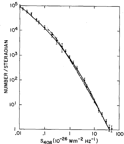
Figure 7-4. \log N - \log S relation at 408 MHz. Units of S are 10^{-26} \text{ W/m}^2 \text{ Hz} . (Pooley and Ryle, 1968)
