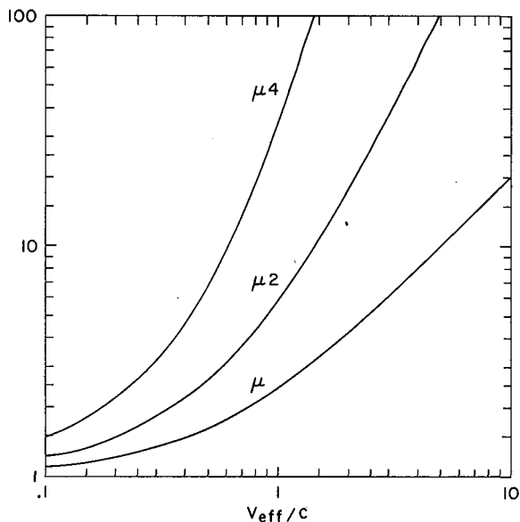
Figure 4-1. Performance of the ideal photon rocket.
