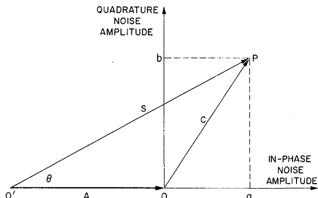
Figure D-1. Noise and signal vectors. P has a two-dimensional Gaussian distribution about O, which makes C have a Rayleigh distribution in amplitude, and S have the distribution given by equation (D34).
