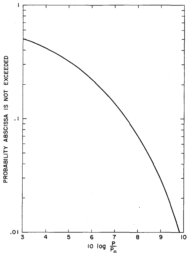
Figure 5-6. Probability of missing signal.
