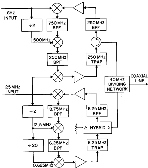
Figure 9-18. Modulator unit.
