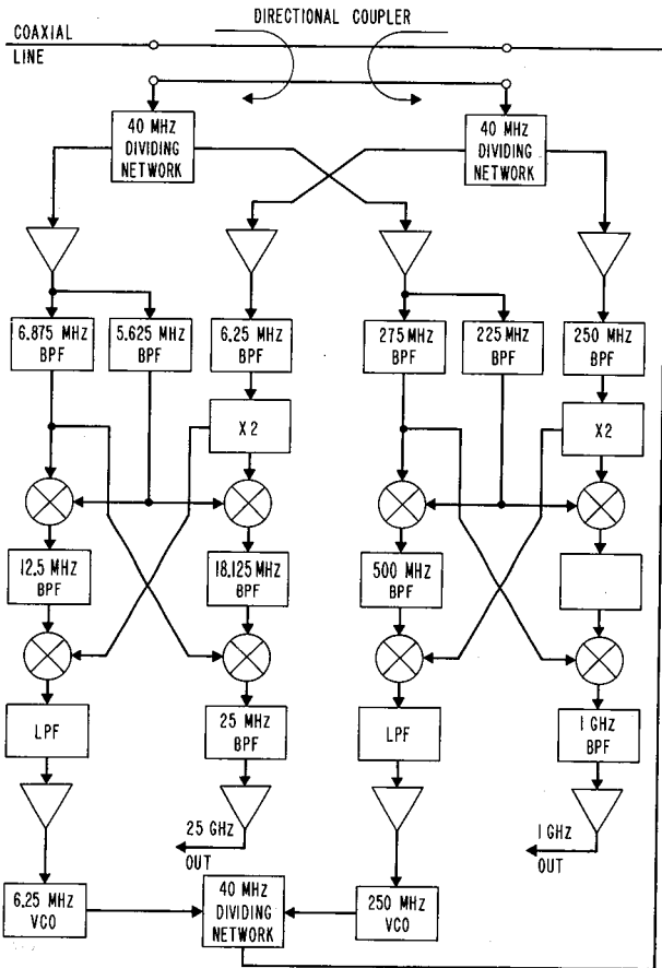
Figure 9-20. Terminator unit.
