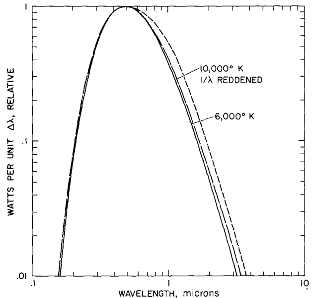
Figure 13-3. Effect of reddening on black-body radiation.
