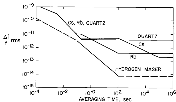
Figure 9-11. Fractional frequency fluctuation versus averaging time.
