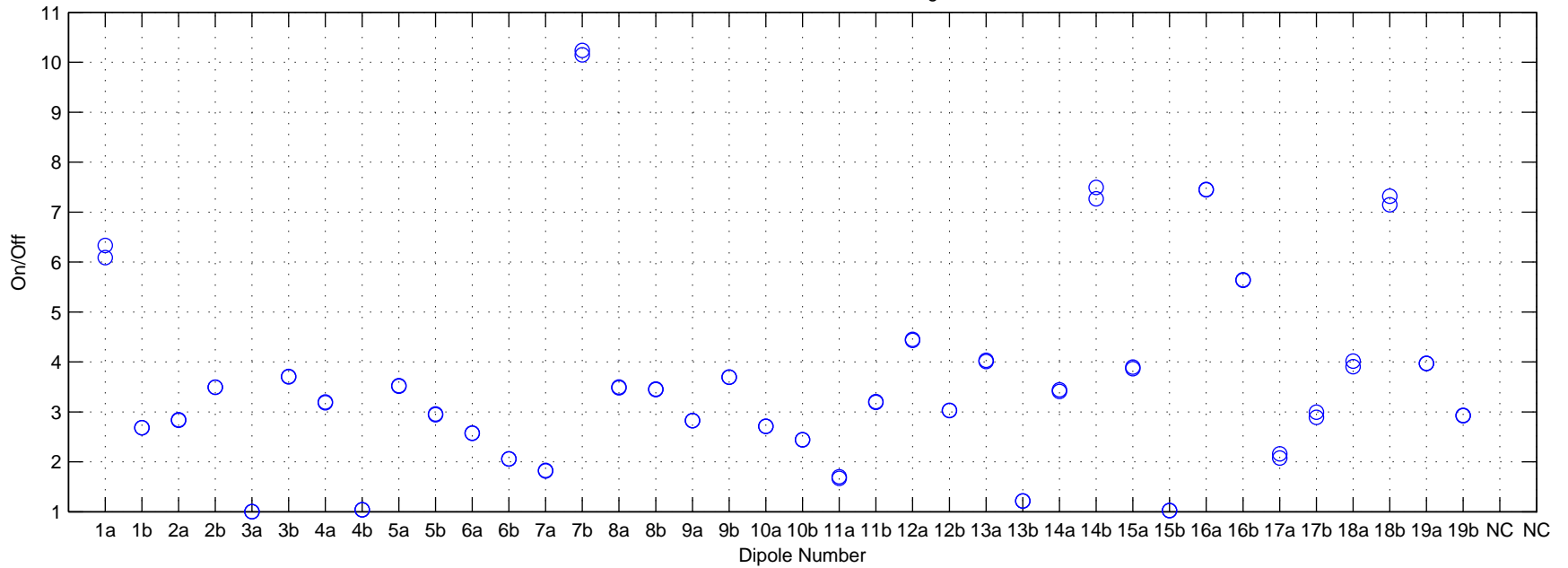
On/Off Y-Factors 1397.7539 MHz Dataset: /media/Disk0/08_03_2013_morning_moon_onoff
