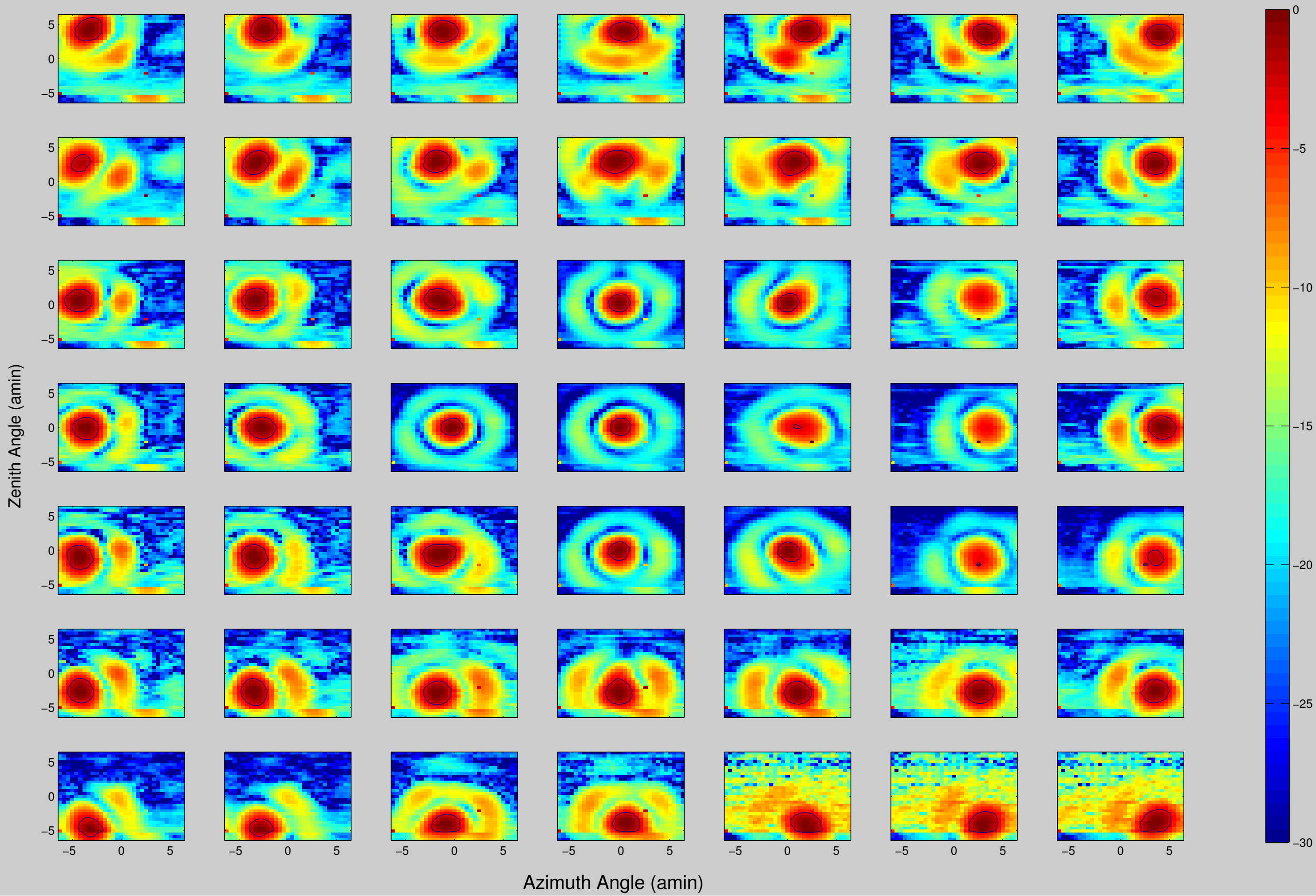
Formed Beams for Grid /media/Disk0/08_02_2013_evening_31x31/default.mat, Frequency 1664.707 MHz, Both Polarizations
