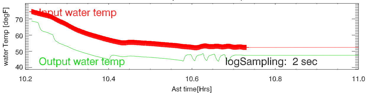
160423 bldll evaporator water temp vs time
