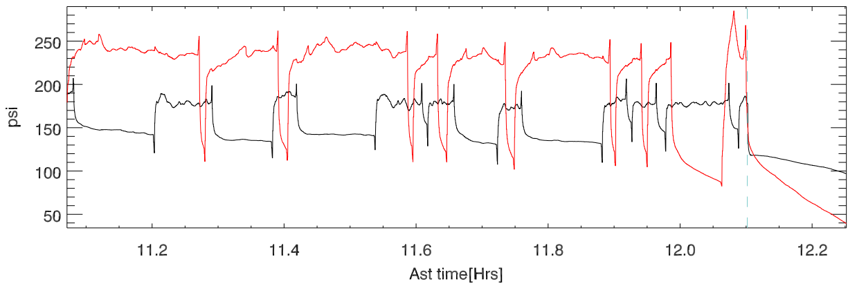
160411 differential refrigerant pressure
