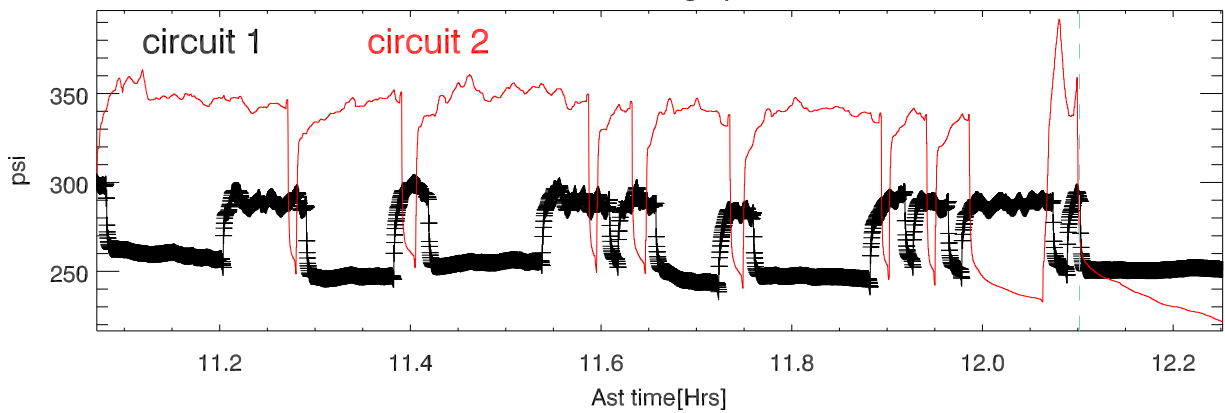
160411 discharge pressure
