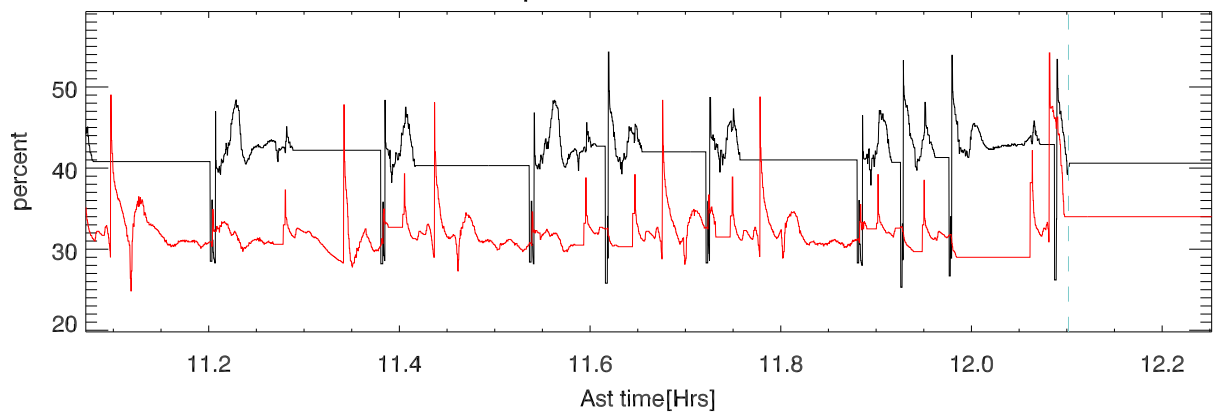
160411 expansion valve, flow command
