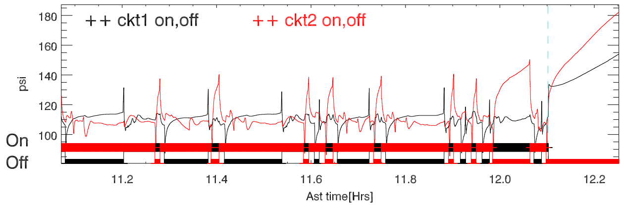
160411 discharge pressure
