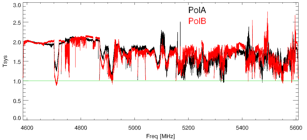
CalDeflection/Tsys
