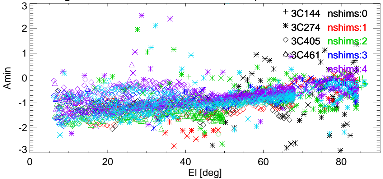
Az Pointing error vs EI for various shims. freq=8789 Pol:A RemoveBase.
