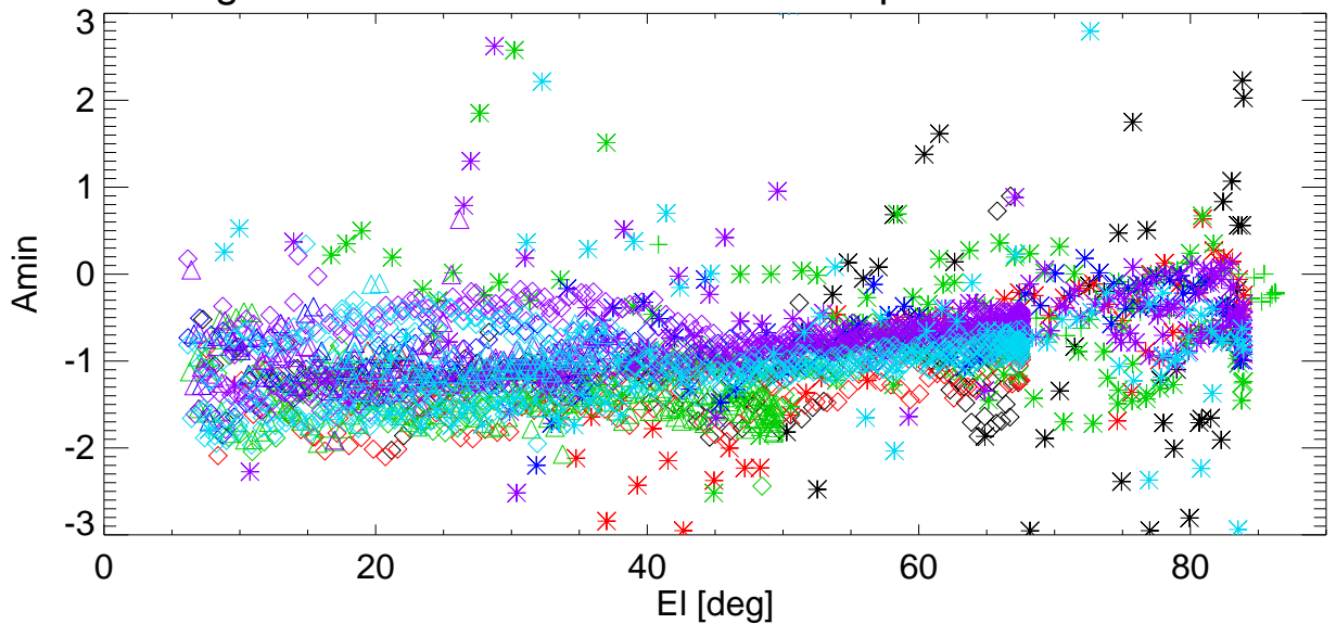
Az Pointing error vs EI for various shims. freq=8789 Pol:B RemoveBase.
