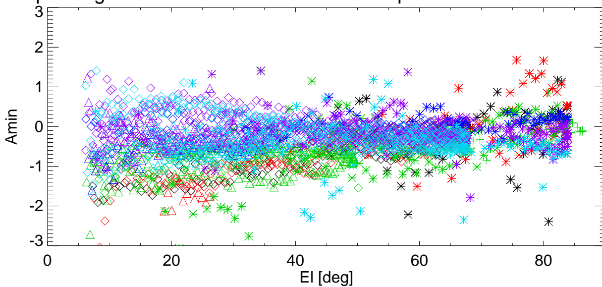
El pointing error vs El for various shims. freq=8789 Pol:B RemoveBase.
