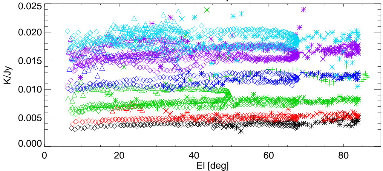
Gain vs EI for various shims. freq=8789 Pol:B RemoveBase.
