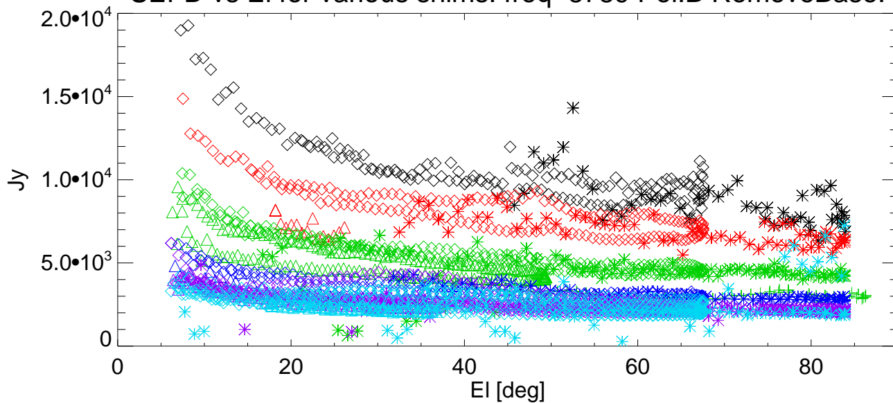
SEFD vs EI for various shims. freq=8789 Pol:B RemoveBase.
