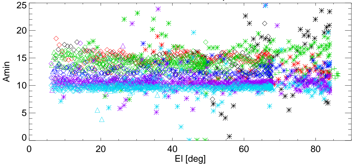
Az BmWidth vs EI for various shims. freq=8789 Pol:B RemoveBase.
