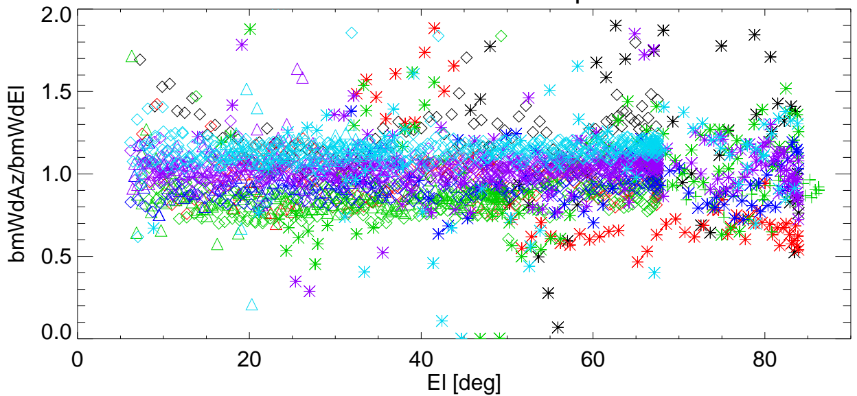
Az/EI BmWdRatio vs EI for various shims. freq=8789 Pol:B RemoveBase.
