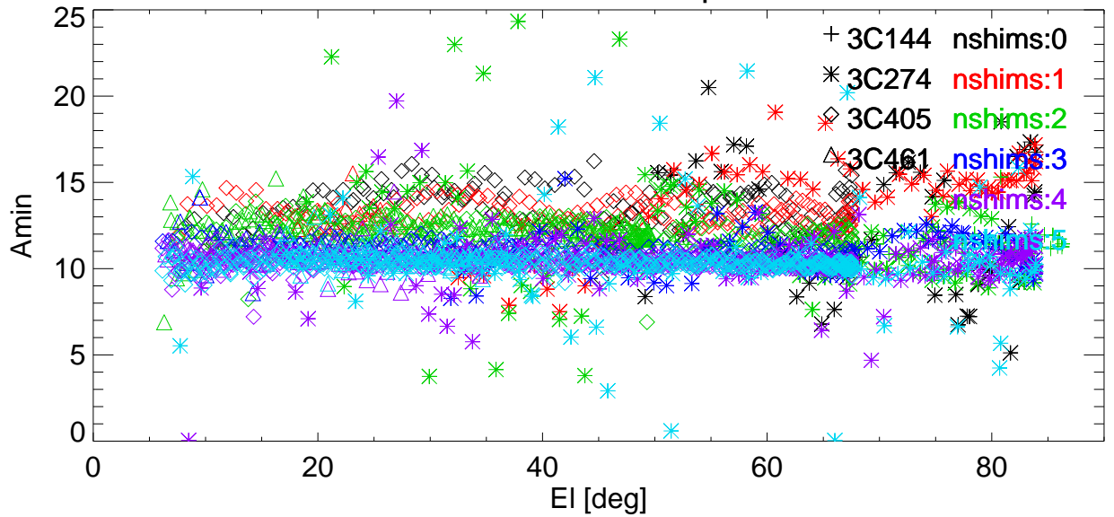
El BmWidth vs El for various shims. freq=8789 Pol:A RemoveBase.
