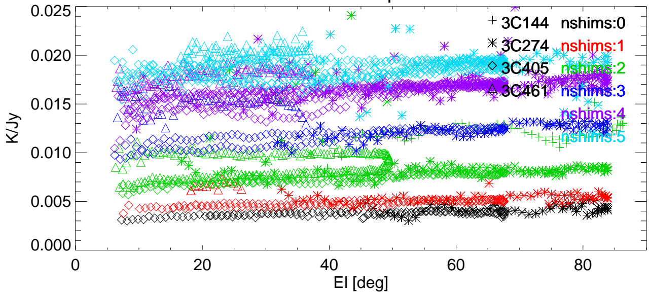
Gain vs EI for various shims. freq=8789 Pol:A RemoveBase.
