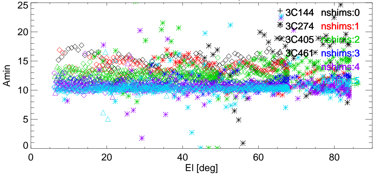
Az BmWidth vs EI for various shims. freq=8789 Pol:A RemoveBase.
