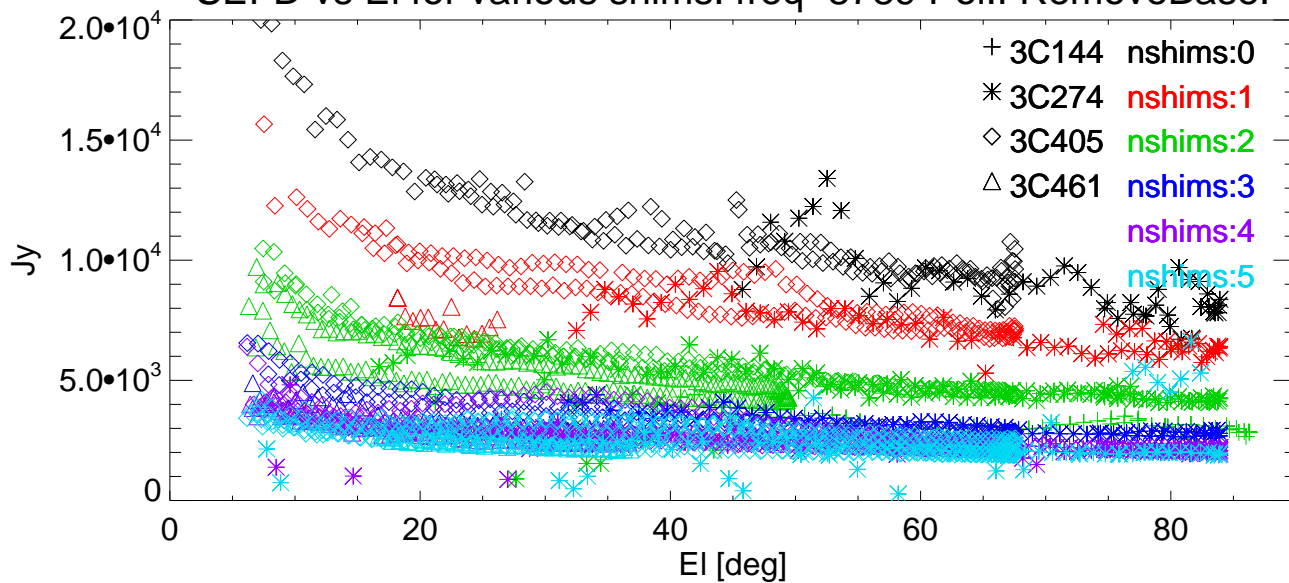
SEFD vs EI for various shims. freq=8789 Pol:A RemoveBase.
