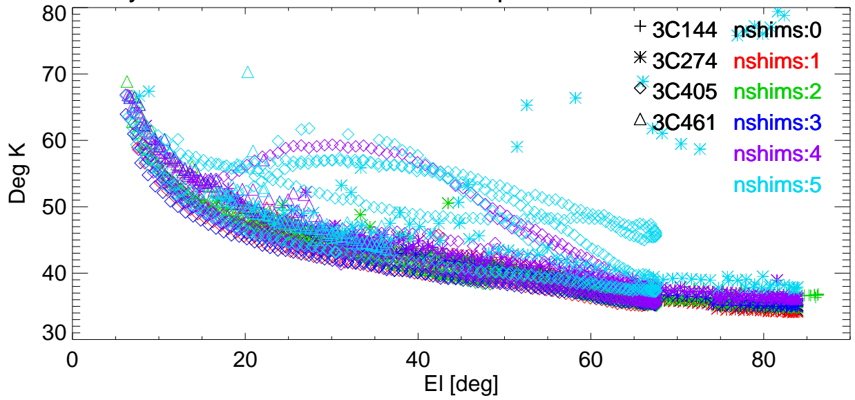
Tsys vs EI for various shims. freq=8789 Pol:A RemoveBase.
