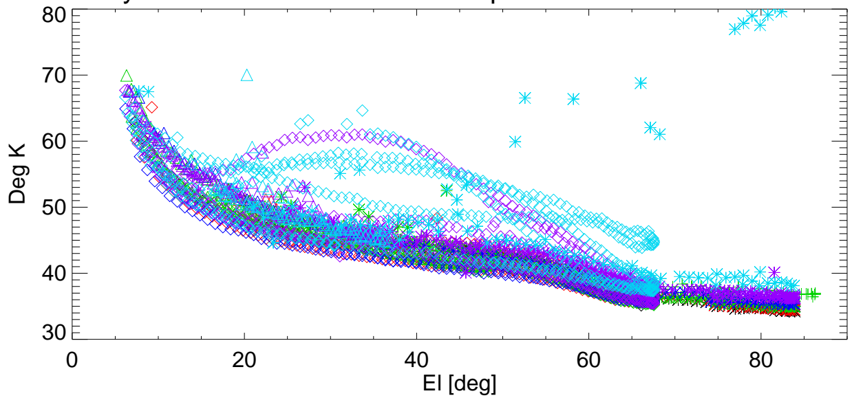
Tsys vs EI for various shims. freq=8789 Pol:B RemoveBase.
