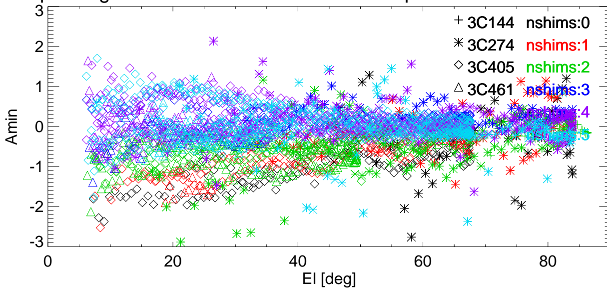
El pointing error vs El for various shims. freq=8789 Pol:A RemoveBase.
