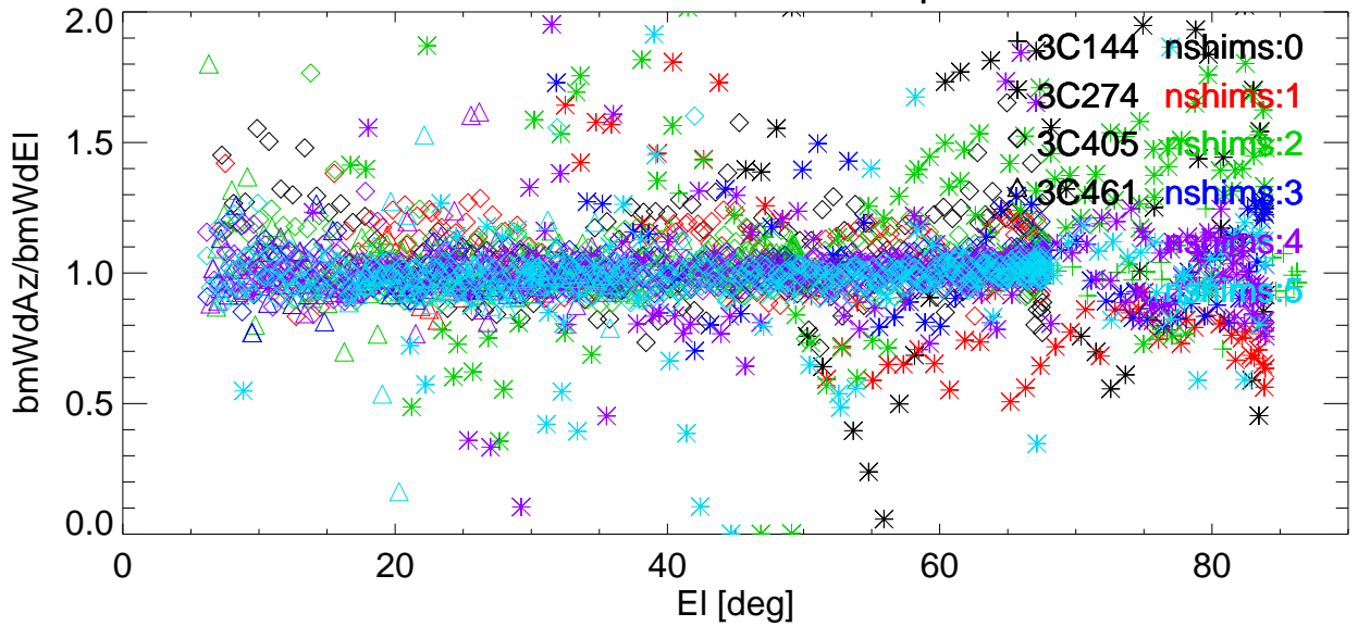
Az/EI BmWdRatio vs EI for various shims. freq=8789 Pol:A RemoveBase.
