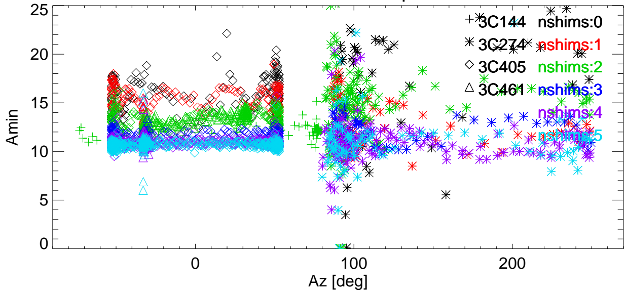
Az BmWidth vs Az for various shims. freq=8363 Pol:A RemoveBase.
