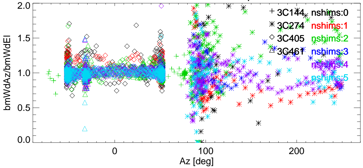
Az/EI BmWdRatio vs Az for various shims. freq=8363 Pol:A RemoveBase.
