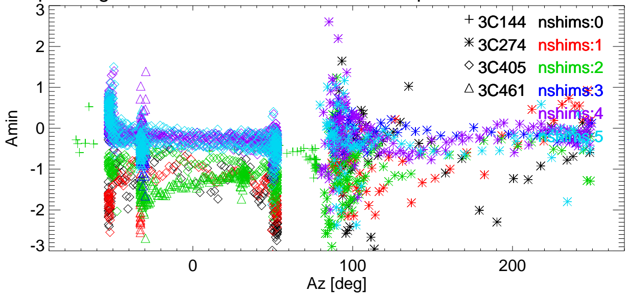
El pointing error vs Az for various shims. freq=8363 Pol:A RemoveBase.
