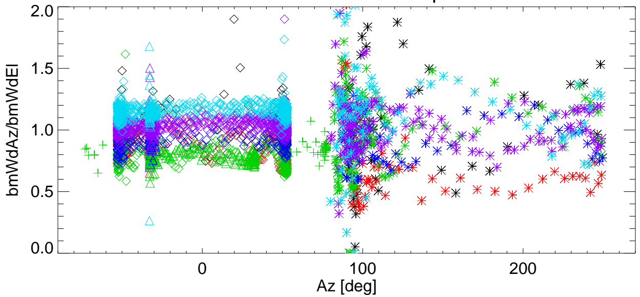
Az/EI BmWdRatio vs Az for various shims. freq=8363 Pol:B RemoveBase.
