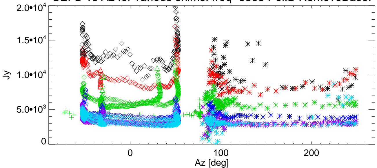
SEFD vs Az for various shims. freq=8363 Pol:B RemoveBase.
