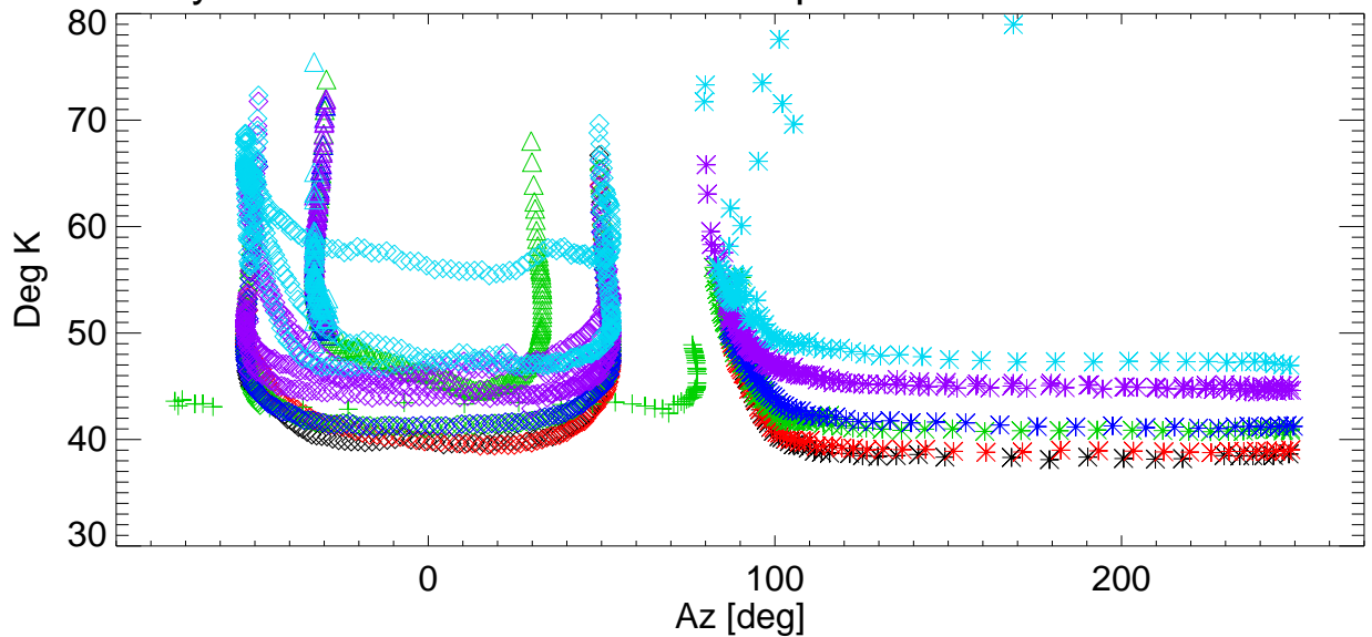
Tsys vs Az for various shims. freq=8363 Pol:B RemoveBase.
