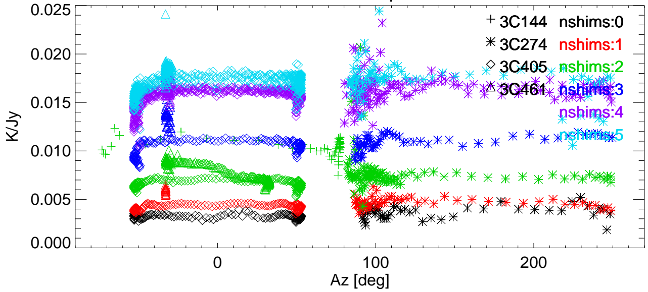
Gain vs Az for various shims. freq=8363 Pol:A RemoveBase.
