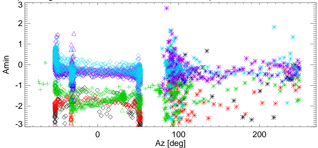
El pointing error vs Az for various shims. freq=8363 Pol:B RemoveBase.
