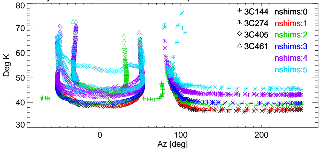
Tsys vs Az for various shims. freq=8363 Pol:A RemoveBase.
