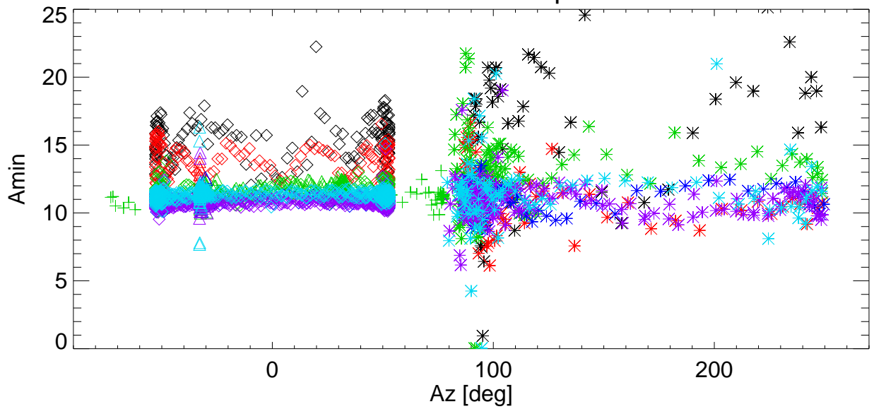
Az BmWidth vs Az for various shims. freq=8363 Pol:B RemoveBase.
