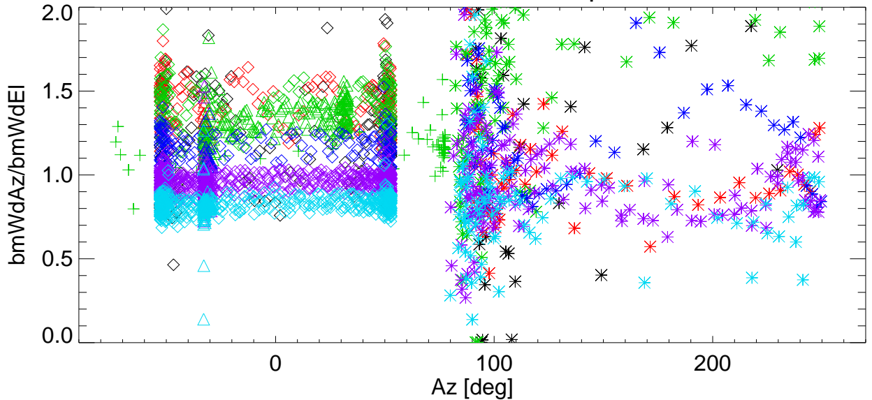
Az/EI BmWdRatio vs Az for various shims. freq=8363 Pol:B RemoveBase.
