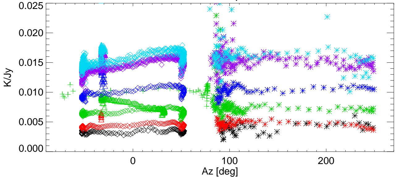
Gain vs Az for various shims. freq=8363 Pol:B RemoveBase.
