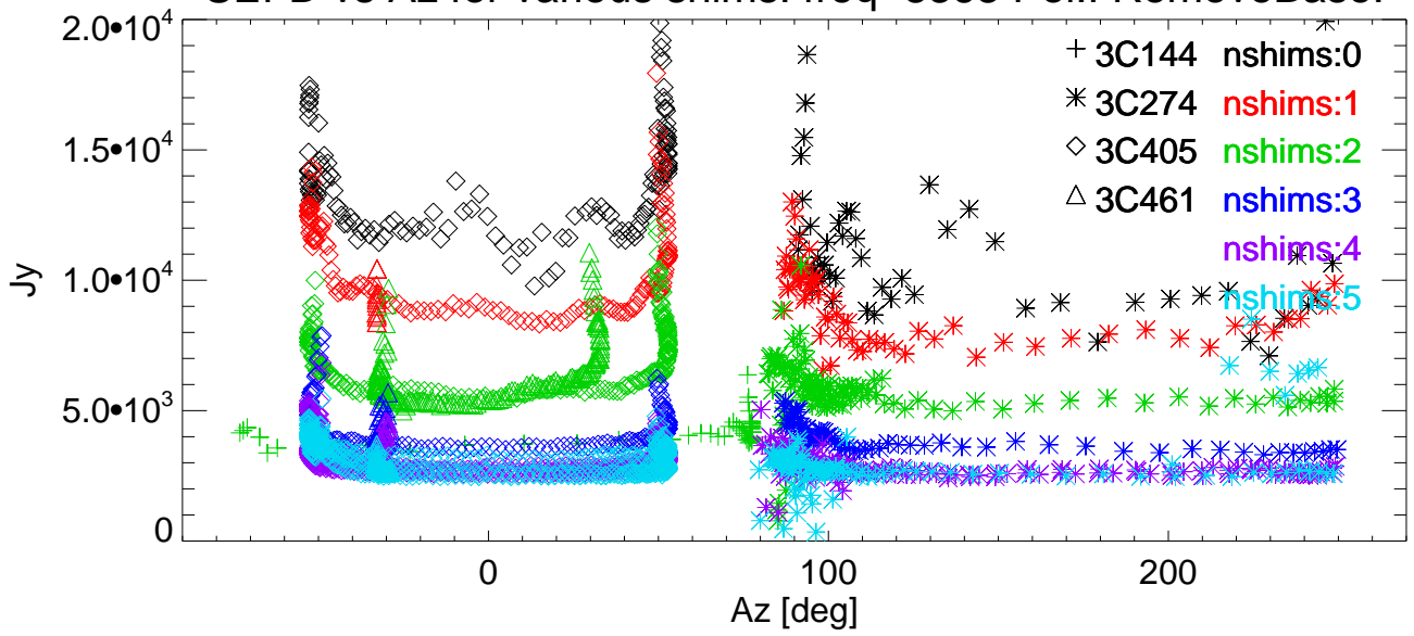
SEFD vs Az for various shims. freq=8363 Pol:A RemoveBase.
