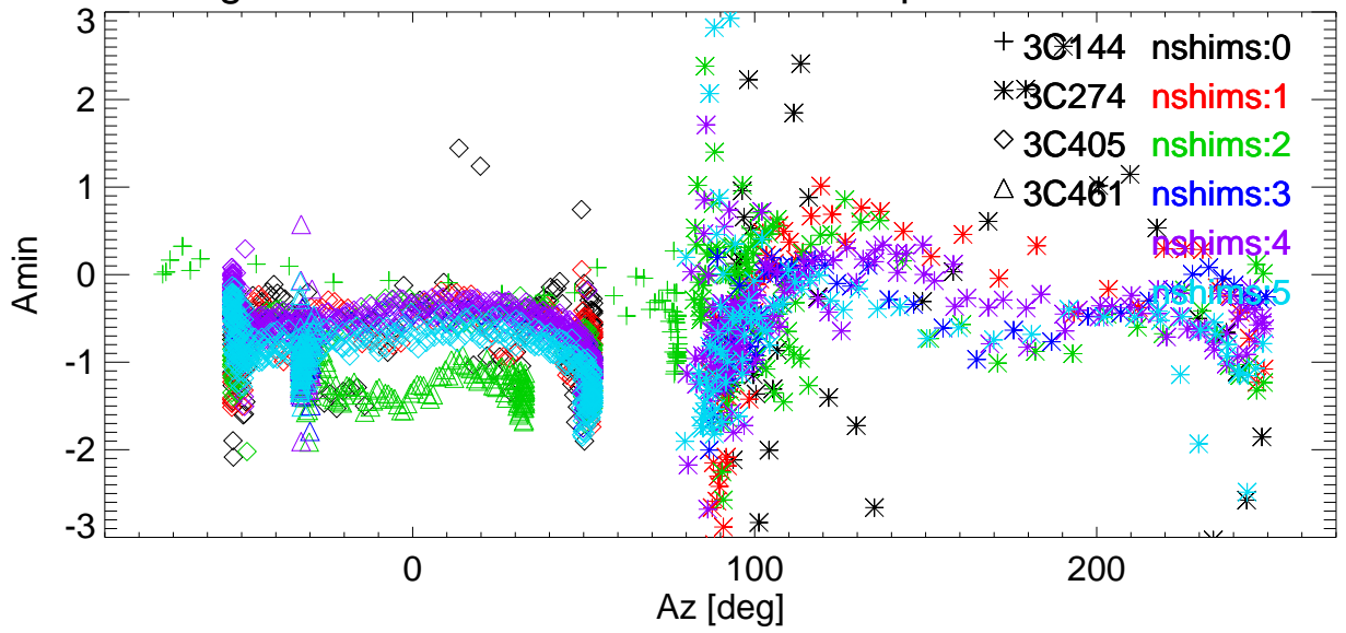
Az Pointing error vs Az for various shims. freq=8363 Pol:A RemoveBase.
