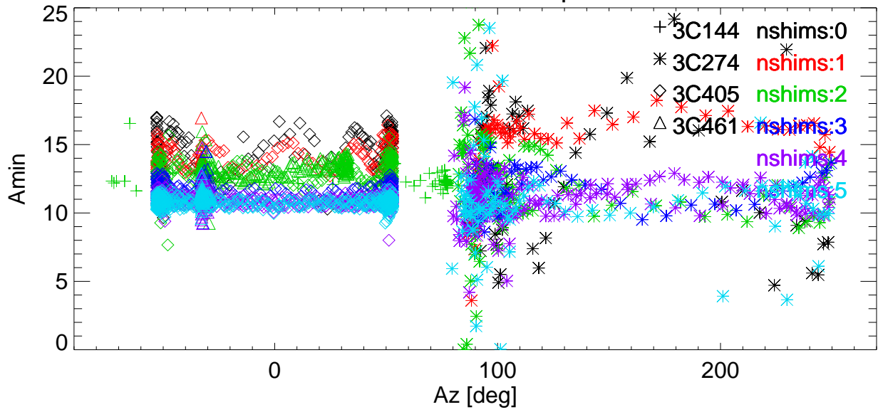
El BmWidth vs Az for various shims. freq=8363 Pol:A RemoveBase.
