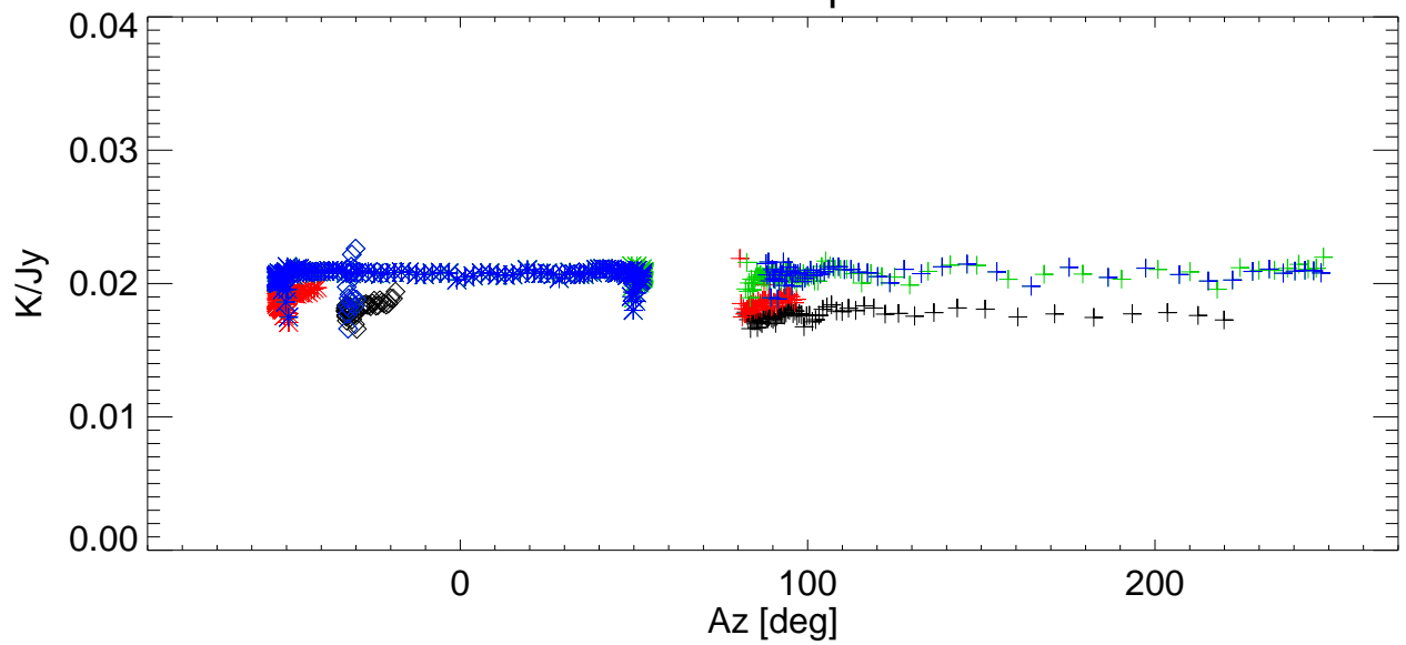
Gain vs Az for various shims. freq=3414 Pol:B RemoveBase.
