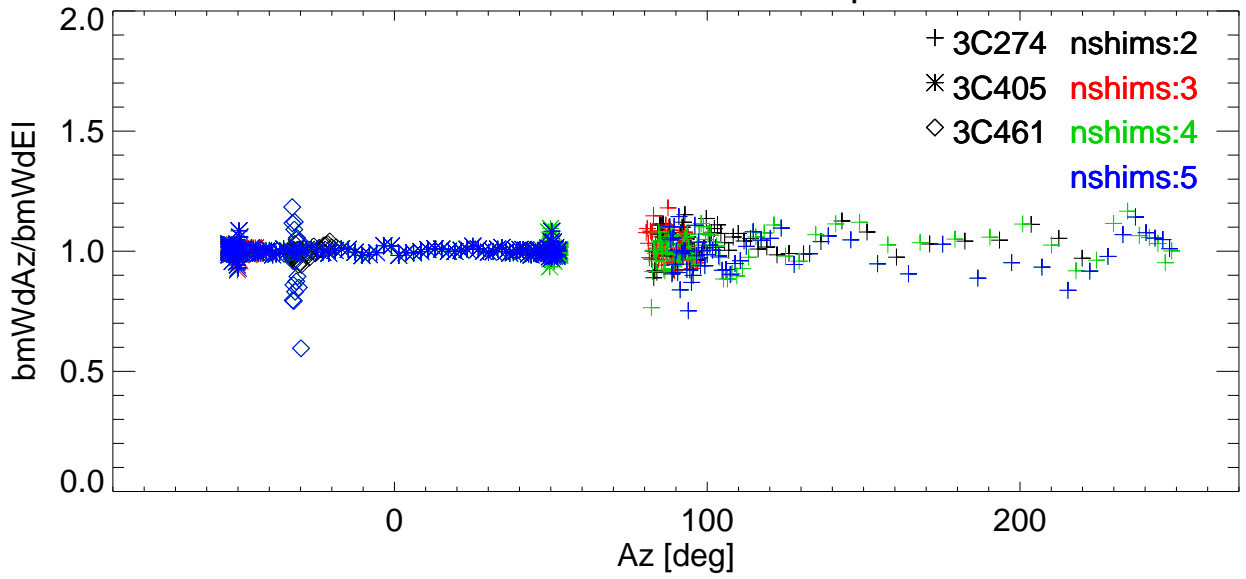
Az/EI BmWdRatio vs Az for various shims. freq=3414 Pol:A RemoveBase.
