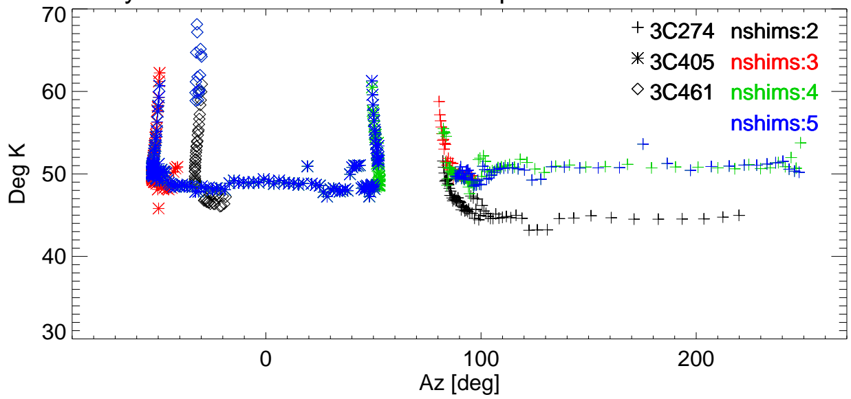
Tsys vs Az for various shims. freq=3414 Pol:A RemoveBase.
