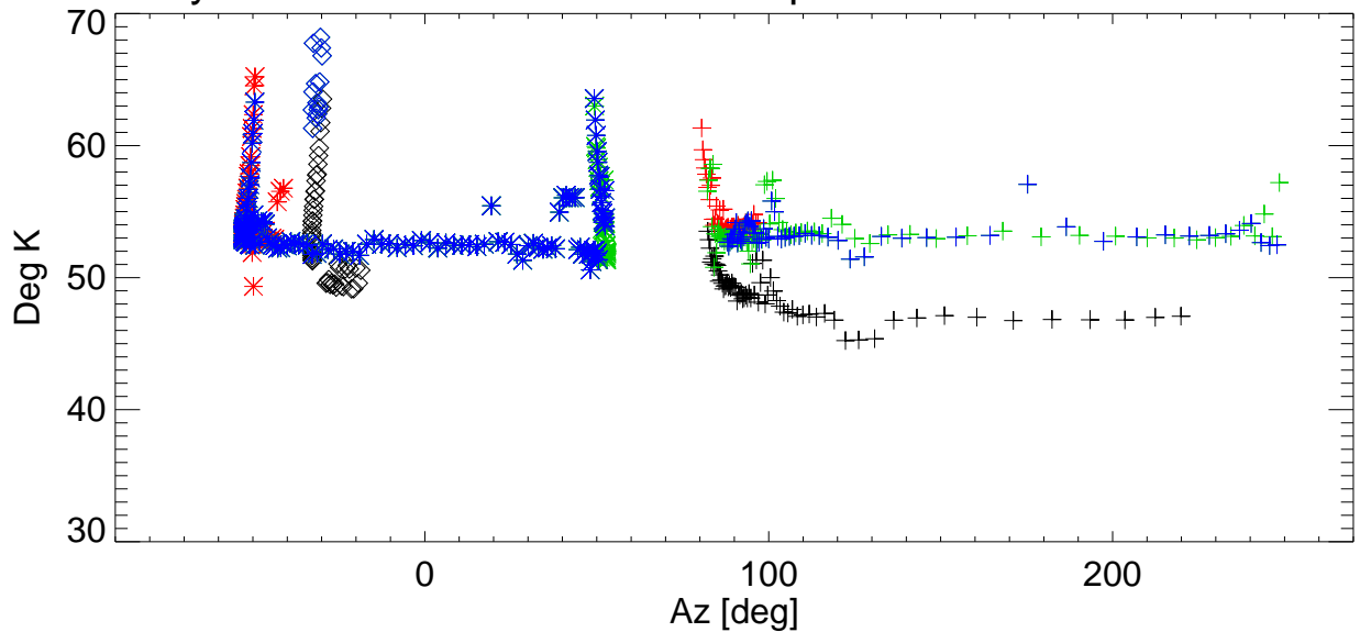
Tsys vs Az for various shims. freq=3414 Pol:B RemoveBase.
