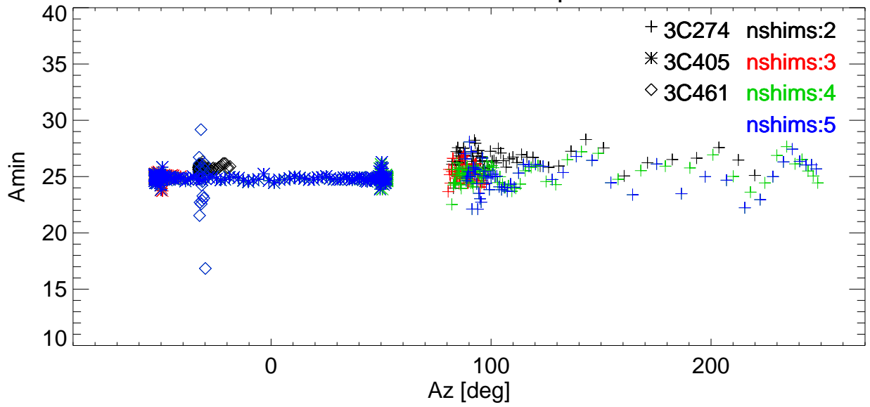
Az BmWidth vs Az for various shims. freq=3414 Pol:A RemoveBase.
