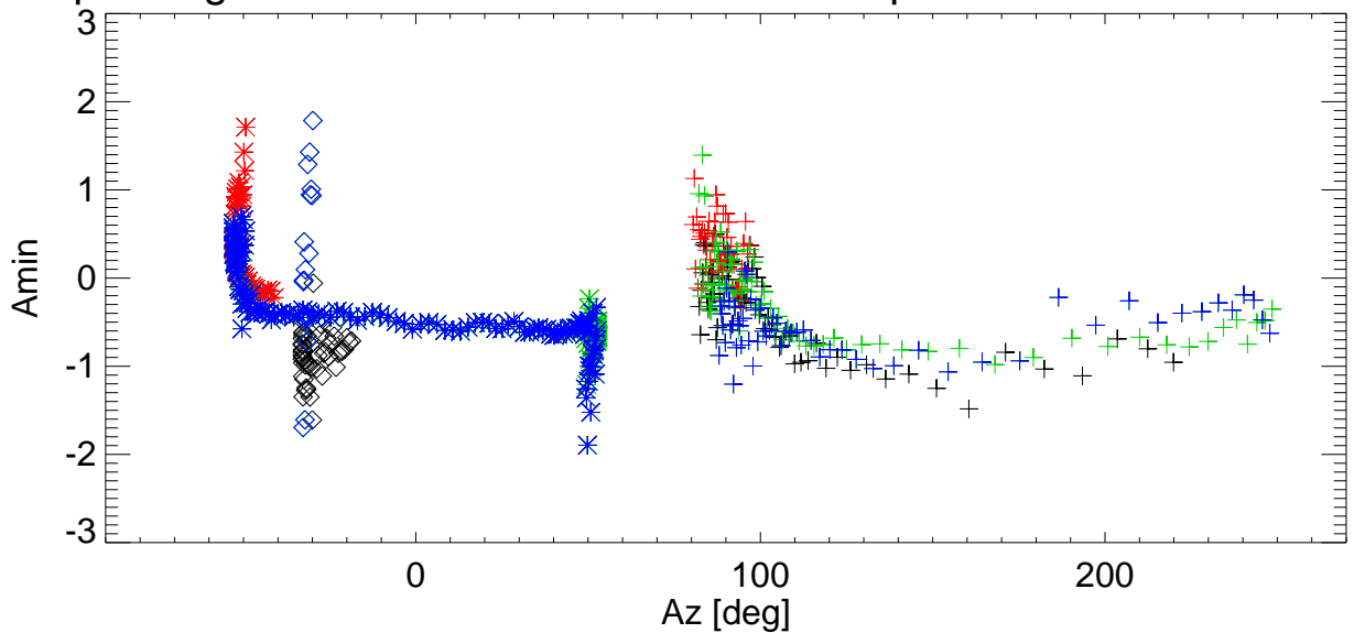
El pointing error vs Az for various shims. freq=3414 Pol:B RemoveBase.
