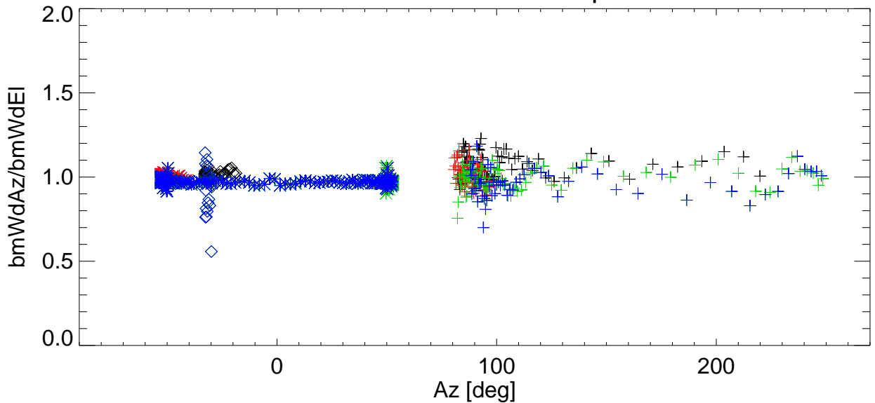
Az/EI BmWdRatio vs Az for various shims. freq=3414 Pol:B RemoveBase.
