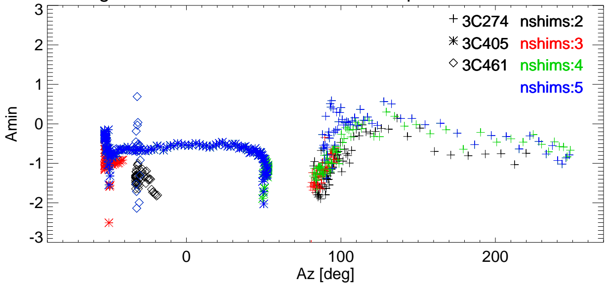
Az Pointing error vs Az for various shims. freq=3414 Pol:A RemoveBase.
