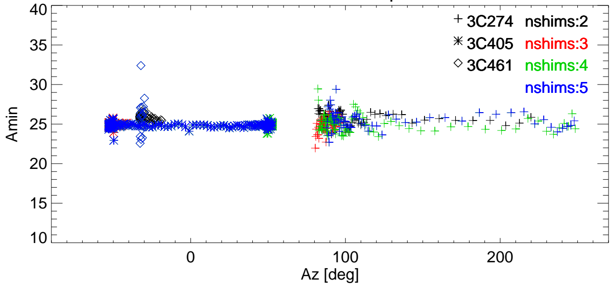
El BmWidth vs Az for various shims. freq=3414 Pol:A RemoveBase.
