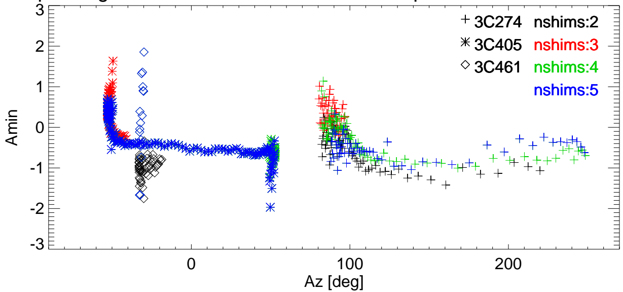
El pointing error vs Az for various shims. freq=3414 Pol:A RemoveBase.
