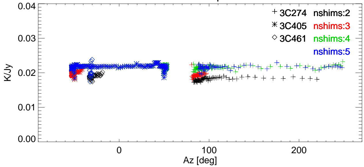
Gain vs Az for various shims. freq=3414 Pol:A RemoveBase.
