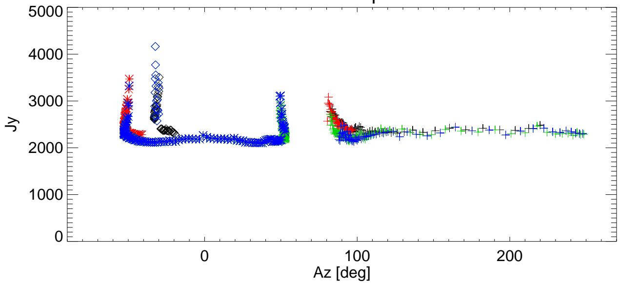
SEFD vs Az for various shims. freq=3414 Pol:B RemoveBase.
