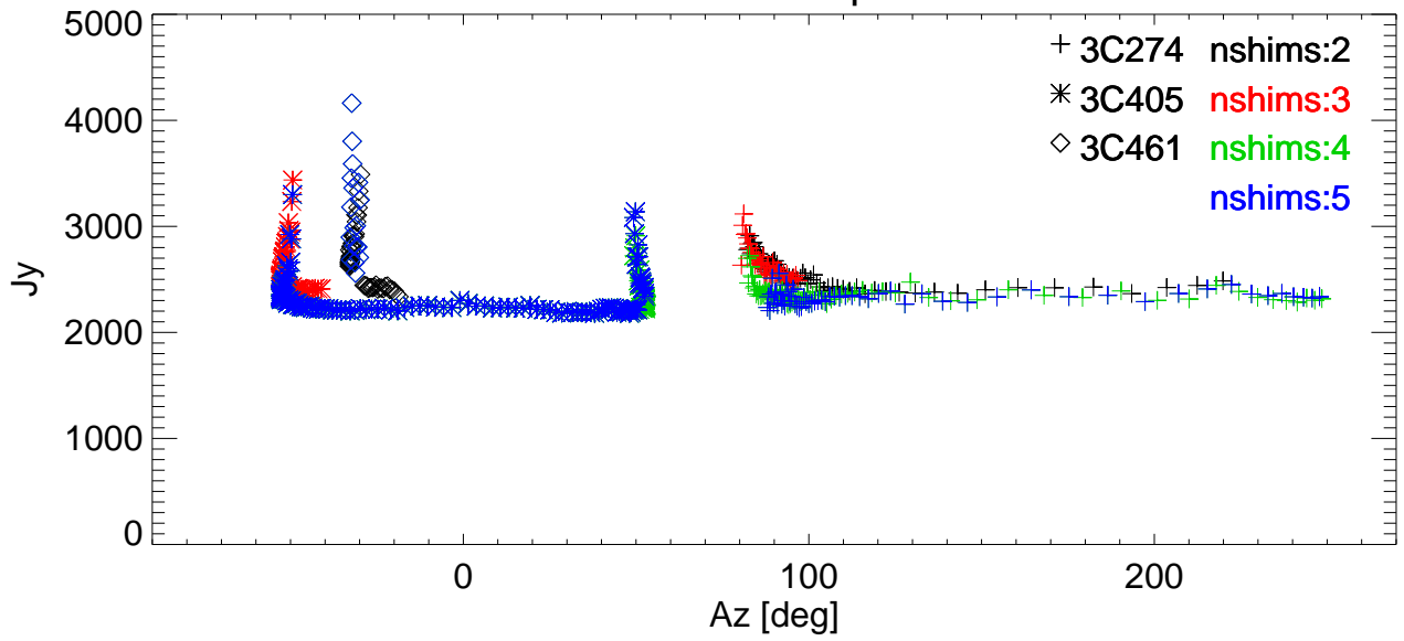
SEFD vs Az for various shims. freq=3414 Pol:A RemoveBase.
