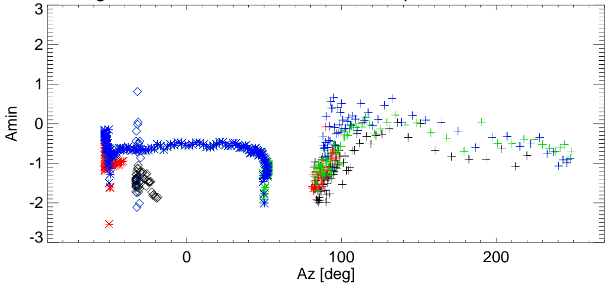
Az Pointing error vs Az for various shims. freq=3414 Pol:B RemoveBase.
