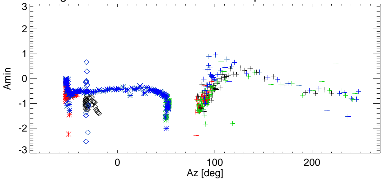
Az Pointing error vs Az for various shims. freq=2988 Pol:B RemoveBase.
