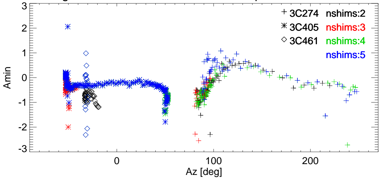
Az Pointing error vs Az for various shims. freq=2988 Pol:A RemoveBase.
