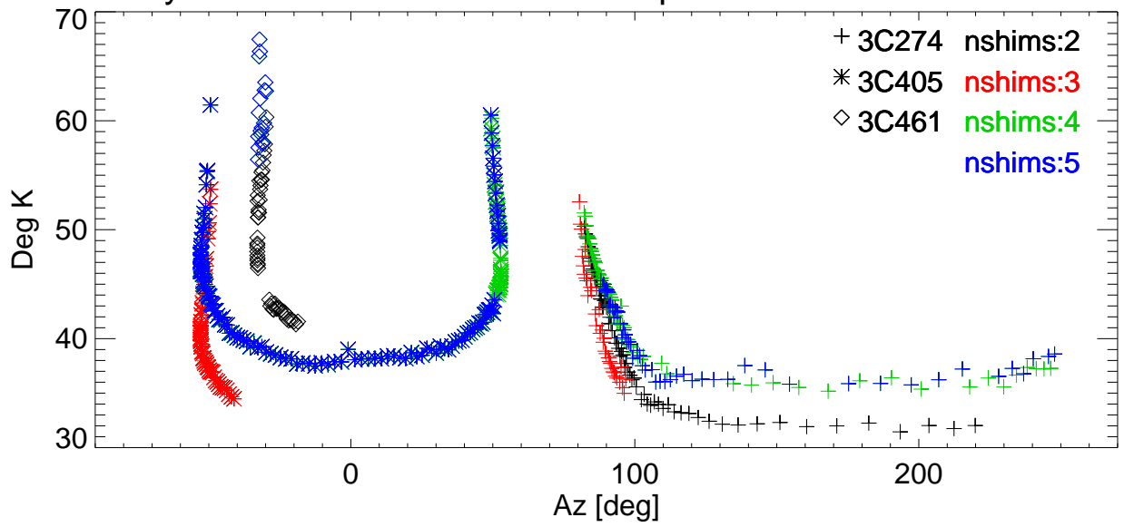
Tsys vs Az for various shims. freq=2988 Pol:A RemoveBase.
