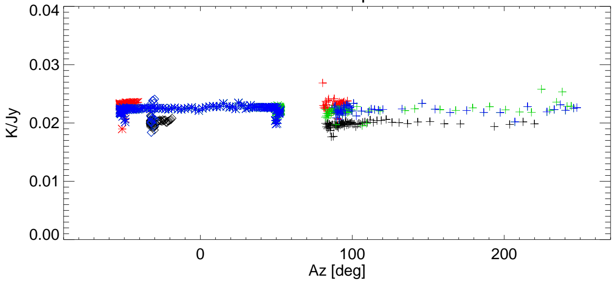
Gain vs Az for various shims. freq=2988 Pol:B RemoveBase.
