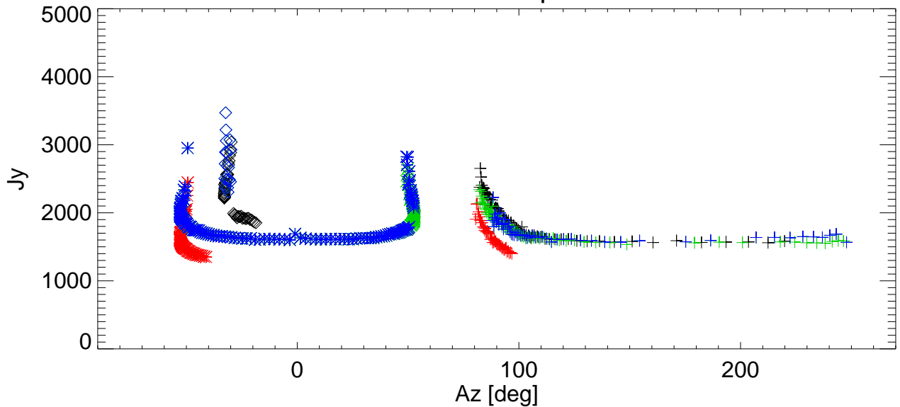
SEFD vs Az for various shims. freq=2988 Pol:B RemoveBase.
