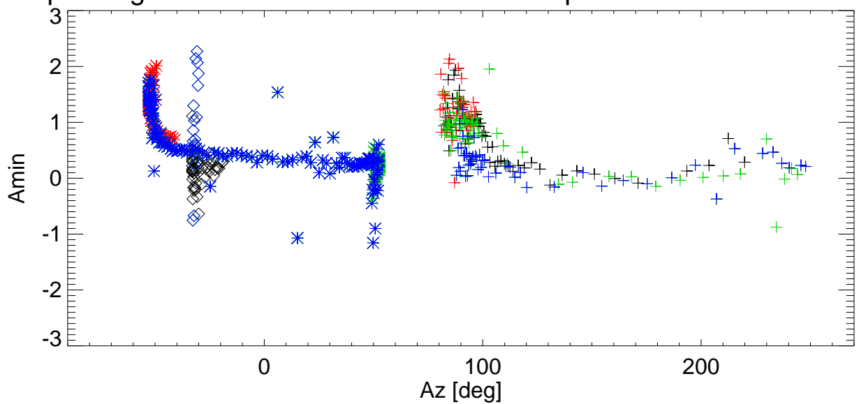
El pointing error vs Az for various shims. freq=2988 Pol:B RemoveBase.
