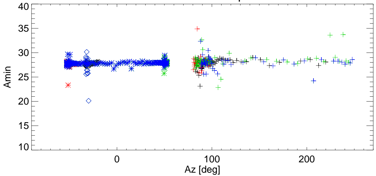
Az BmWidth vs Az for various shims. freq=2988 Pol:B RemoveBase.
