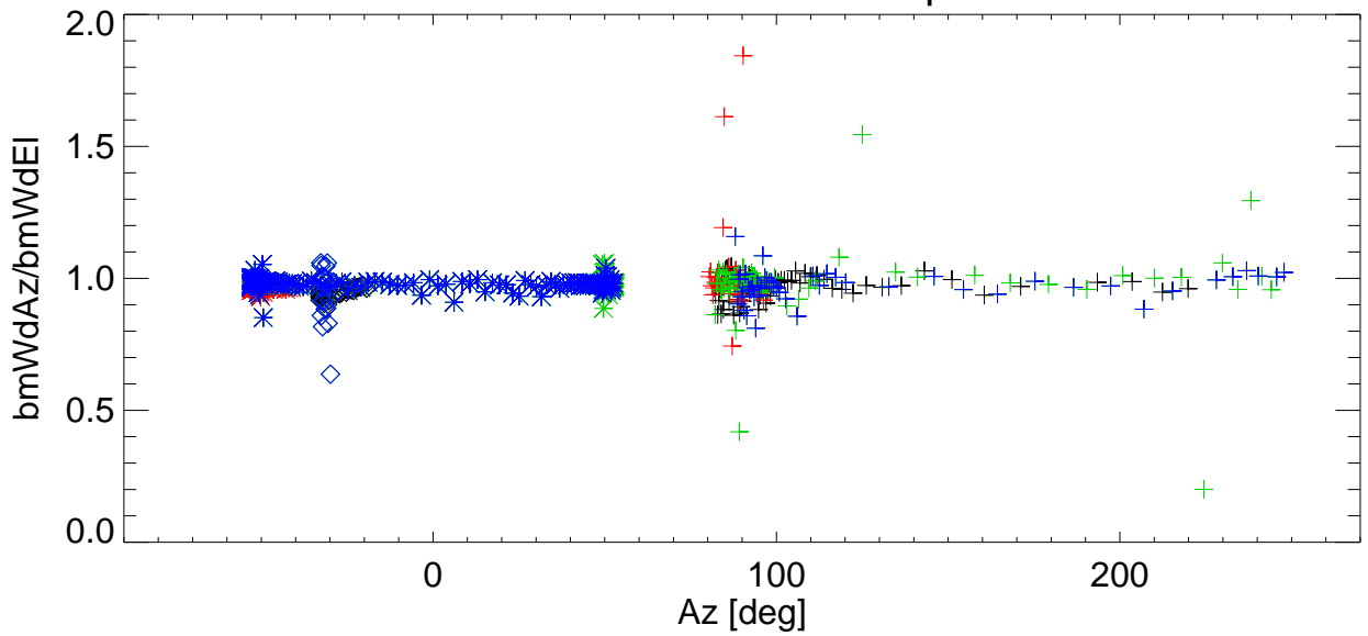
Az/EI BmWdRatio vs Az for various shims. freq=2988 Pol:B RemoveBase.
