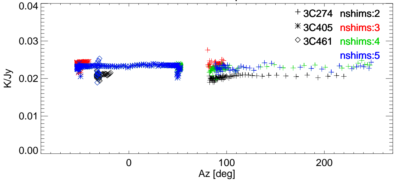
Gain vs Az for various shims. freq=2988 Pol:A RemoveBase.
