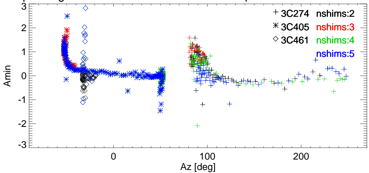
El pointing error vs Az for various shims. freq=2988 Pol:A RemoveBase.
