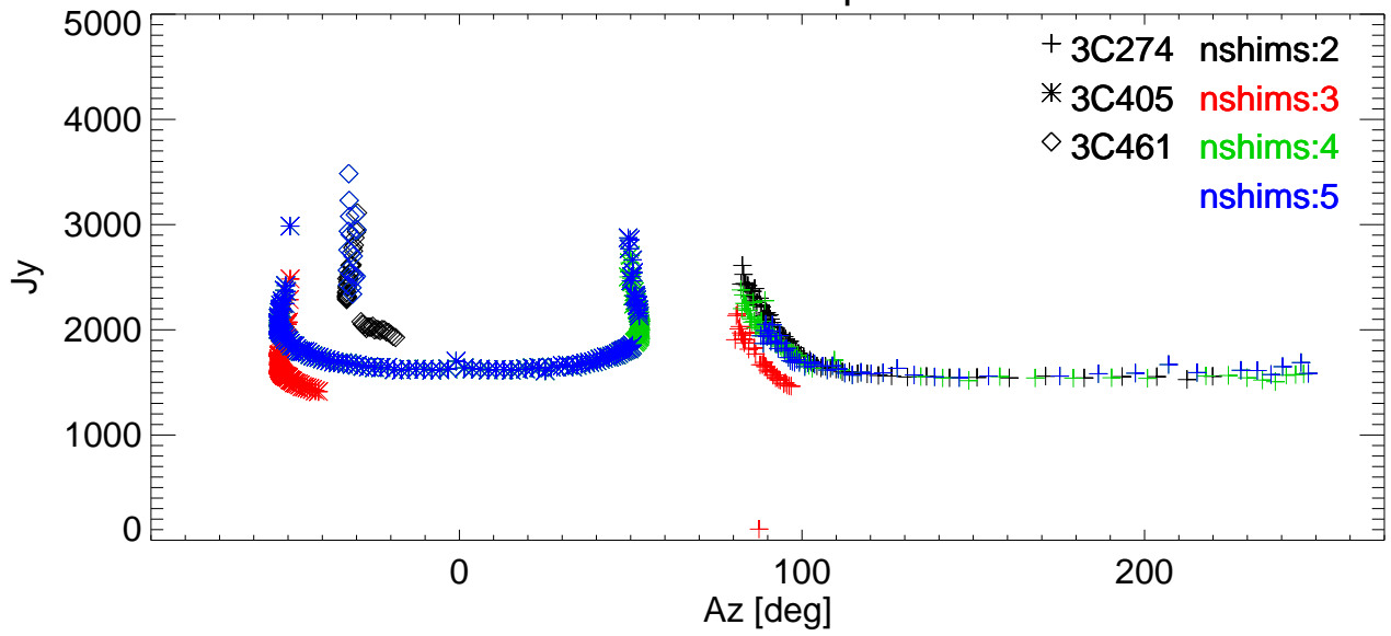
SEFD vs Az for various shims. freq=2988 Pol:A RemoveBase.
