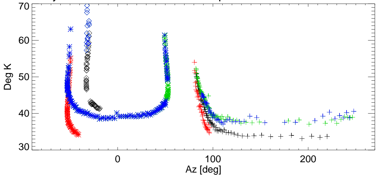
Tsys vs Az for various shims. freq=2988 Pol:B RemoveBase.
