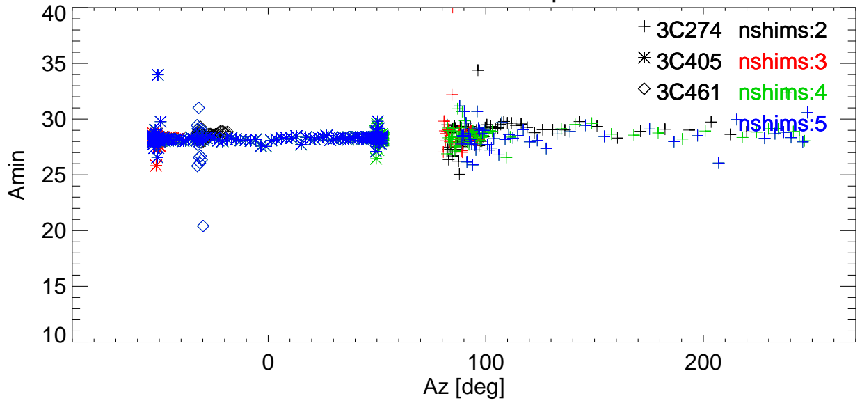
Az BmWidth vs Az for various shims. freq=2988 Pol:A RemoveBase.
