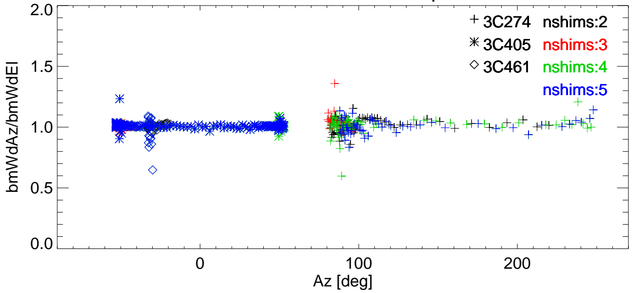
Az/EI BmWdRatio vs Az for various shims. freq=2988 Pol:A RemoveBase.
