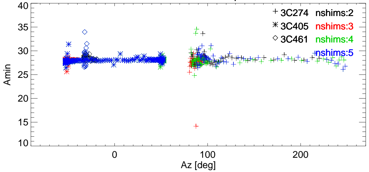
El BmWidth vs Az for various shims. freq=2988 Pol:A RemoveBase.
