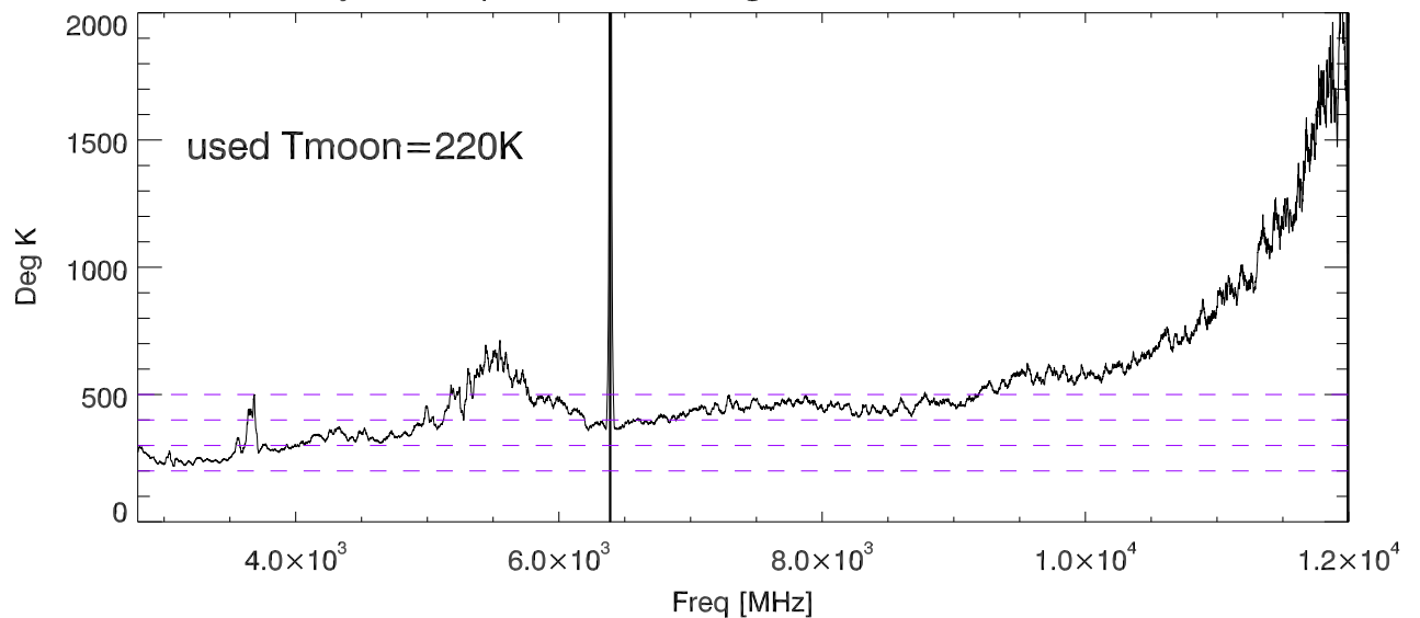
12meter Tsys vs freq with QRFH using moon and bmSize,offset correction
