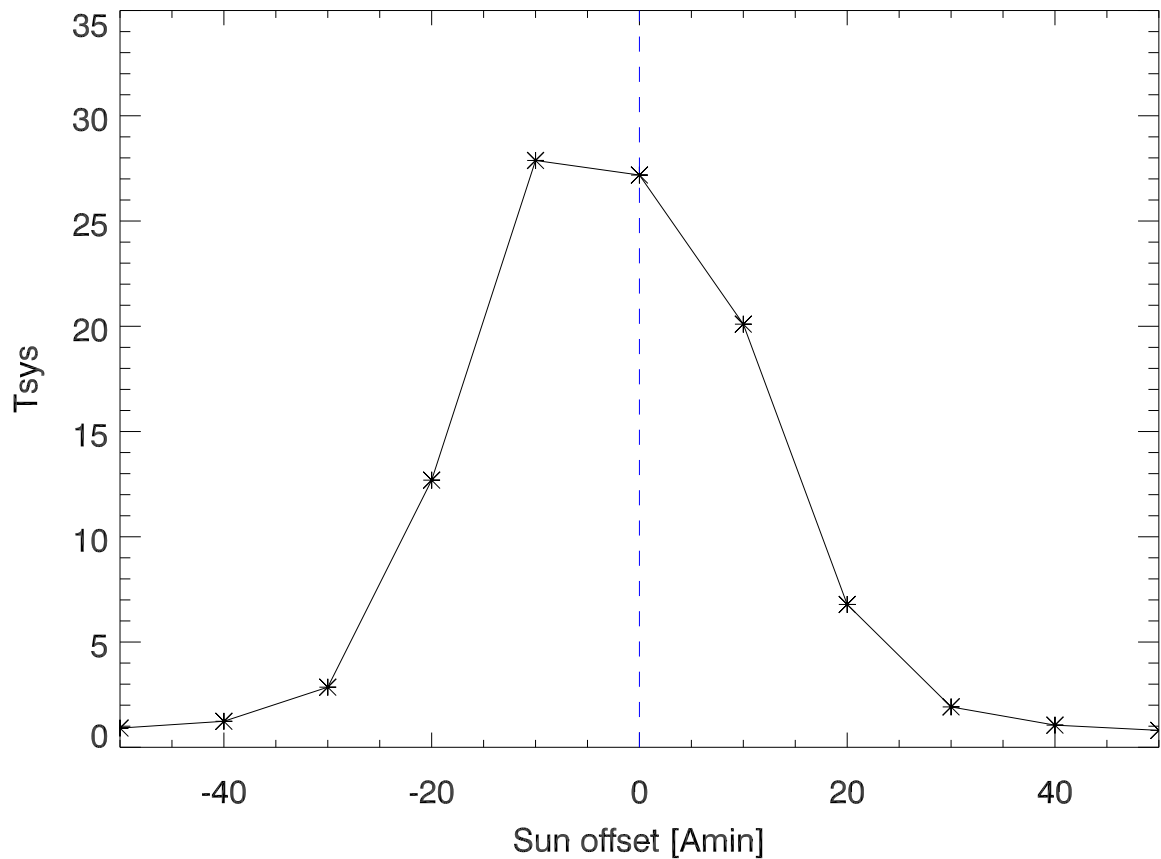
Total power vs az offset for azstrip (11 pnts)
