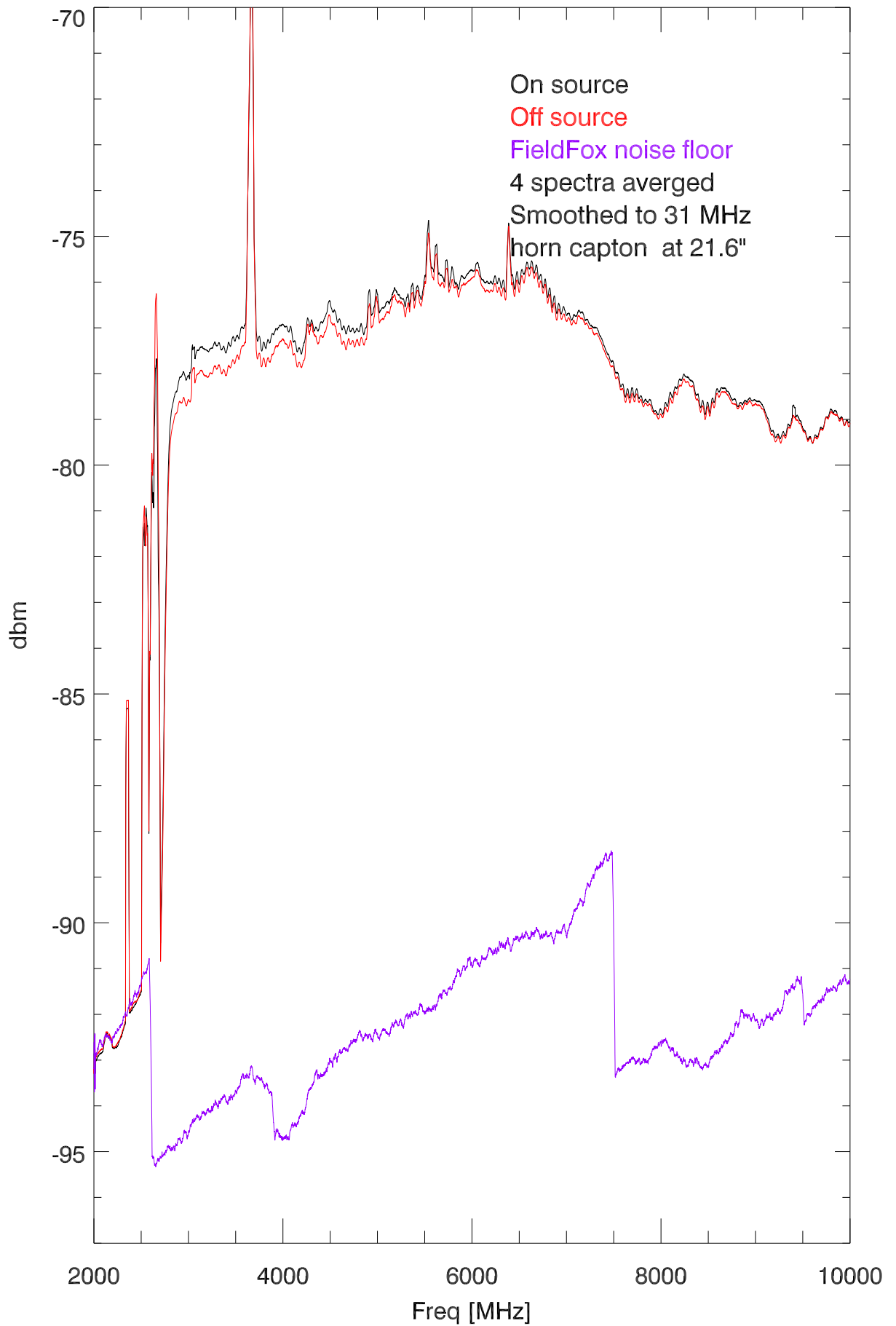
220617 QRFH: 4 Position switches on CasA. on,off spectra
