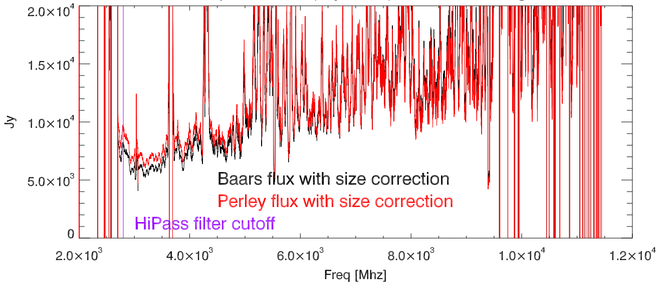
Computed SEFD (Tsys/Gain) 31Mhz smoothing
