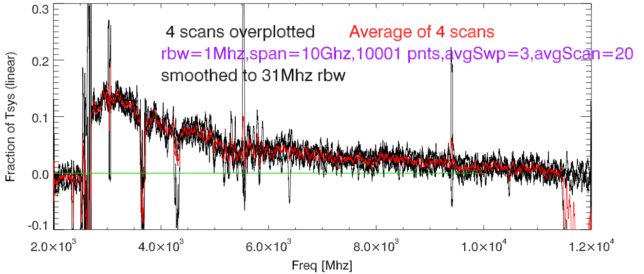
CasA (SrcDeflection/Tsys -1) (4 (on-off)/off -1 scans)
