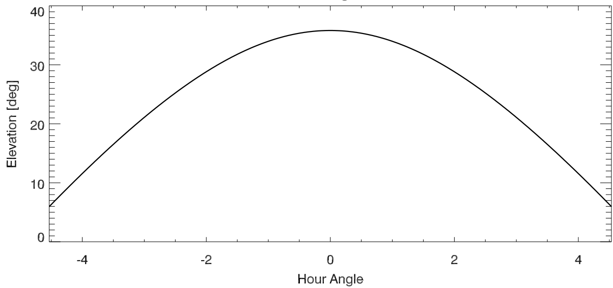
elevation vs hour angle for: NGC6334
