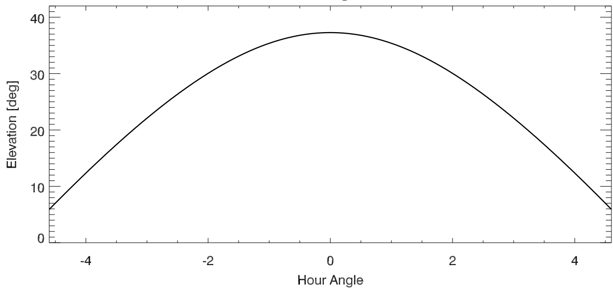
elevation vs hour angle for: NGC6357
