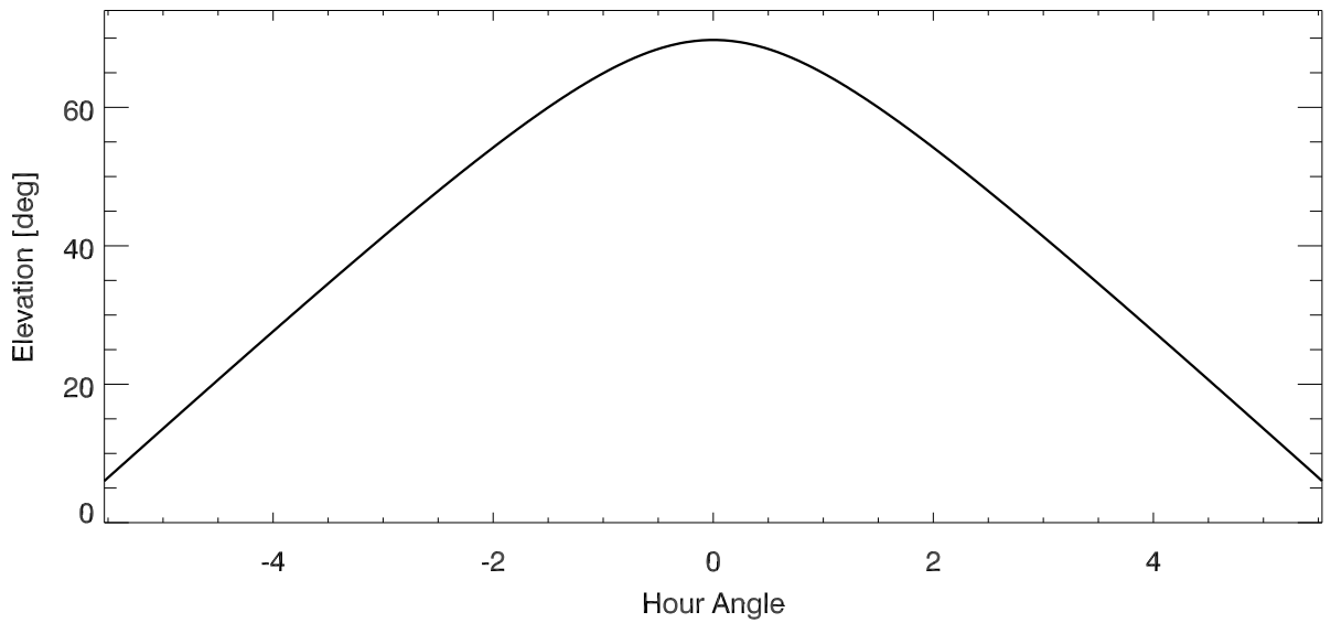
elevation vs hour angle for: M42B
