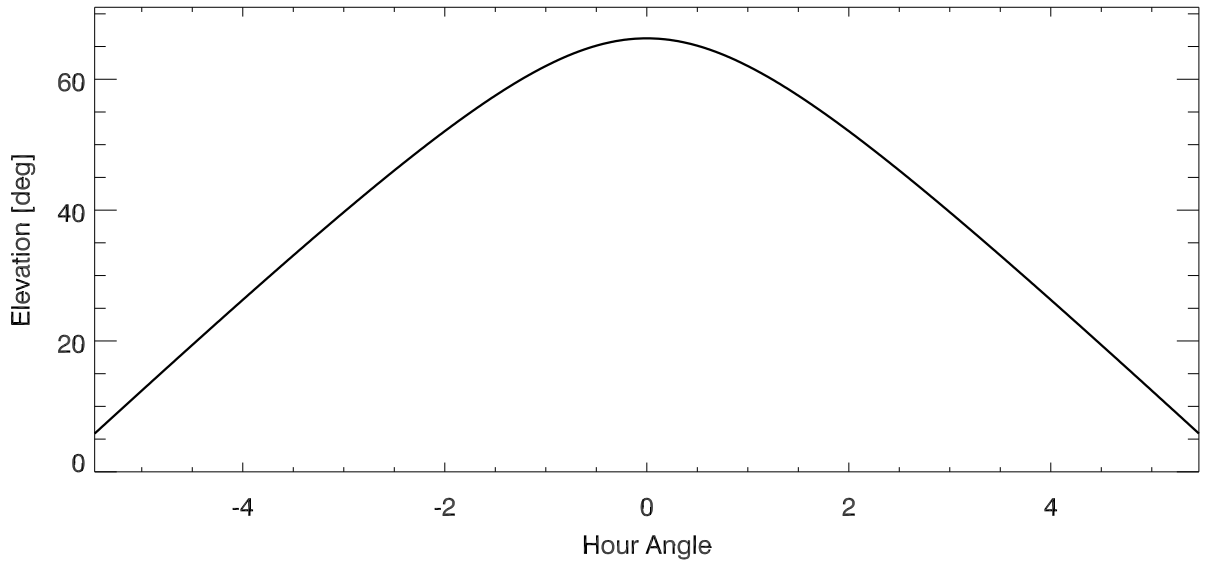
elevation vs hour angle for: M42A
