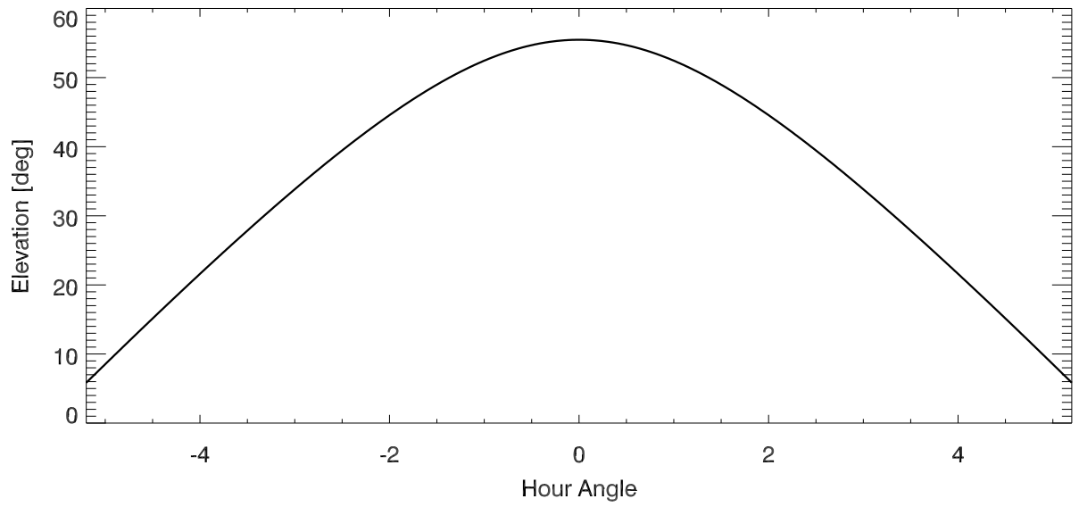
elevation vs hour angle for: M17
