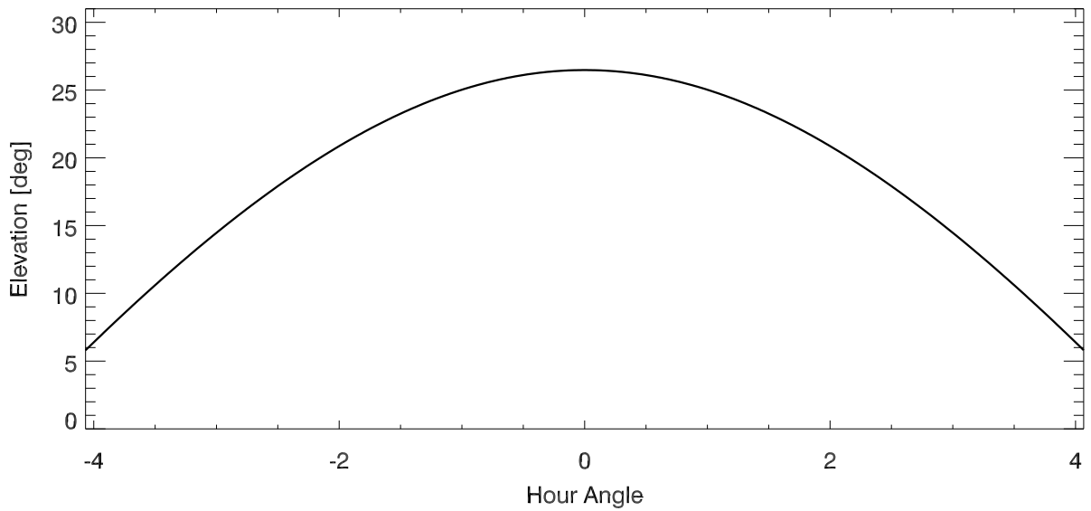
elevation vs hour angle for: B0833-45
