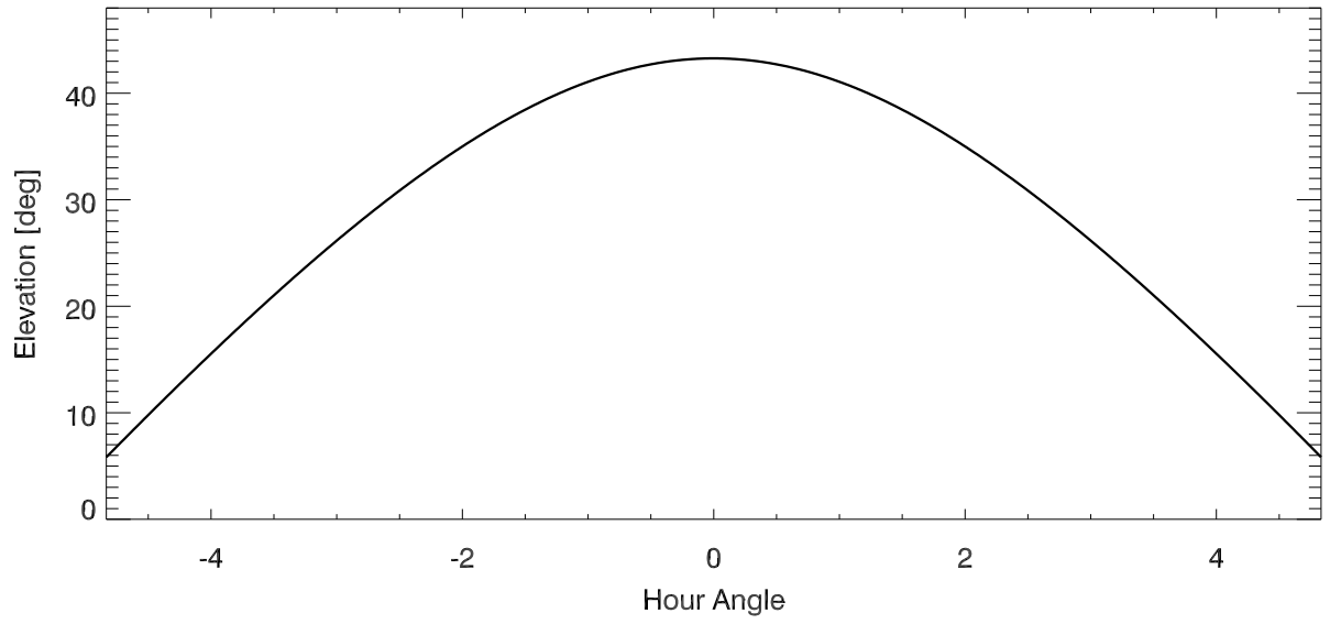
elevation vs hour angle for: SgrB2
