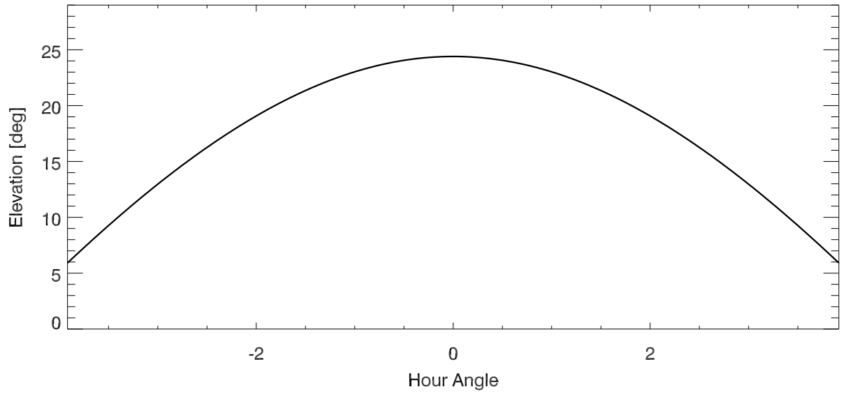
elevation vs hour angle for: J0437-4715
