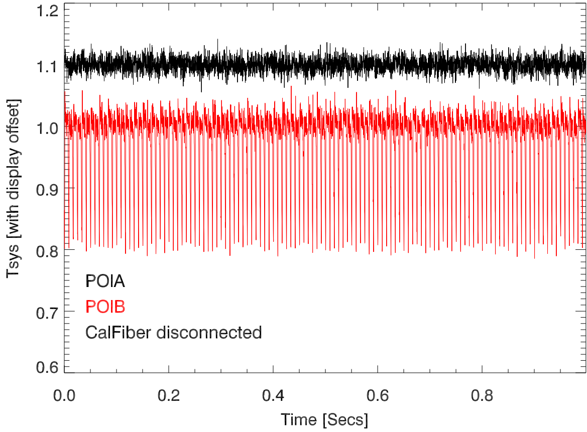
221104 psr B0329+54 totPwr vs time rec 1
