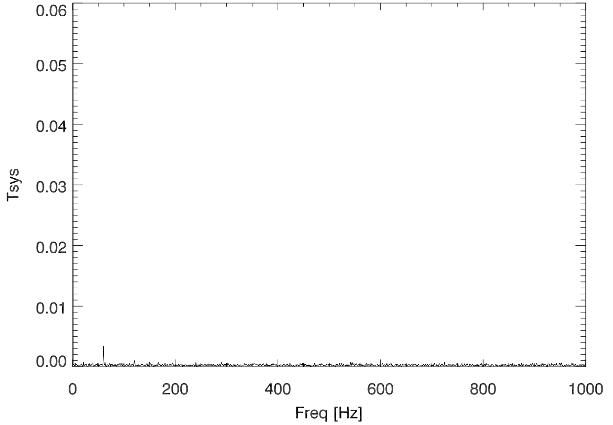
221104 psr B0329+54 spectralMag of TotalPwr. PoIA
