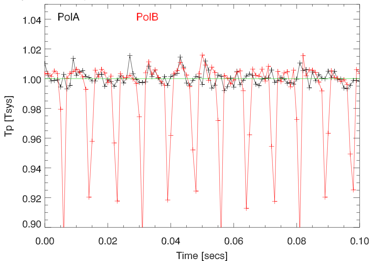
221110 Tp vs Time. (File 500: calFibBufAcOn, cal cables normal, switch bias cab
