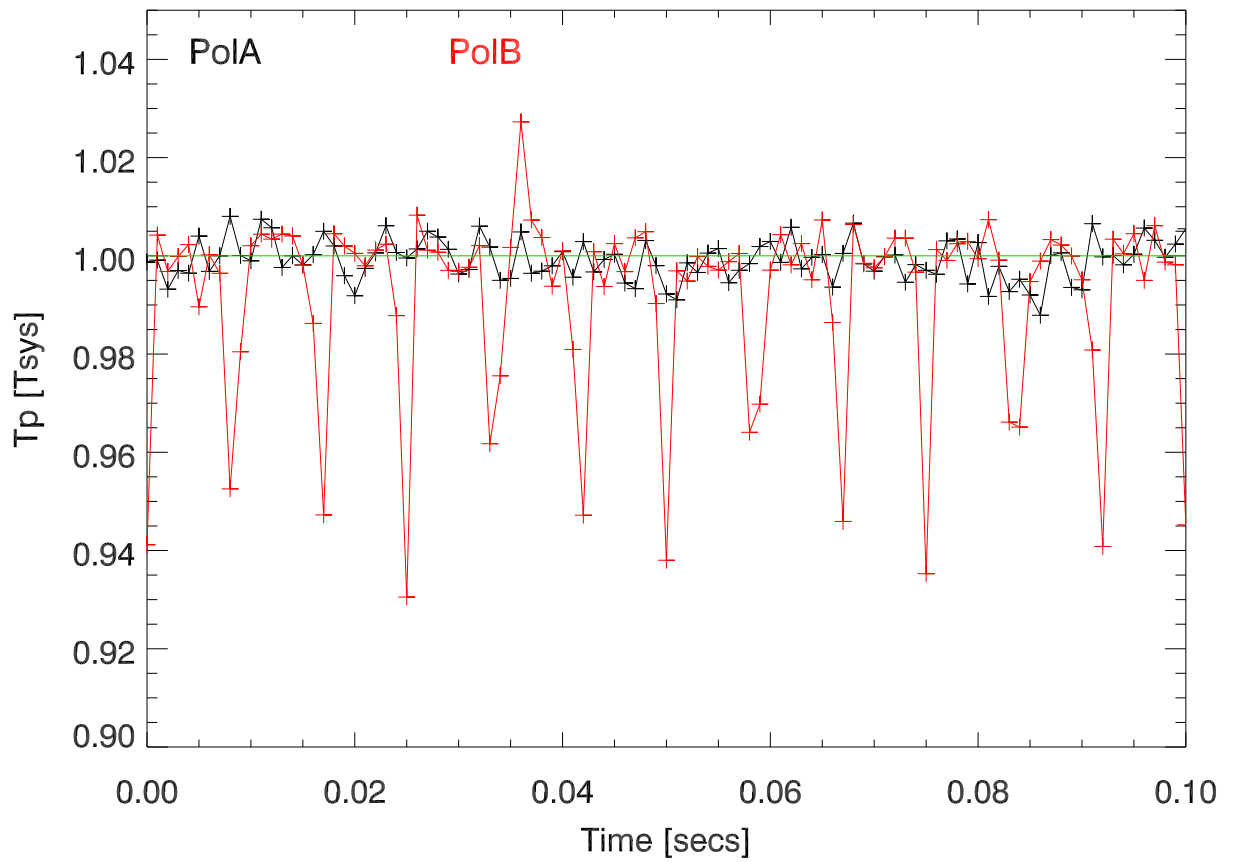
221110 Tp vs Time. (File 200: calFibBufAcOff, reverse cal cables at couplers)
