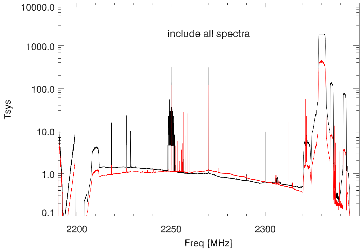
Peak hold spectra for az swing 1
