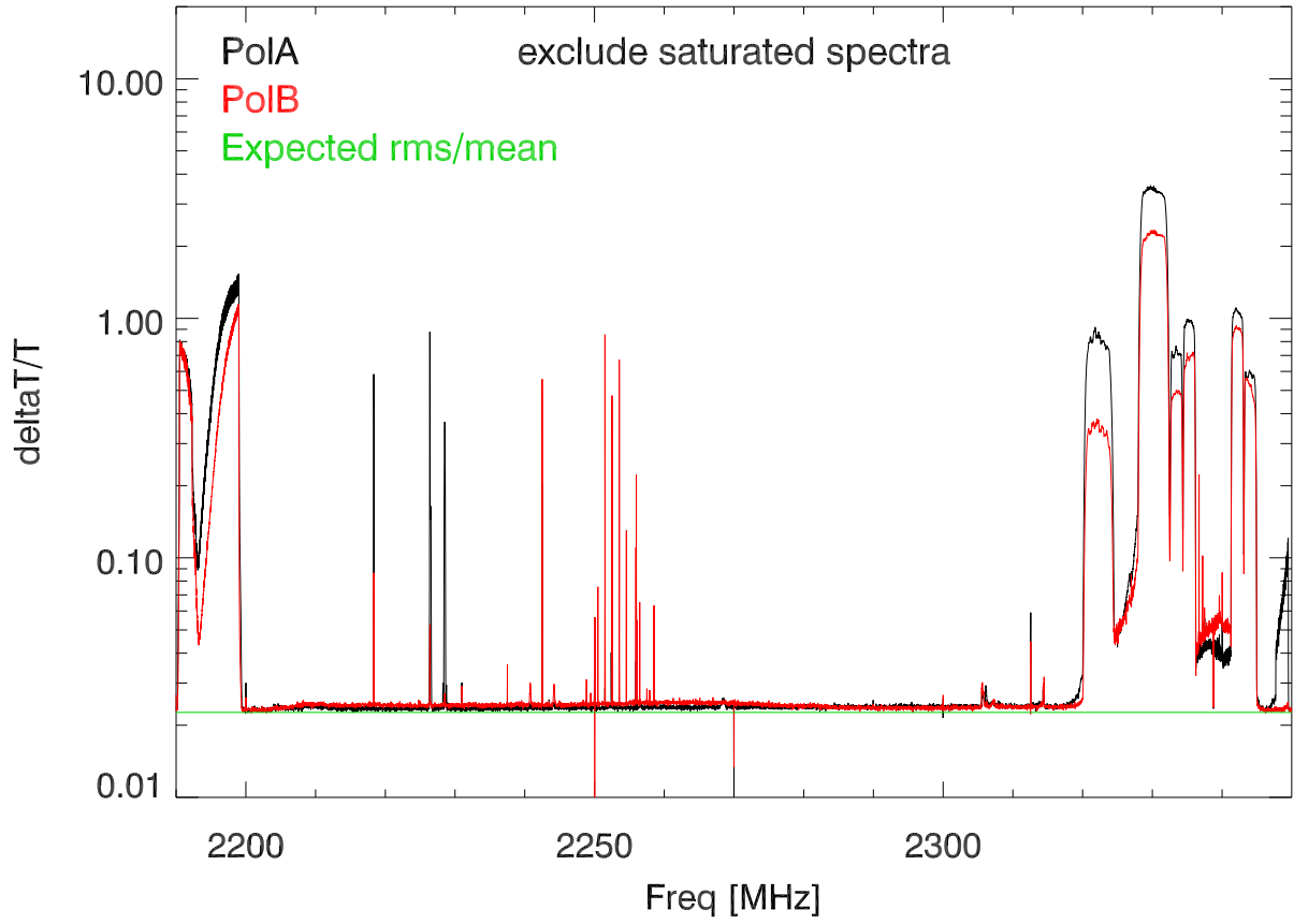
22mar22 azswing 1: rms/mean by freqchan for 360 deg swing
