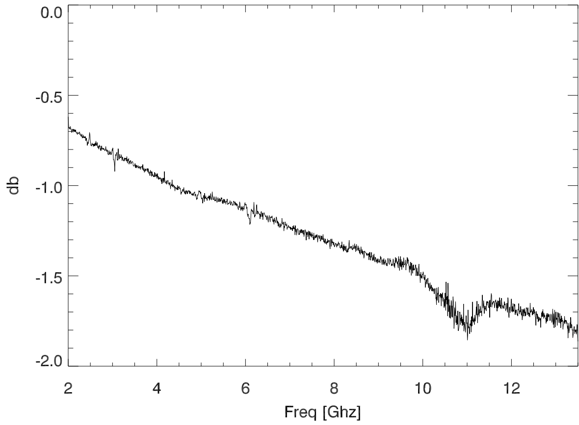
15may23: cable loss dewar to filterbank box
