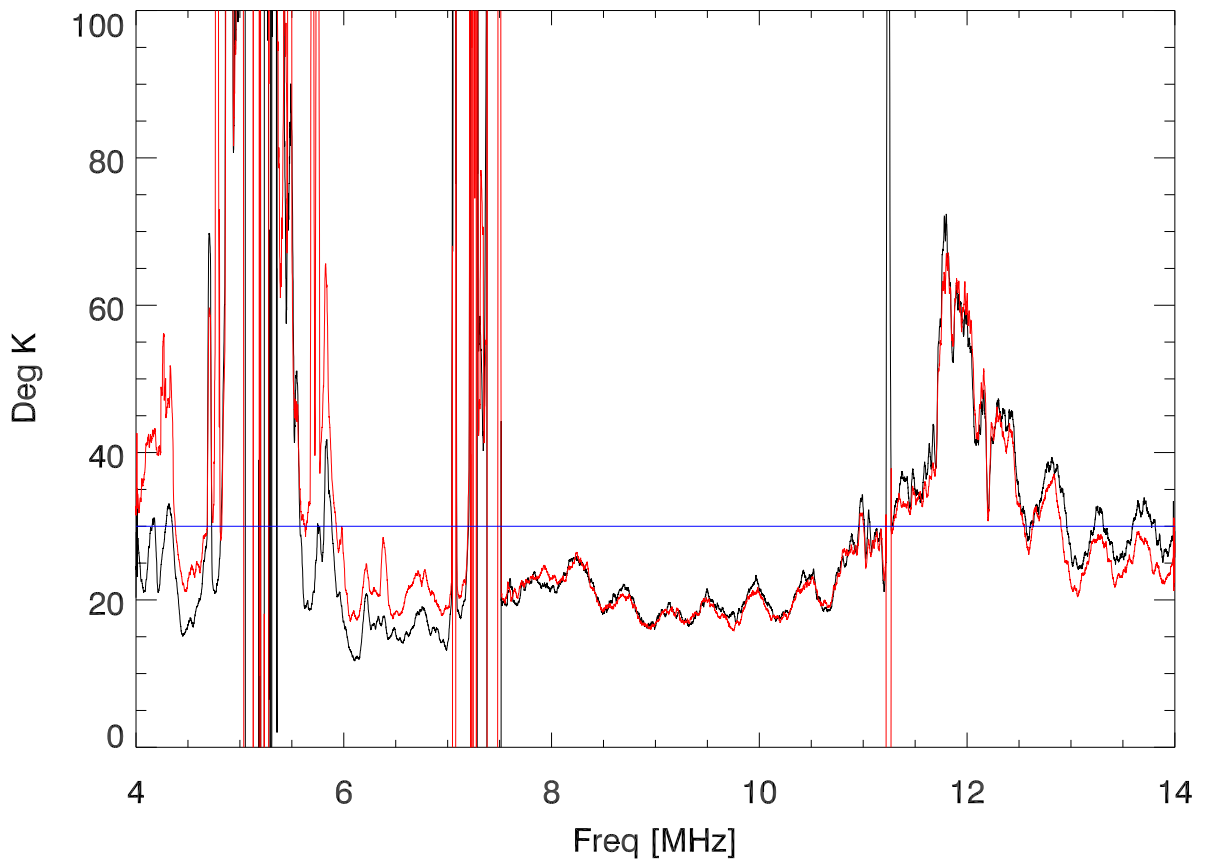
Compare Tflange postamp on, before after cable change
