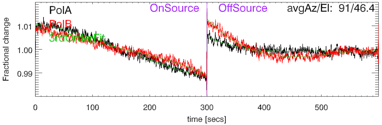
220803 3C274 Fractional change cal Deflection vs time. BandCfr:8931.0 Pat:2
