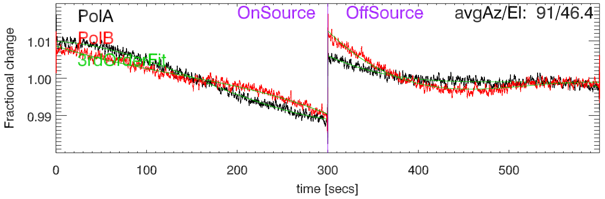
220803 3C274 Fractional change cal Deflection vs time. BandCfr:8505.0 Pat:2
