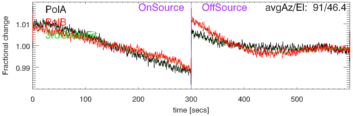
220803 3C274 Fractional change cal Deflection vs time. BandCfr:8789.0 Pat:2
