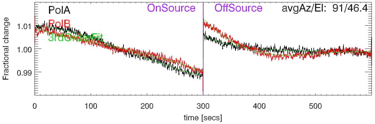
220803 3C274 Fractional change cal Deflection vs time. BandCfr:8219.0 Pat:2
