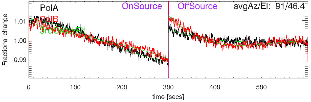
220803 3C274 Fractional change cal Deflection vs time. BandCfr:9073.0 Pat:2
