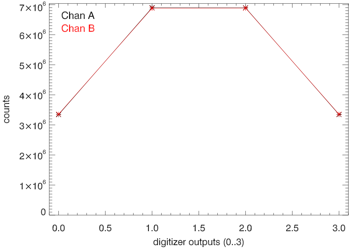
histogram of 2bit raw a/d outputs. t004aa
