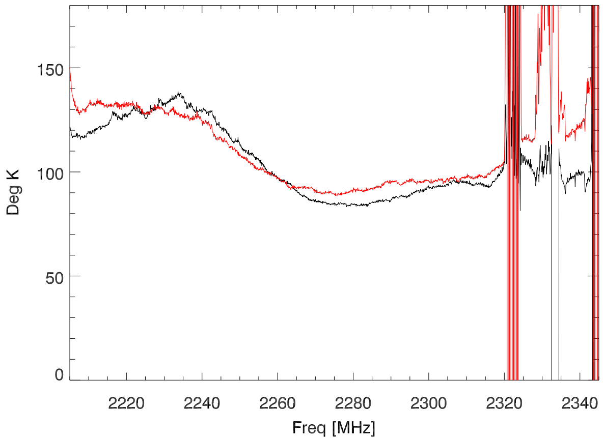
220624 Measured Sband Tsys vs freq (using calOffs)
