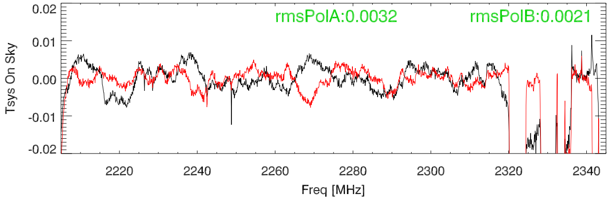
Fit residuals: (measured - fit) vs freq. On Sky
