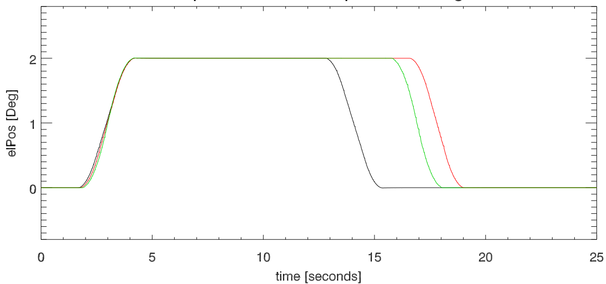
EI position vs Tm. EIStepSize=2.00 Deg
