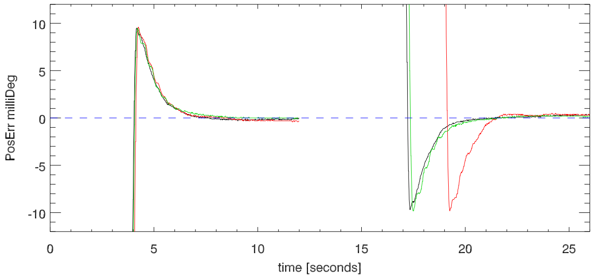
Az step settling Error vs Tm. AzStepSize=2.00 Deg
