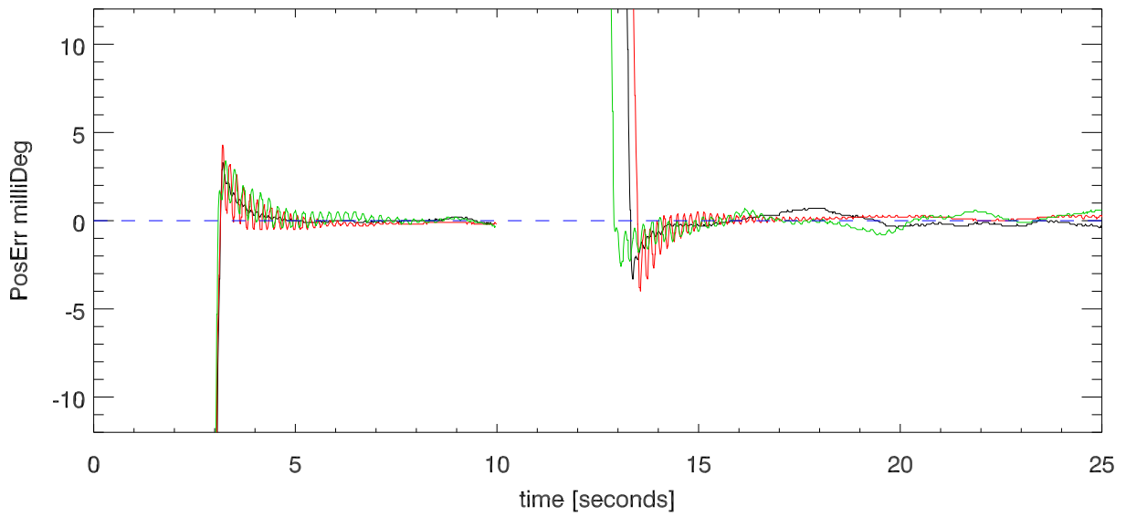
EI step settling Error vs Tm. EIStepSize=0.10 Deg
