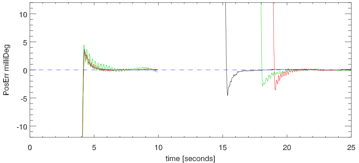
EI step settling Error vs Tm. EIStepSize=2.00 Deg
