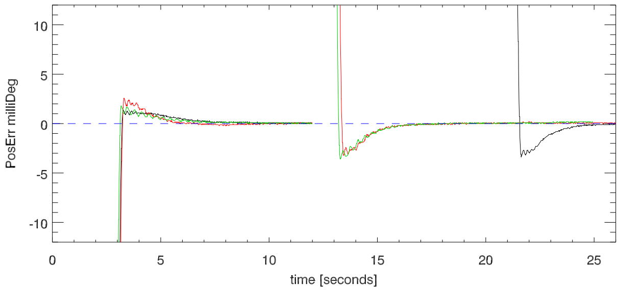
Az step settling Error vs Tm. AzStepSize=0.10 Deg
