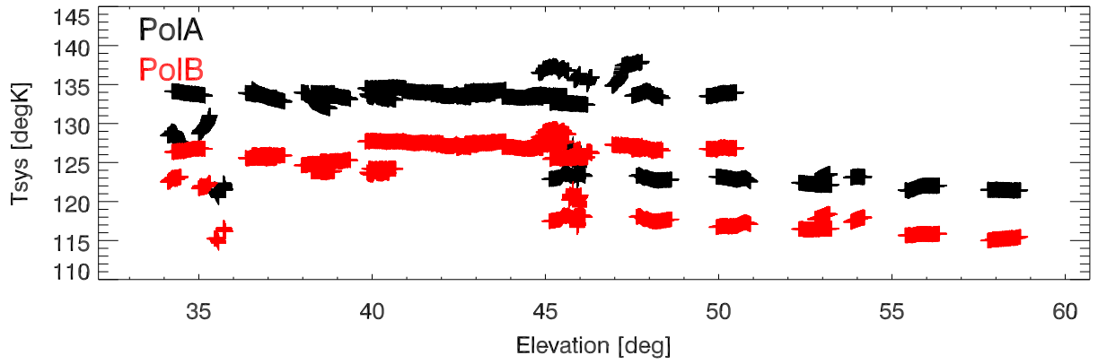
220209 Tsys vs elevation (using 1sec offSrc samples). freqBand:9168
