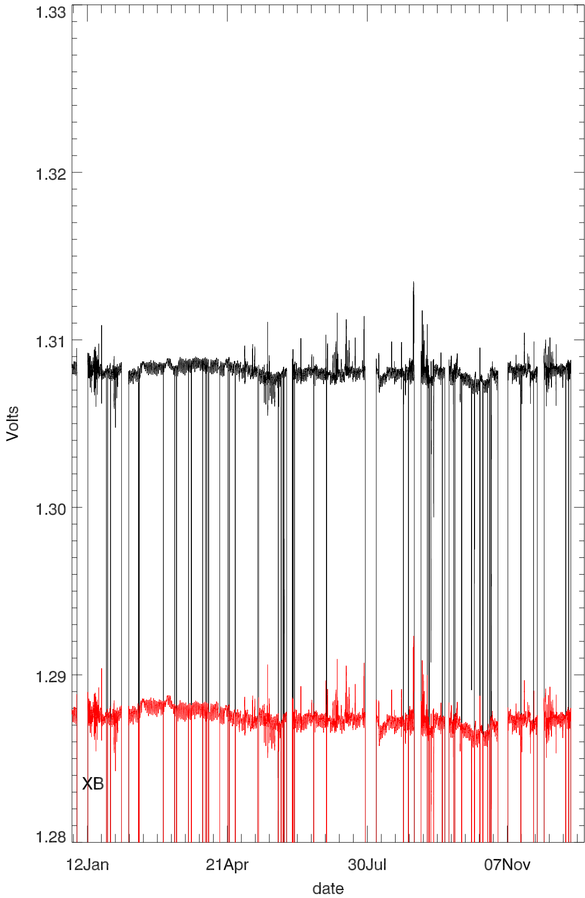
Dewar voltage stage 1 (year 2016)
