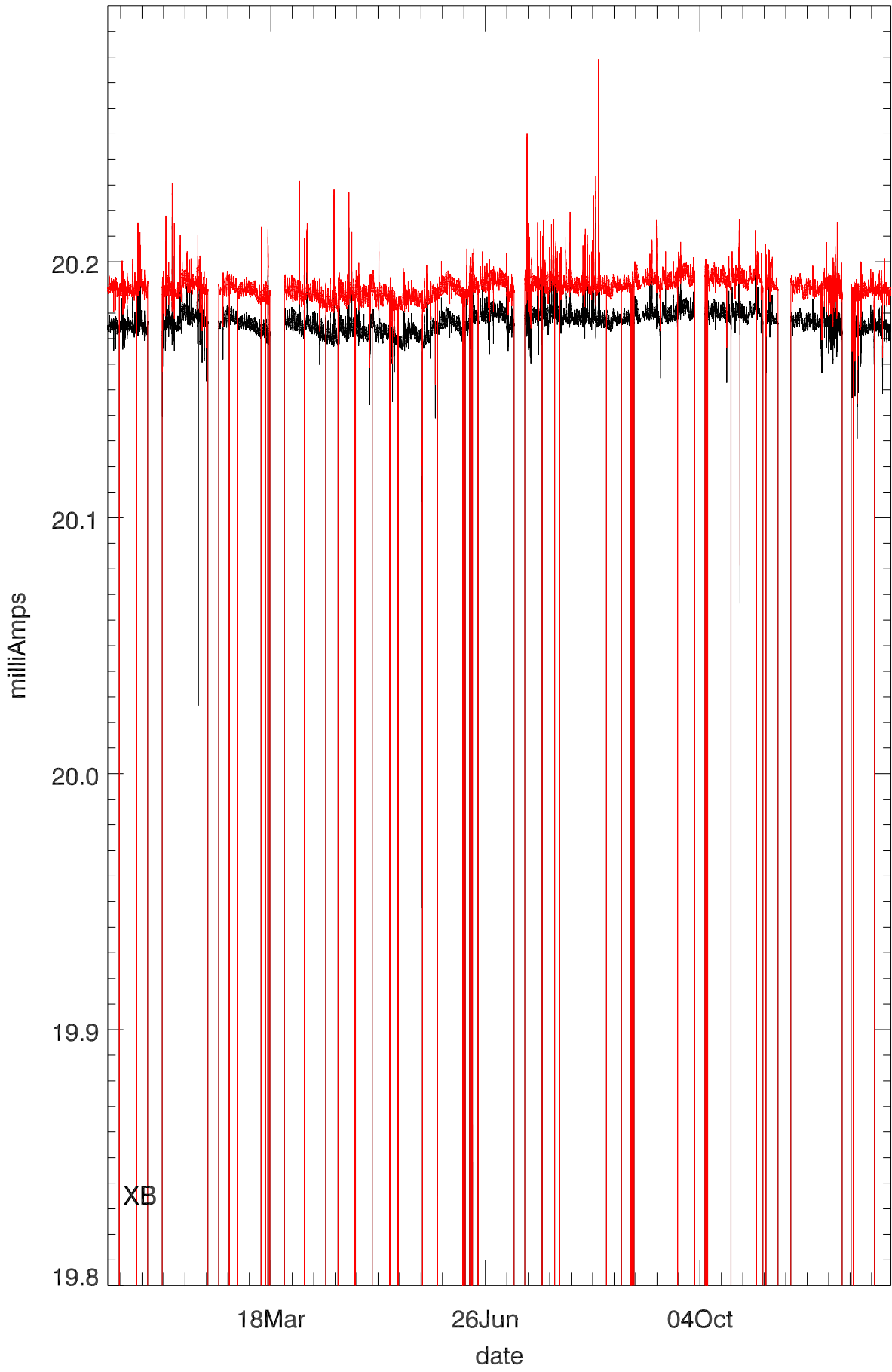
Dewar Current stage 1 (year 2015)
