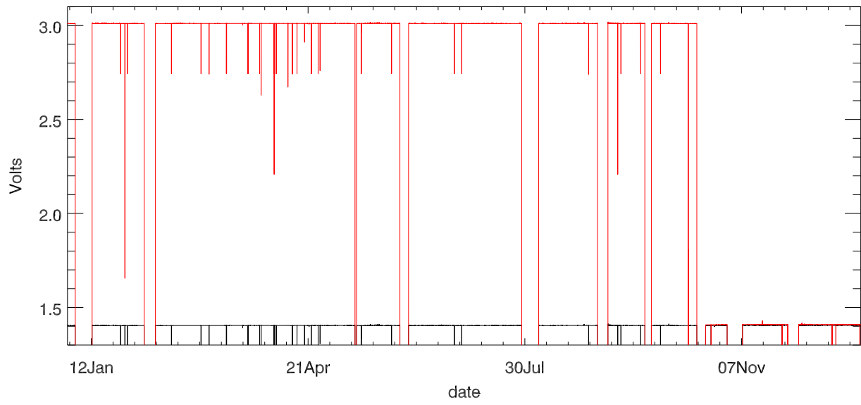
Dewar voltage stage 2 (year 2016)
