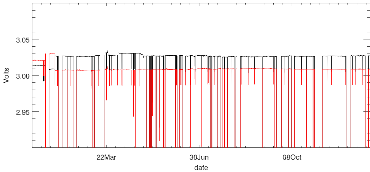
Dewar voltage stage 2 (year 2018)
