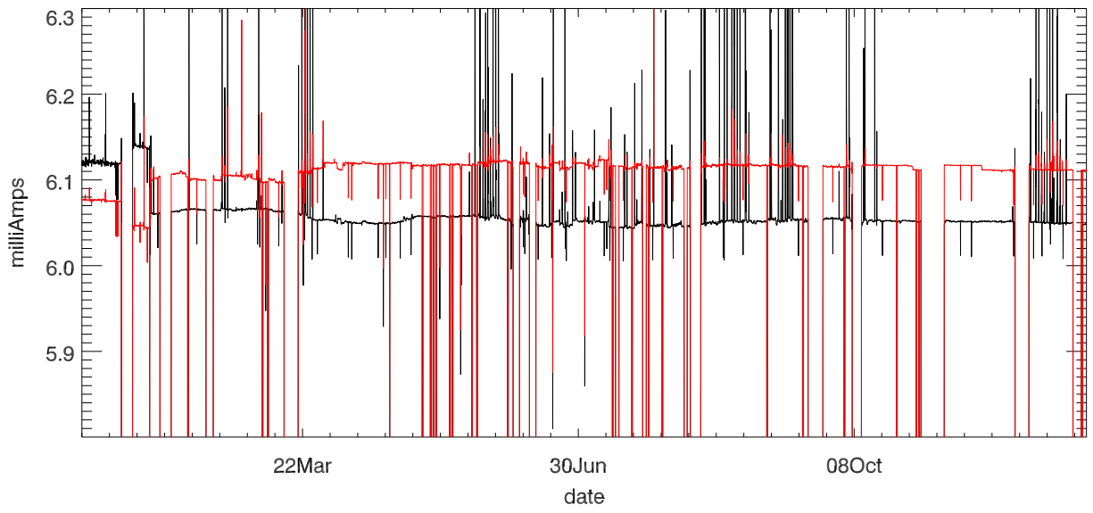
Dewar Current stage 2 (year 2018)
