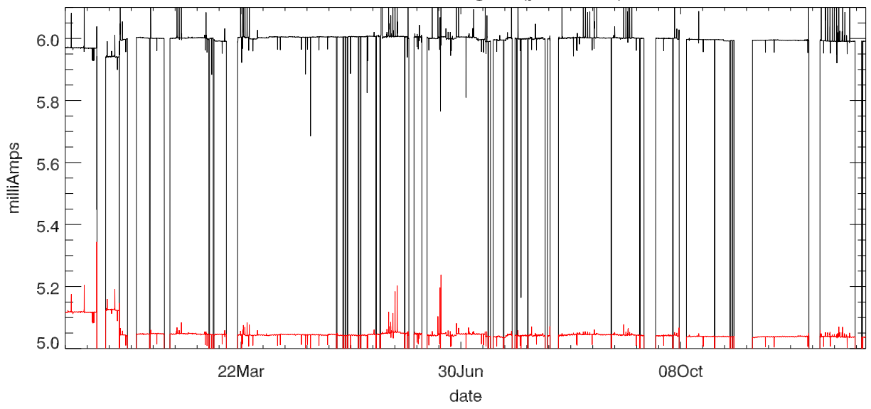
Dewar Current stage 3 (year 2018)
