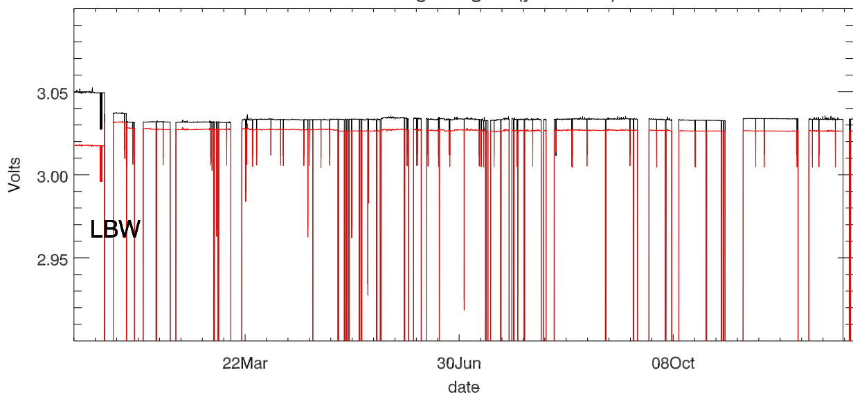
Dewar voltage stage 3 (year 2018)
