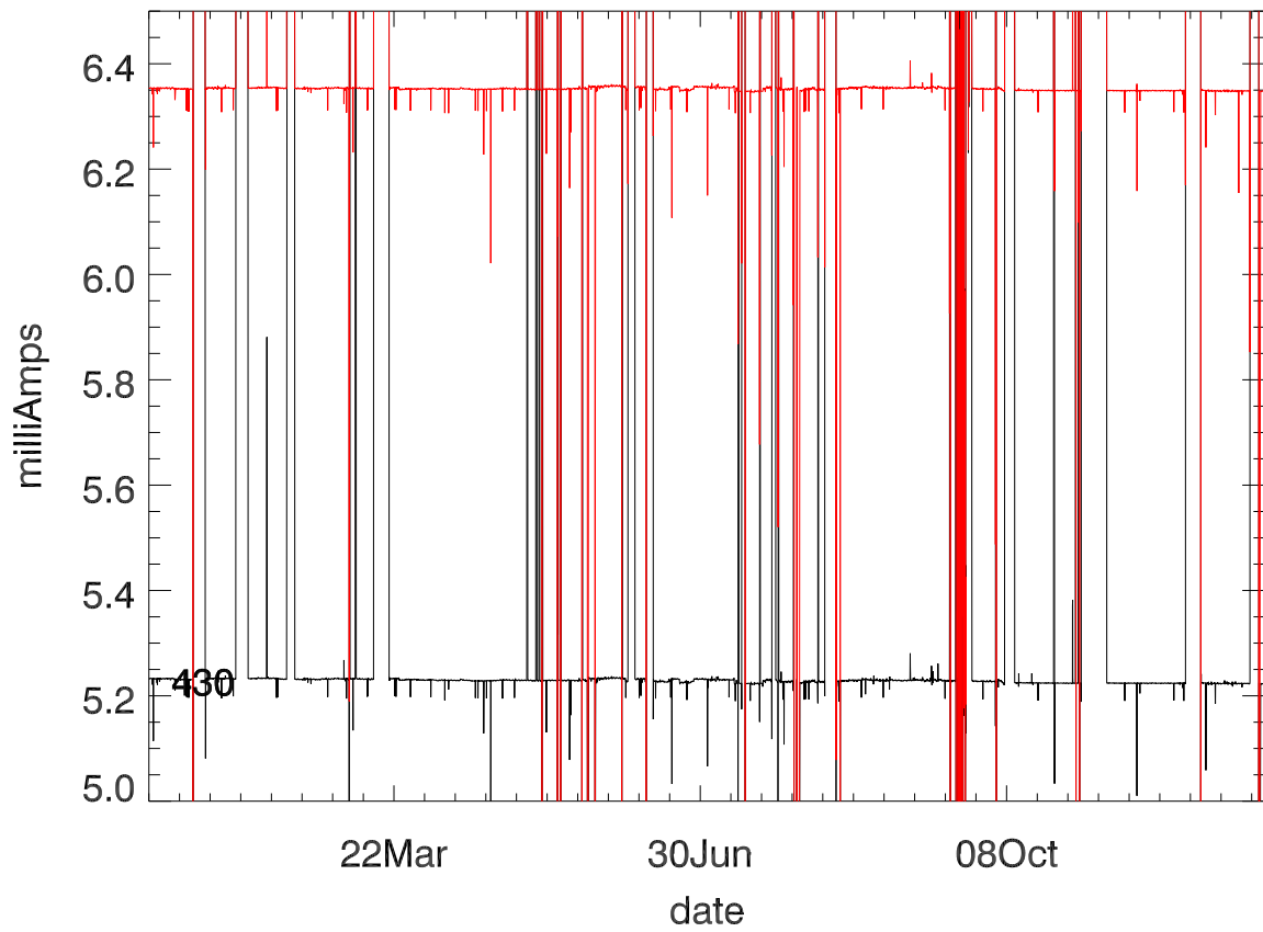
Dewar Current stage 2 (year 2018)
