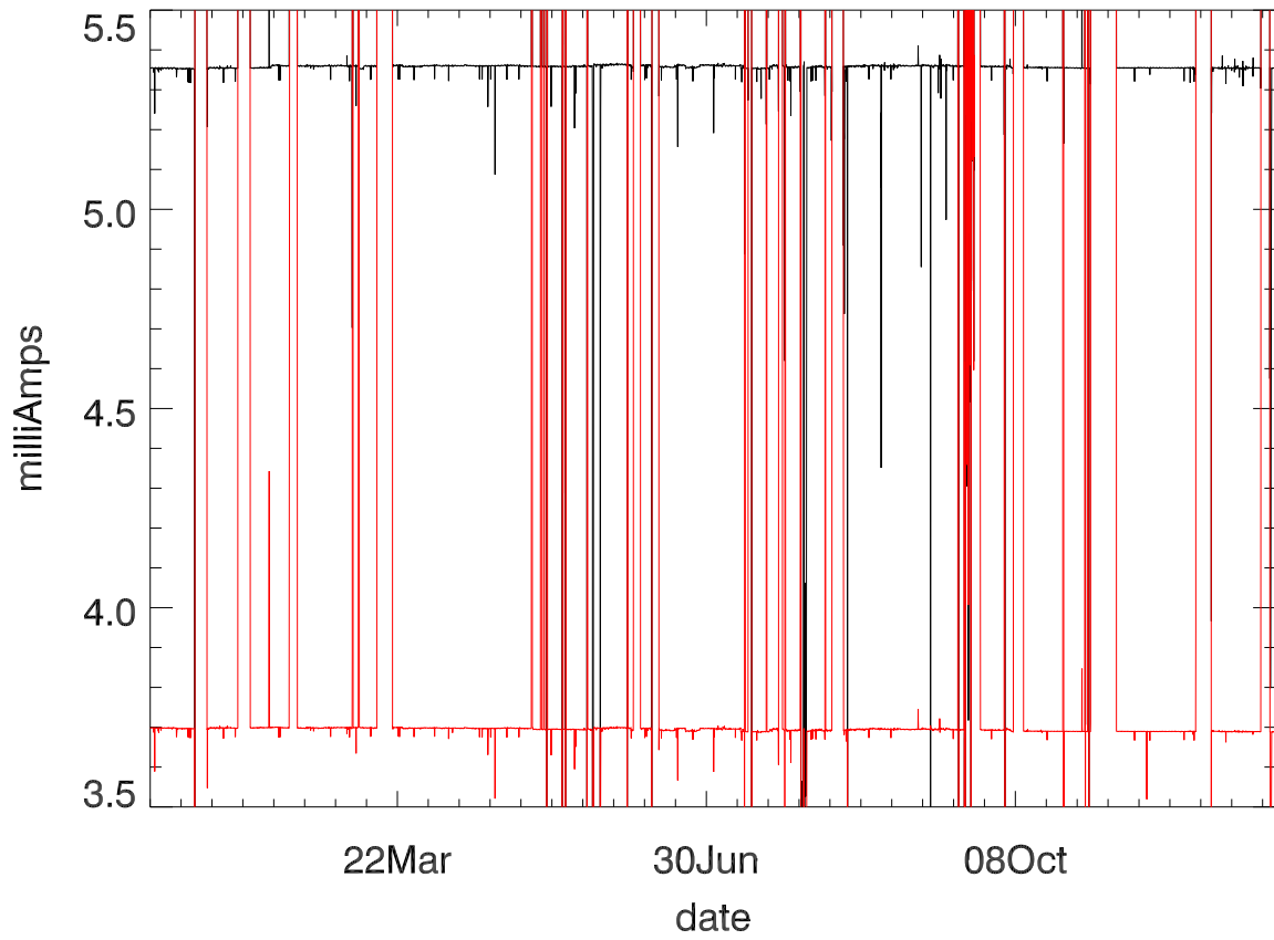
Dewar Current stage 1 (year 2018)
