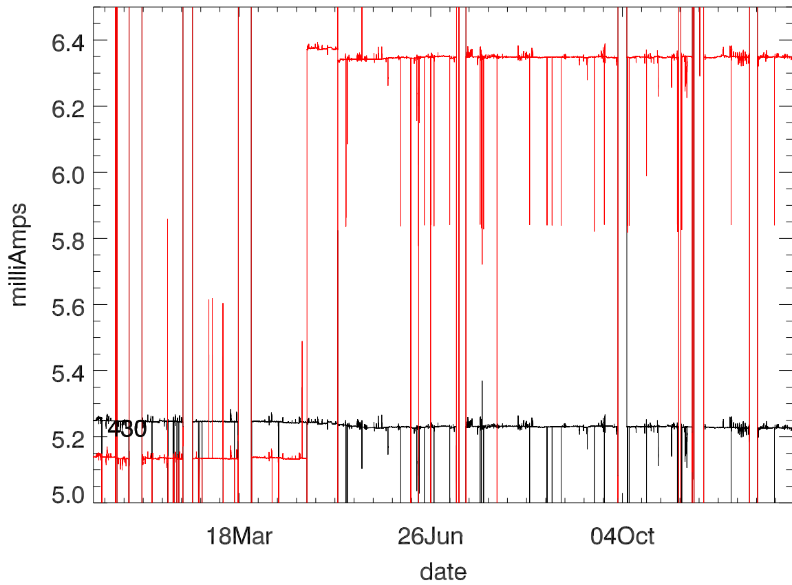
Dewar Current stage 2 (year 2015)
