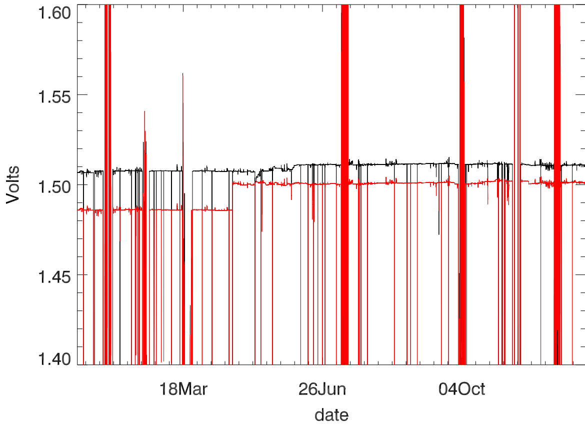
Dewar voltage stage 1 (year 2015)
