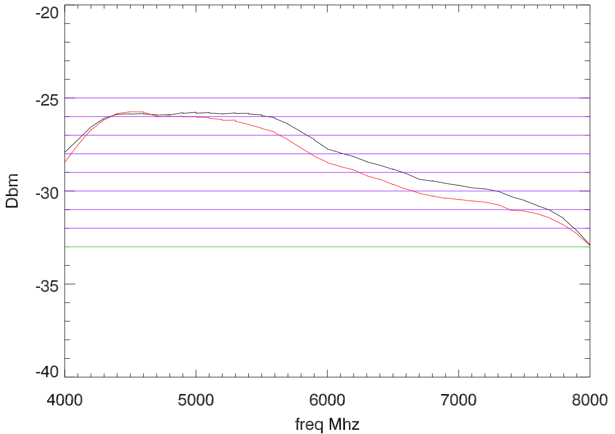
Add 9db gain to polA, 5db gain to polB. (rf attn=0db)
