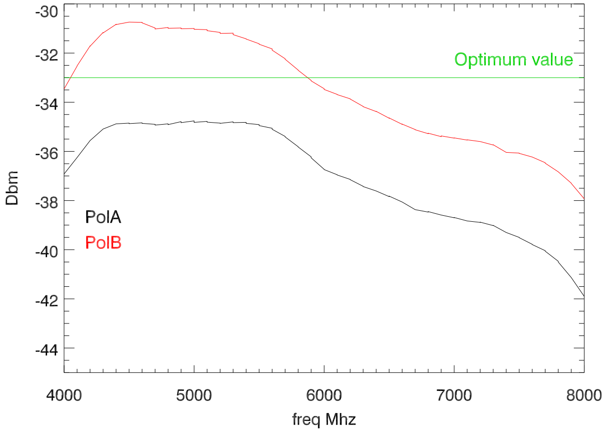
10aug17 cbw if1 power meter value vs freq. rf attn=0db
