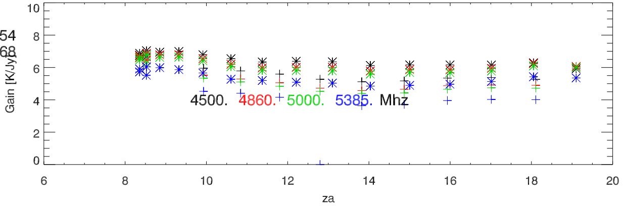
29aug17 cbw after horn move, turpos=162 Deg Gain K/Jy
