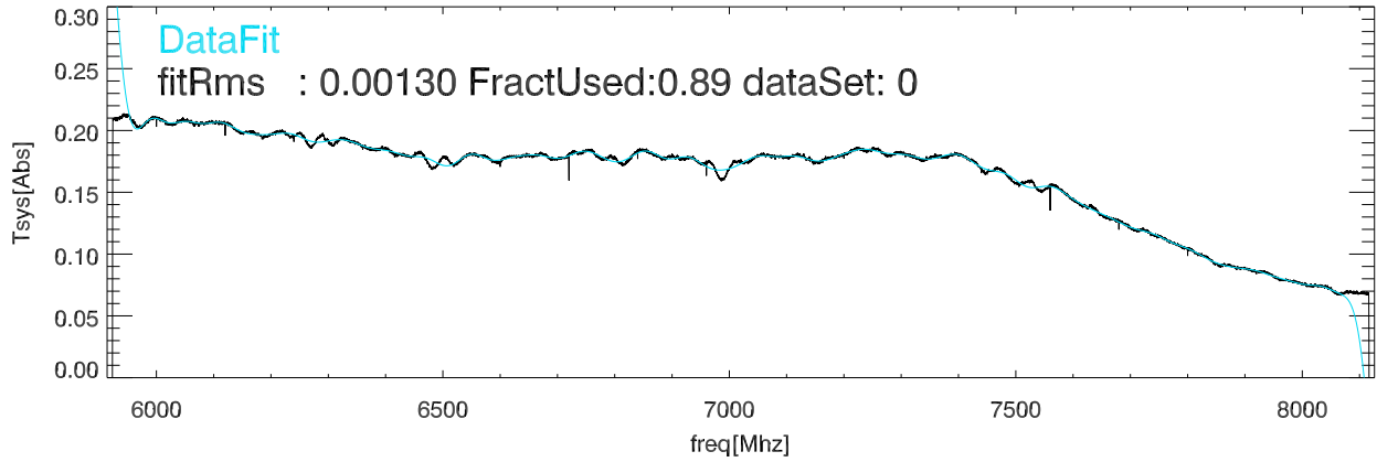
28jun12 cbhi: Averaged data and fit for CalDeFlection/Tsys on abs polB
