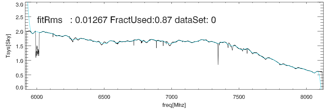
28jun12 cbhi: Averaged data and fit for CalDeFlection/Tsys on Sky polA
