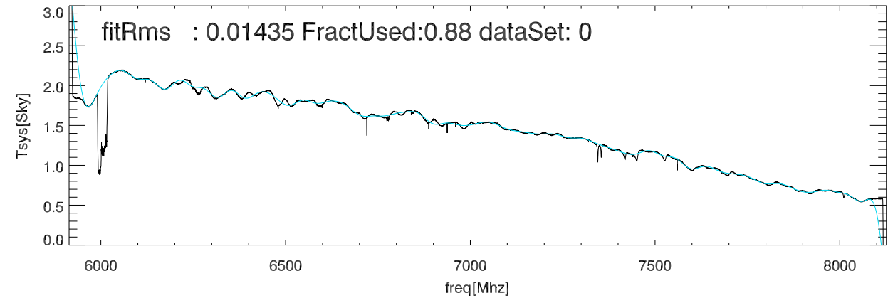
28jun12 cbhi: Averaged data and fit for CalDeFlection/Tsys on Sky polB
