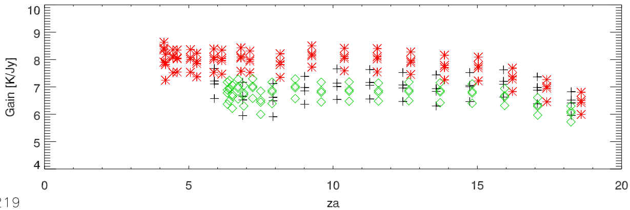
11feb13 cband after reinstall in dome Gain K/Jy
