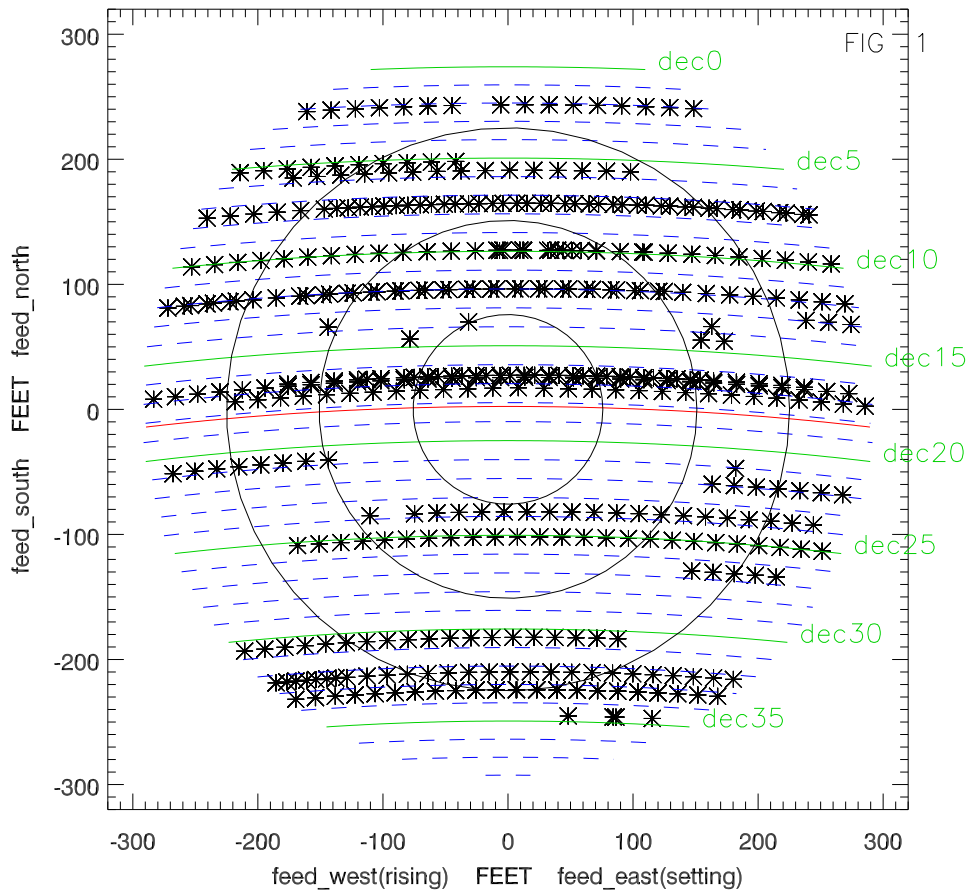
az za coverage nov17-mar18 sbn calibration runs
