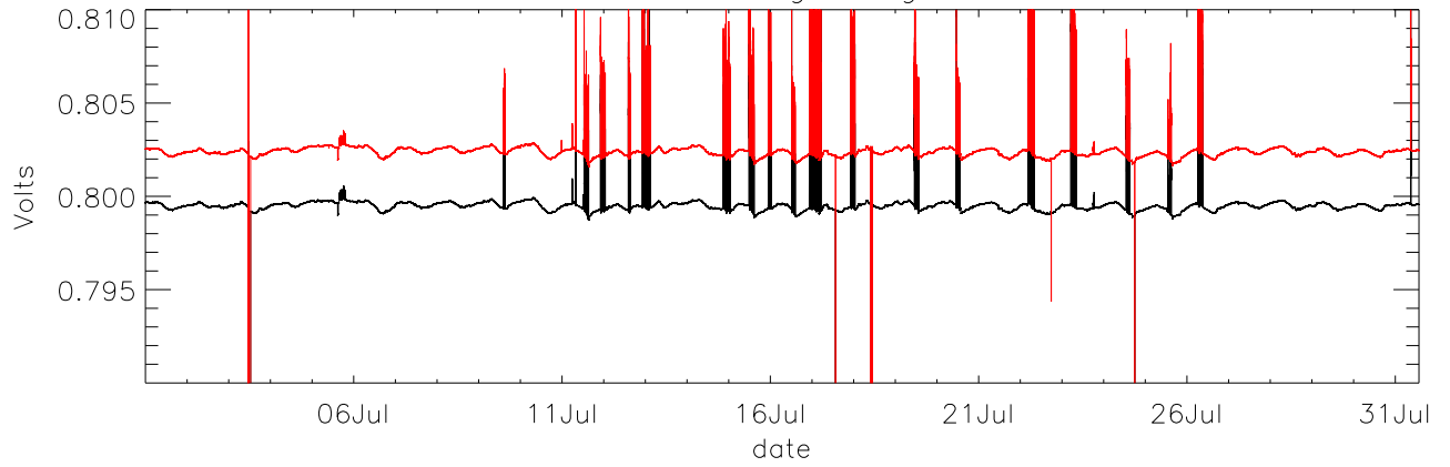
Dewar current stage 1
