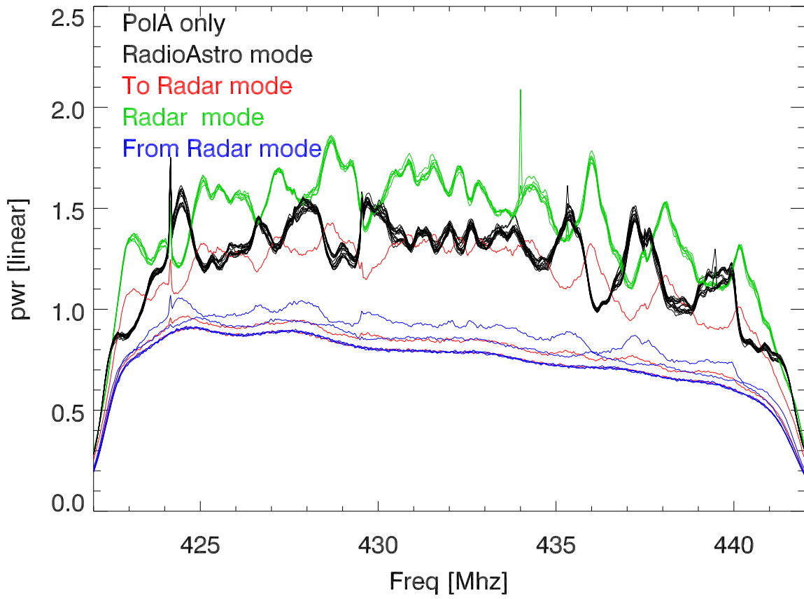
spectra while switch turned astro->radar->astro
