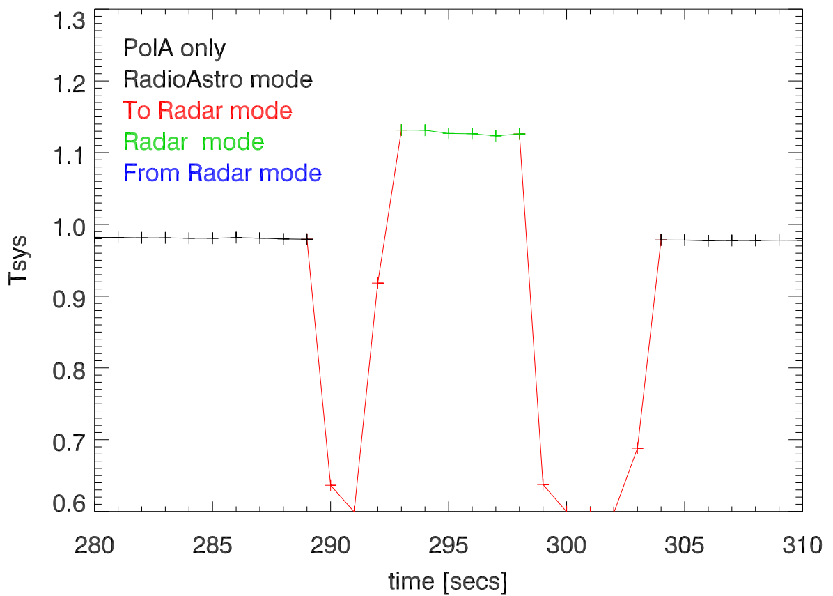
blowup when radar/radioastronomy switch moved
