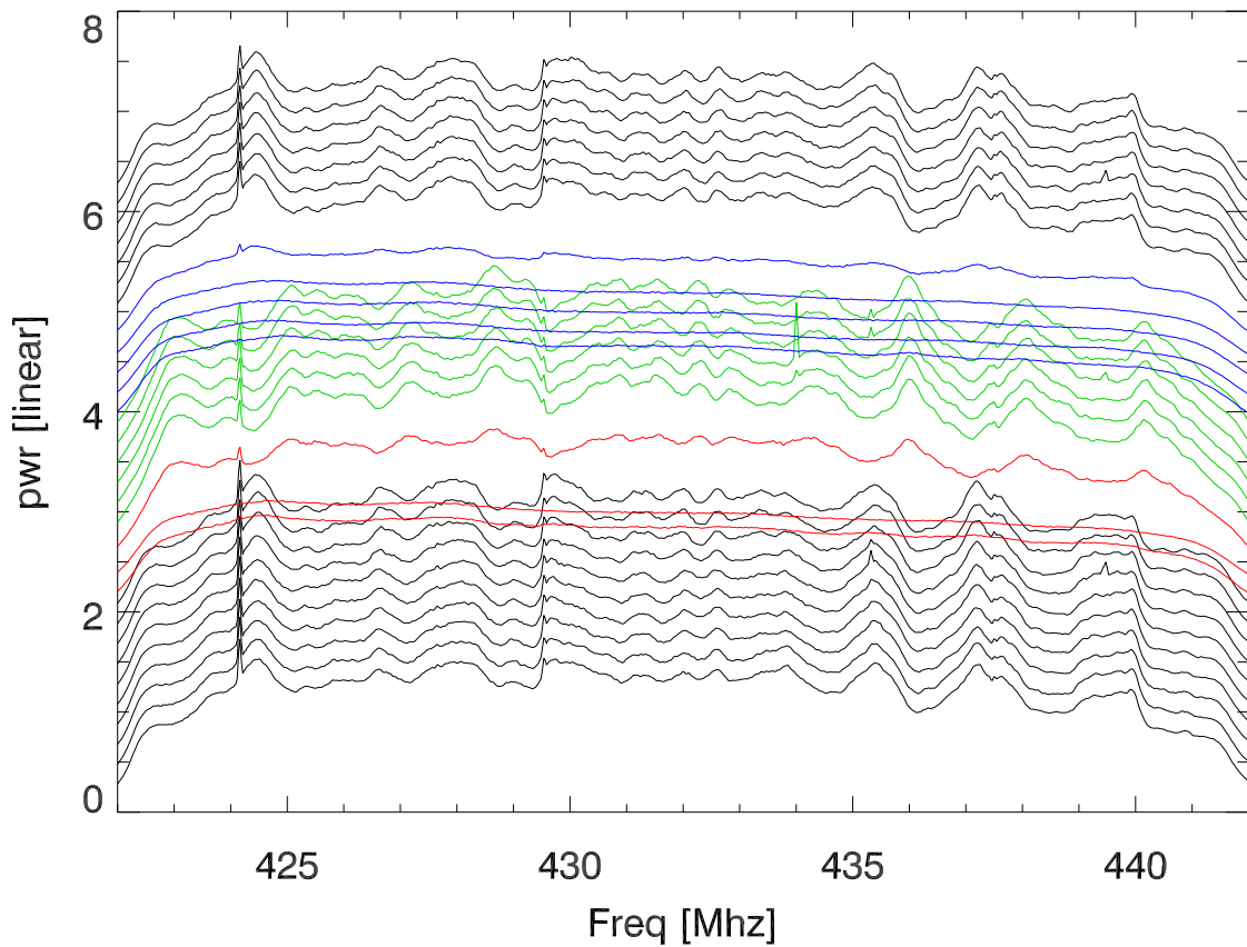
spectra with offsets for display
