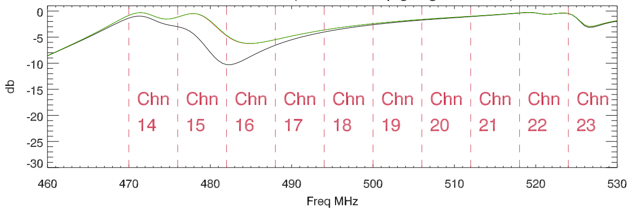
02dec12 430Gr PoIA filter. (S11 = c clamp going to turnstile). S11
