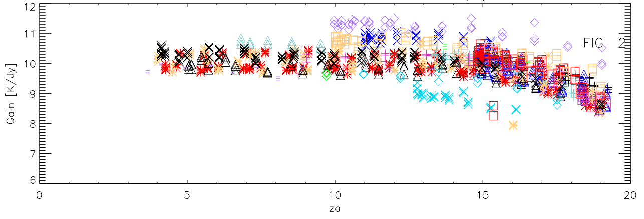
327 calibration runs Mar03–Feb05 Gain K/Jy
