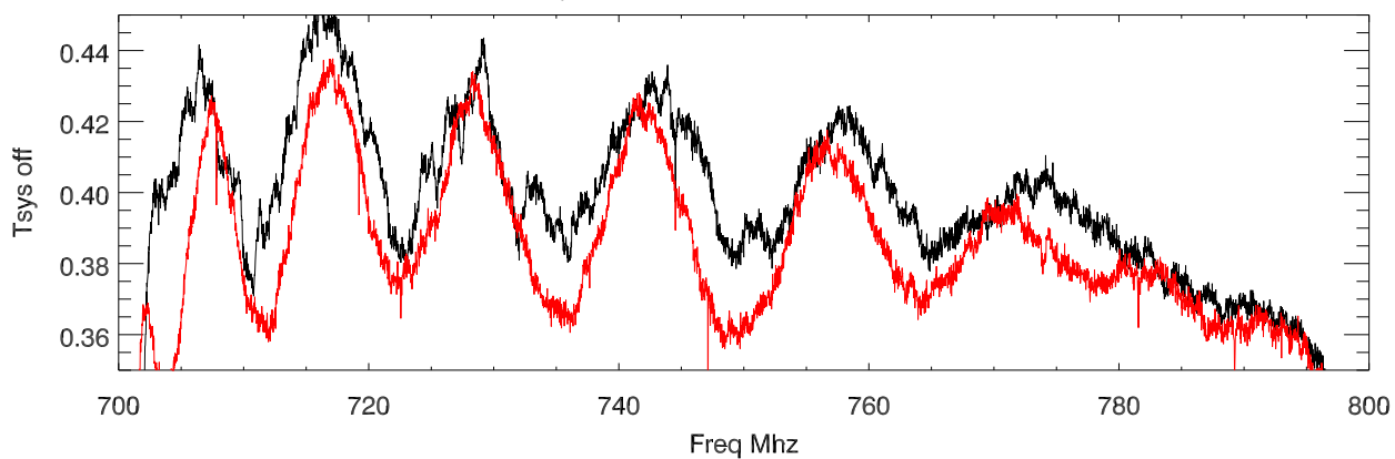
CalibOn/CalibOff -1 for:J001018+1433BP
