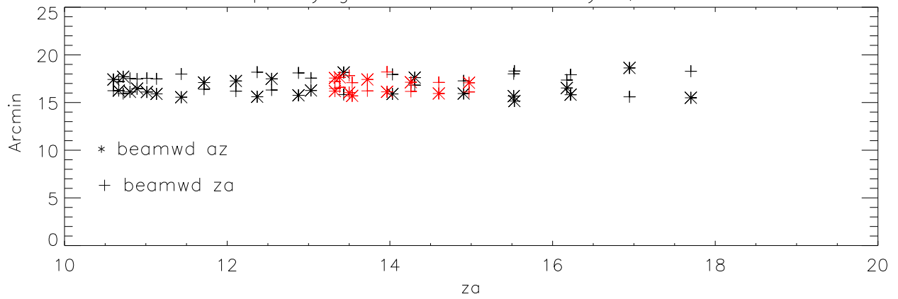
compare ch beam widths: 29may06, 12feb06
