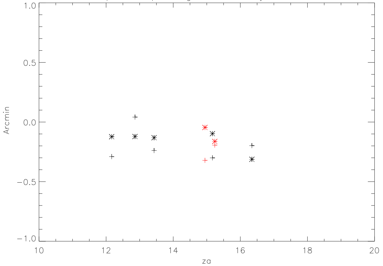
compare ch pointing error: 29may06, 12feb06
